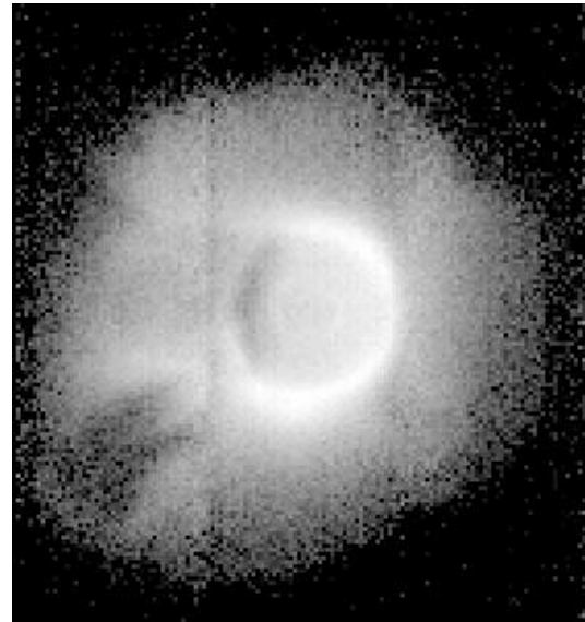
IMAGE EUV image of Earth's plasmasphere taken at 1712 UT on 24 June 2000. To the lower left is a prominent low-density region or “void.”
