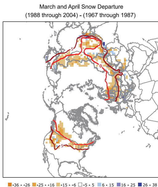
Figure TS.12. (Top) Northern Hemisphere March–April snow-covered area from a station-derived snow cover index (prior to 1972) and from satellite data (during and after 1972). The smooth curve shows decadal variations (see Appendix 3.A) with the 5 to 95% data range shaded in yellow. (Bottom) Differences in the distribution of March–April snow cover between earlier (1967–1987) and later (1988–2004) portions of the satellite era (expressed in percent coverage). Tan colours show areas where snow cover has declined. Red curves show the 0°C and 5°C isotherms averaged for March–April 1967 to 2004, from the Climatic Research Unit (CRU) gridded land surface temperature version 2 (CRUTEM2v) data. The greatest decline generally tracks the 0°C and 5°C isotherms, reflecting the strong feedback between snow and temperature. {Figures 4.2, 4.3}
