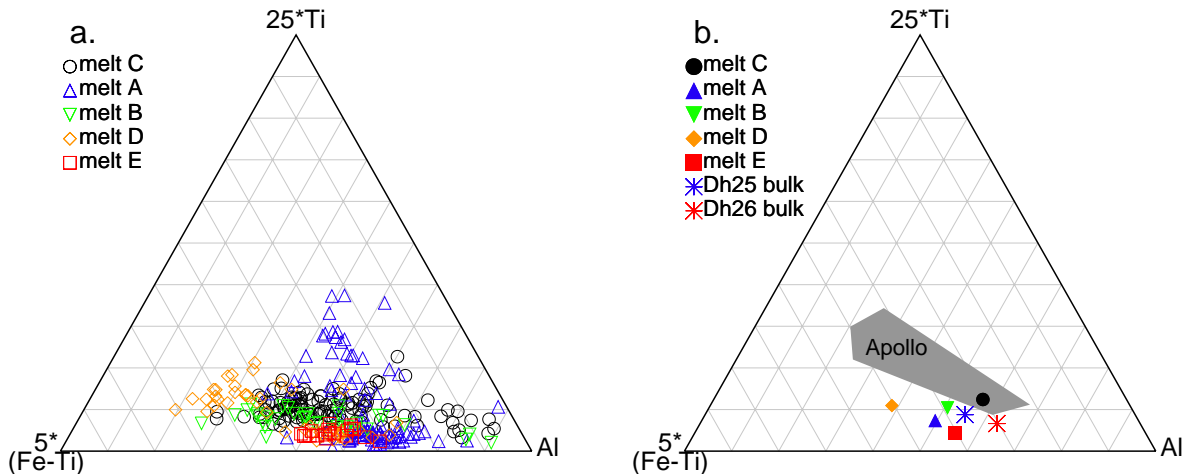
Figure 2: a) all analyses of impact melt clasts; b) clast averages, with bulk meteorites and Apollo impact melts.
