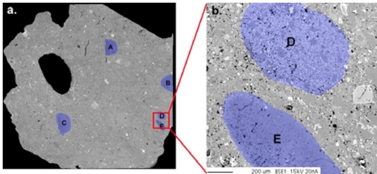
Figure 1: a) BSE mosaic of Dhofar 025 thin section (f.o.v. ~ 2 cm), with analyzed melt clasts in blue; b) enlarged area showing textural characteristics and scale of heterogeneity within clasts D and E (scale bar = 200 \mu\text{m} ).
