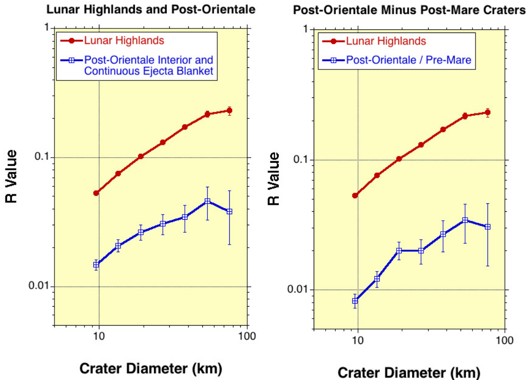
Fig. 5 R plots of the post-Oriente craters (left) and the post-Oriente minus post-mare craters (right). The lunar highlands R plot is shown in red for comparison.
