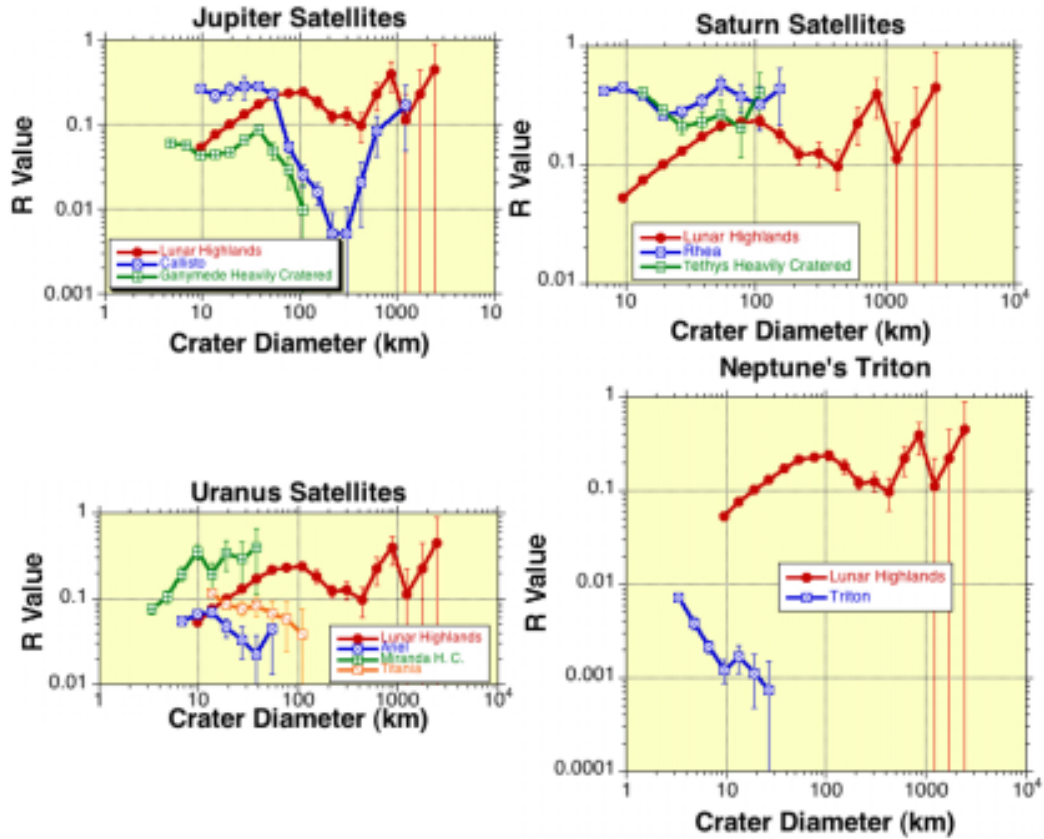
Fig. 13 The impact crater SFDs on the heavily cratered surface units of the outer planet satellites. In each panel, for reference we also show the R plot for the lunar highlands craters.
