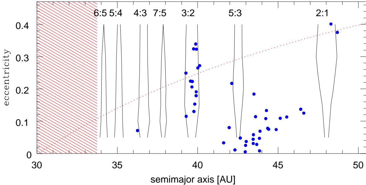
Fig. 2. The locations and widths in the (a, e) plane of Neptune's low order mean motion resonances in the Kuiper Belt. Orbits above the dotted line are Neptune-crossing; the hatched zone on the left indicates the chaotic zone of first order resonance overlap. The dots indicate the orbits of KBOs with reasonably well determined orbits in January 1999. (Adapted from Malhotra (1996).)
