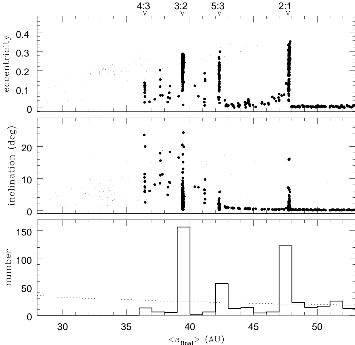
Fig. 5. The distribution of orbital elements of trans-Neptunian test particles after resonance sweeping, as obtained from a 200 Myr numerical simulation in which the Jovian planets’ semimajor axes evolve according to a(t) = a_f - \Delta a \exp(-t/\tau) , with timescale \tau = 4\text{Myr} and \Delta a = \{-0.2, 0.8, 3.0, 7.0\} AU for Jupiter, Saturn, Uranus and Neptune, respectively (Malhotra, 1999). The test particles were initially distributed smoothly in circular, zero-inclination orbits between 28 AU and 63 AU, as indicated by the dotted line in the lower panel. In the upper two panels, the filled circles represent particles that remain on stable orbits at the end of the simulation, while the open circles represent the elements of those particles which had a close encounter with a planet and subsequently move on scattered chaotic orbits (‘removed’ from the simulation at the instant of encounter). Neptune’s mean motion resonances are indicated at the top of the figure.
