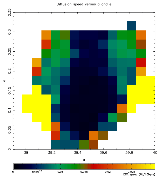
Fig. 4. A map of the dynamical diffusion speed of the semimajor axis of test particles in Neptune's 3:2 mean motion resonance. The test particles in this numerical study had initial inclinations less than 5 degrees. The color scale is indicated on the bottom. (From Morbidelli (1997).)
