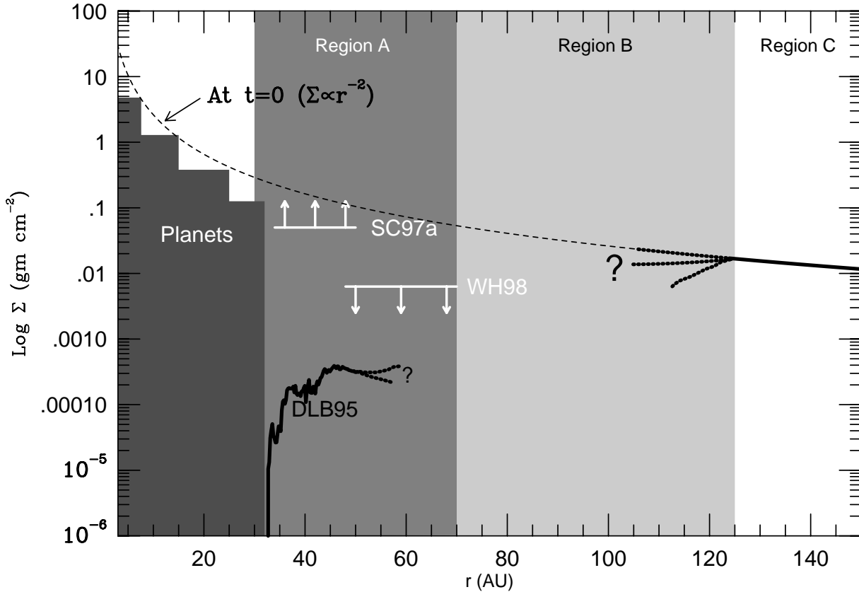
Fig. 8. A strawman model of the Kuiper belt. The dark area at left marked "Planets" shows the distribution of solid material in the outer planets region: it follows a power law with a slope of about -2 in heliocentric distance. The dashed curve is an extension into the Kuiper belt of the power law found for the outer planets and illustrates the likely initial surface density distribution of solid material in the Kuiper belt. The dashed curve has been scaled so that it is twice the surface density of the outer planets, under the assumption that planet formation was 50% efficient. The solid curve shows a model of the mass distribution by Duncan et al. (1995, see Figure 7), scaled to an estimated population of 5 \times 10^9 Kuiper belt objects between 30 and 50 AU. The Kuiper belt is divided into three regions; see text for a description. The dotted curves illustrate the unknown shape of the surface density distribution in Region B.
