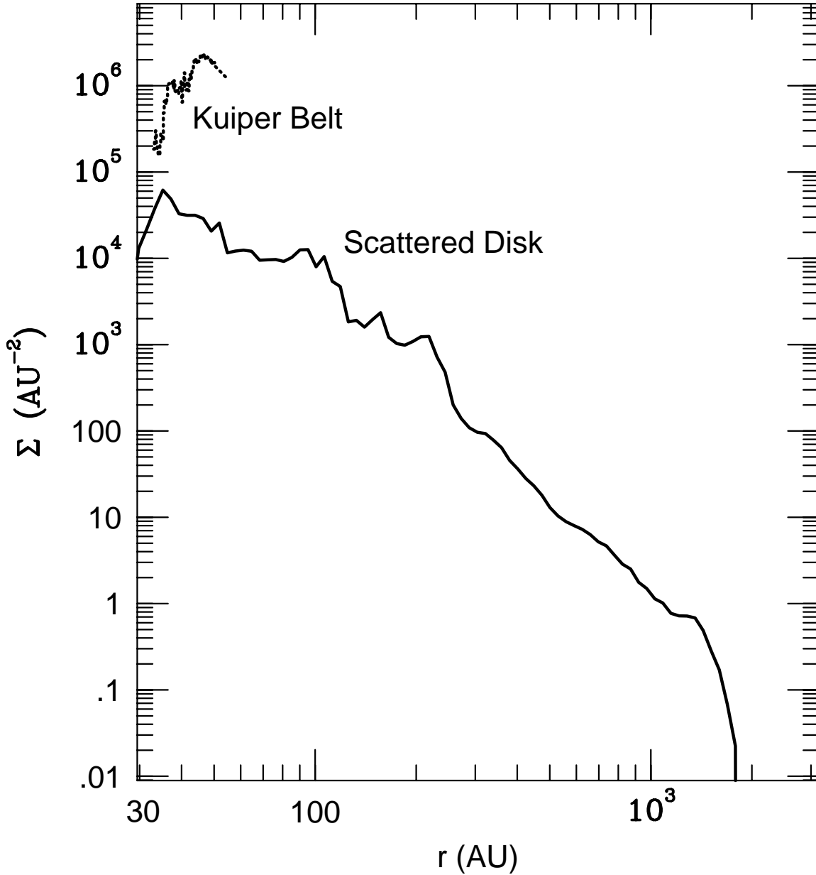
Fig. 7. The surface density of comets beyond Neptune for two different models of the source of Jupiter-family comets. The dotted curve is a model assuming that the Kuiper belt is the current source (Levison & Duncan 1997). There are 7 \times 10^9 comets in this distribution between 30 and 50 AU. This curve ends at 50 AU because the models are unconstrained beyond this point and not because it is believed that there are no comets there. The solid curve is DL97's model assuming the scattered disk is the sole source of the Jupiter-family comets. There are 6 \times 10^8 comets currently in this distribution.
