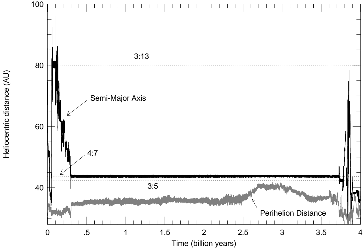
Fig. 6. The temporal behavior of a long-lived member of the scattered disk. The black curve shows the behavior of the comet’s semi-major axis. The gray curve shows the perihelion distance. The three dotted curves show the location of the 3:13, 4:7, and 3:5 mean motion resonances with Neptune.
