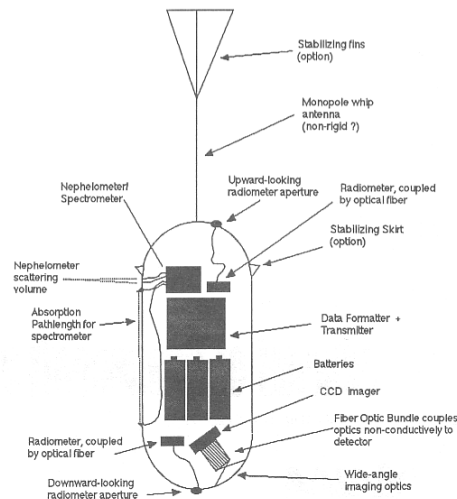
Fig. 1 Cross-sectional sketch of candidate microprobe configuration. The fins and/or skirt provide stabilization and spin control. The probe can be considered as a block of insulating material populated by electronic boxes.
