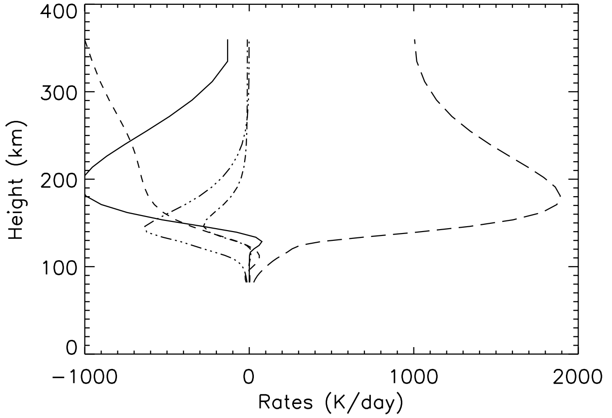
Thermal Balances for LT=15 at EQU MAX
