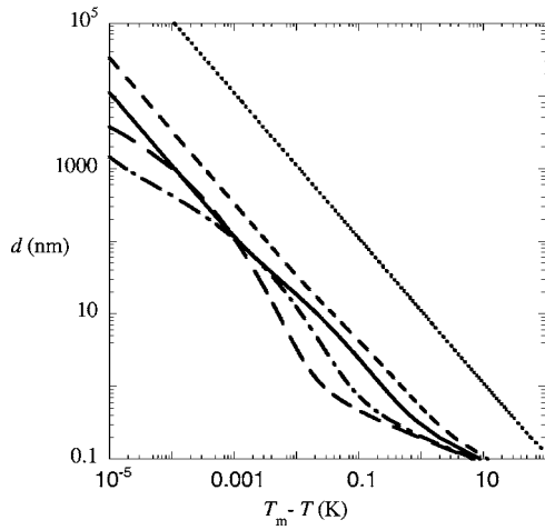
FIG. 4. Film thickness (nm) vs undercooling (K) at the interface between ice and water vapor. N_i=6 \times 10^{-4} (long dashed line), 6 \times 10^{-3} (dash-dotted line), 0.06 (solid line), 0.18 (small dashed line), and 6 \mu\text{M} NaCl (dotted line) per square meter. See the text for discussion. Adapted from Wettlaufer, 1999a .
