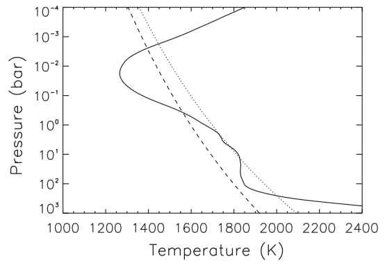
Fig. 9. The dayside temperature–pressure (T–P) profile of HD209458b from Showman et al. (2009) that includes a temperature inversion at low pressures. The condensation curves for forsterite (dotted line) and enstatite (dashed line) are shown.
