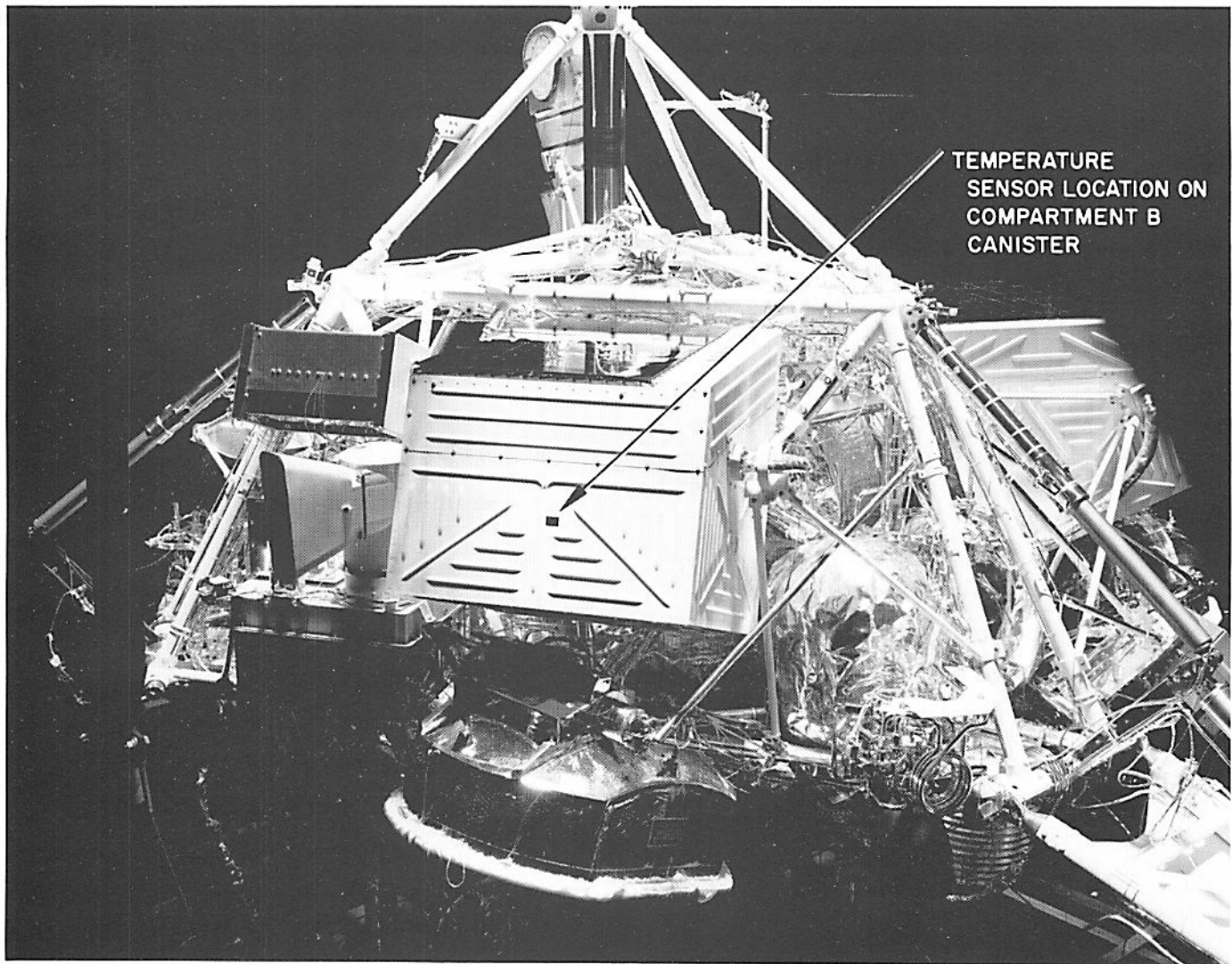
Fig. IV-5. Surveyor model showing compartment B
