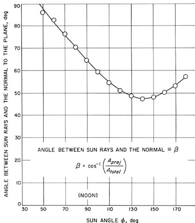
Fig. IV-10. Angle between sun rays and the normal to outboard plane of compartment B during first lunar day
