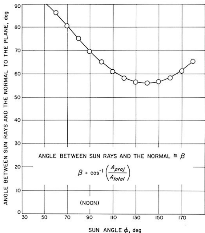
Fig. IV-9. Angle between sun rays and the normal to outboard plane of compartment A during first lunar day
