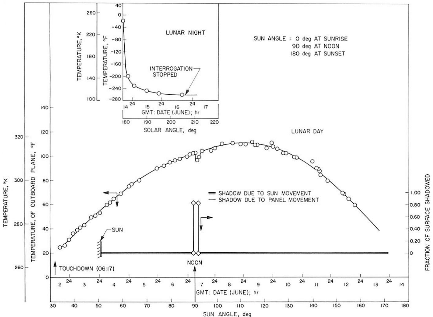
Fig. IV-8. Temperature and shadow of outboard face of compartment B during first lunar day and night
