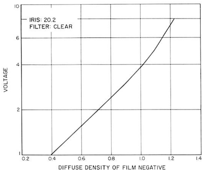
Fig. III-28. Typical plot of measured film density versus voltage from electronic grey scale
