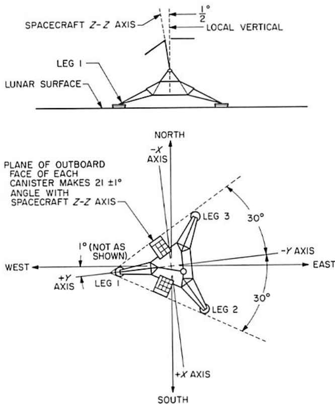
Fig. IV-6. Surveyor I spacecraft landed orientation
