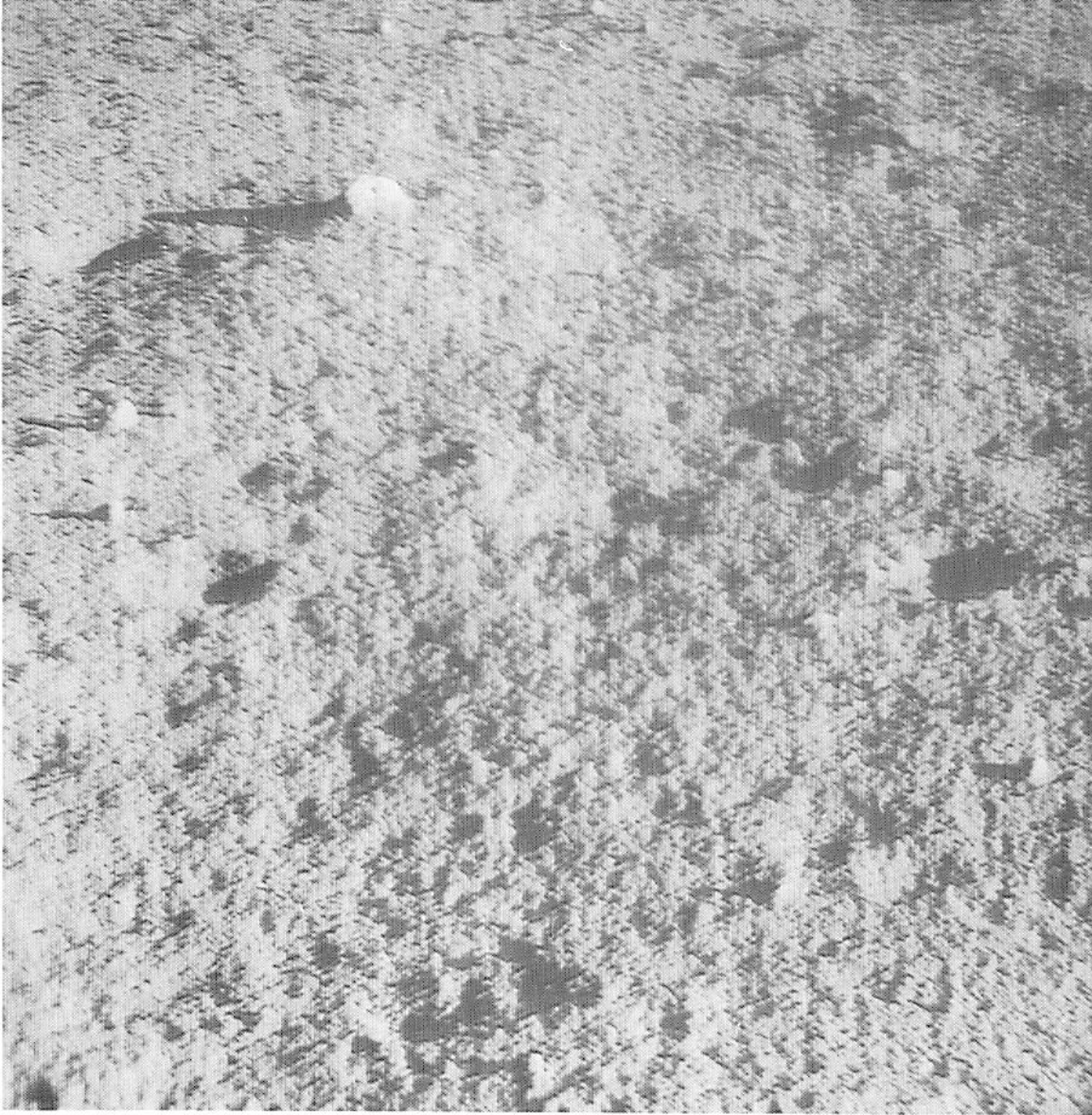
Fig. III-14. Area A: sun elevation of approximately 20^\circ
