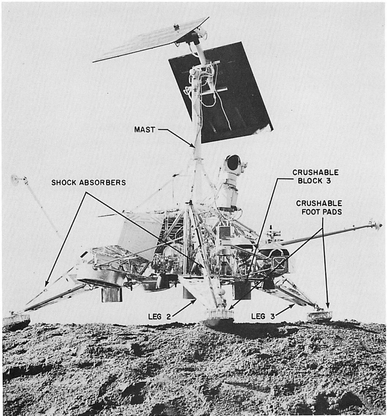
Fig. VI-1. Surveyor spacecraft
