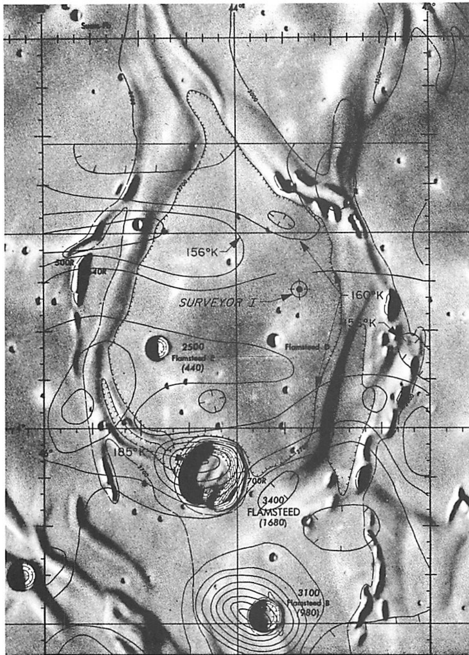
Fig. IV-1. Isotherms in landing site region during totality of lunar eclipse (Ref. IV-1)
