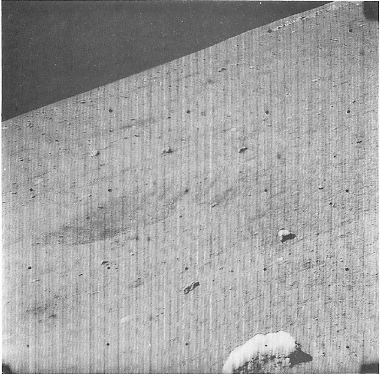
Fig. III-11. Crater approximately 3 m in diameter, southeast of spacecraft
