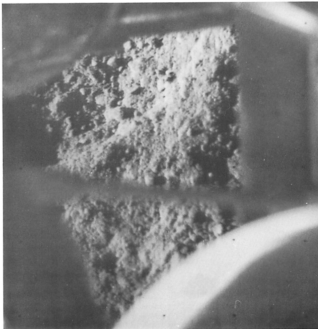
Fig. VI-13. Block assembly imprint taken late on the second lunar day. (Sun angle is 22^\circ and from the left of picture. No noticeable change in the disturbed material has been observed during a time period greater than 5 wk.)
