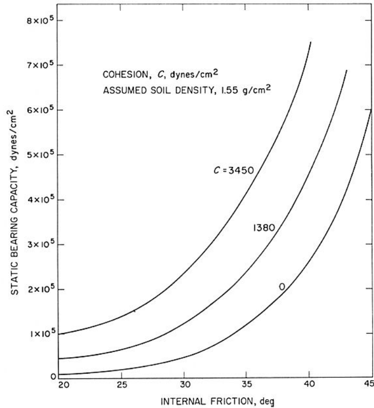
Fig. VI-15. Possible static bearing capacity of a 30.5-cm-diameter footing on moon
