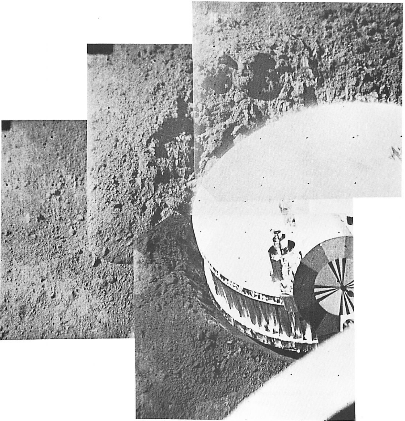
Fig. VI-7. Mosaic of computer-processed narrow-angle pictures of footpad 2 area taken on June 4, 1966. (Sun angle is 54^\circ .)
