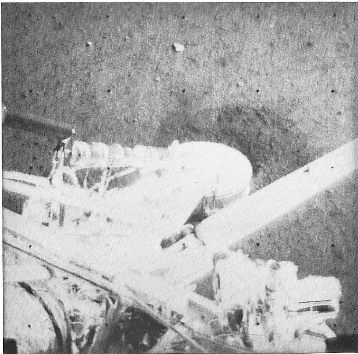
Fig. VI-6. Wide-angle picture of footpad 3 (Note similarity of throwout material to material shown in Fig. III-1.)
