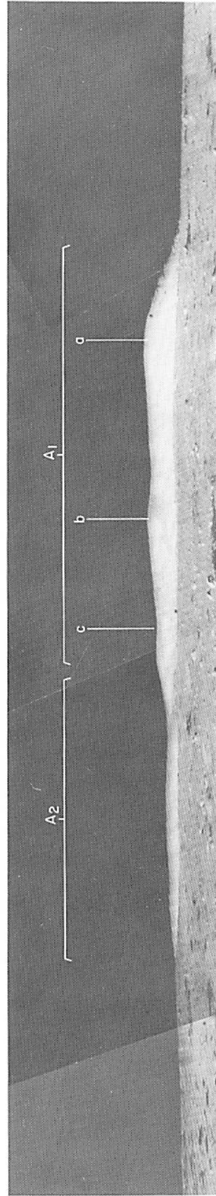
Fig. III-7. Enlargement of feature A in Fig. III-6
