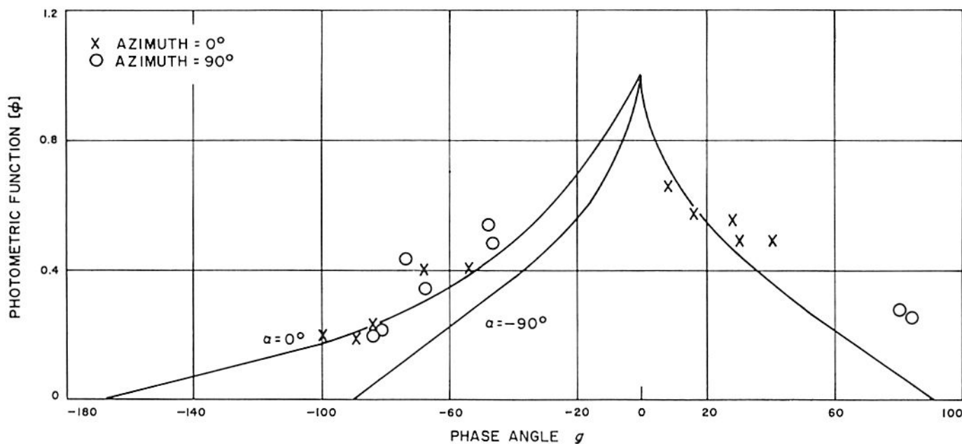
Fig. III-29. Photometric function versus phase angle. (Curves are mean values of terrestrially observed data.)
