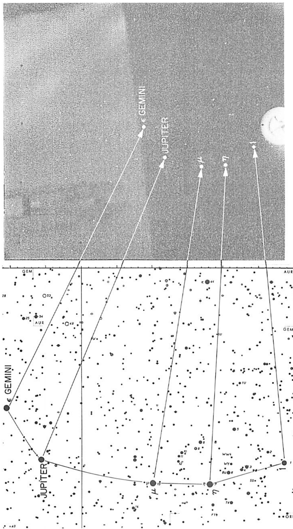
Fig. III-9. Jupiter and constellation Gemini taken on June 14, 1966, 16:14:22 GMT. (Additional marks on photograph are the reseau dots and vidicon surface blemishes.)
