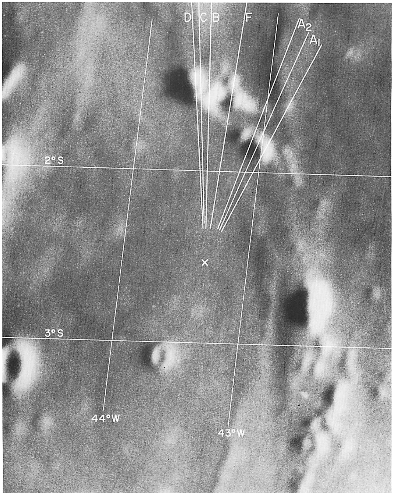
Fig. III-8. Relationship of horizon features to Surveyor landing site (lunar photograph by courtesy of E. A. Whitaker of the Lunar and Planetary Laboratory, University of Arizona)
