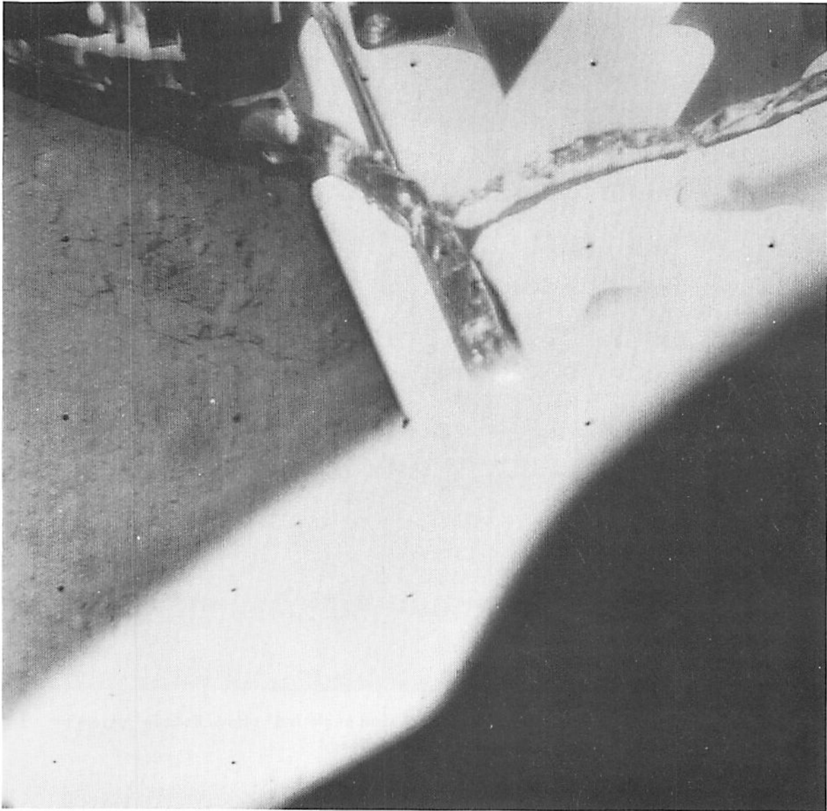
Fig. VI-9. Narrow-angle picture of disturbed lunar surface material near footpad 2. (Disturbed lunar material is in the approximate area in which the exhaust of the attitude control jet impinged on the surface.)
