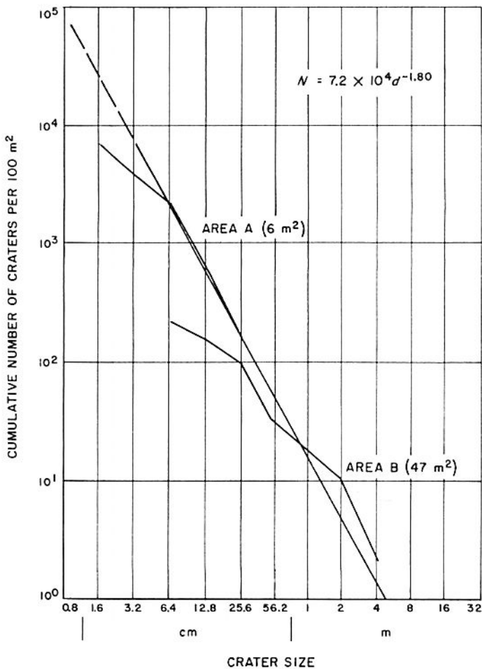
Fig. III-18. Cumulative size-frequency distribution of craters on lunar surface determined from Surveyor I pictures
