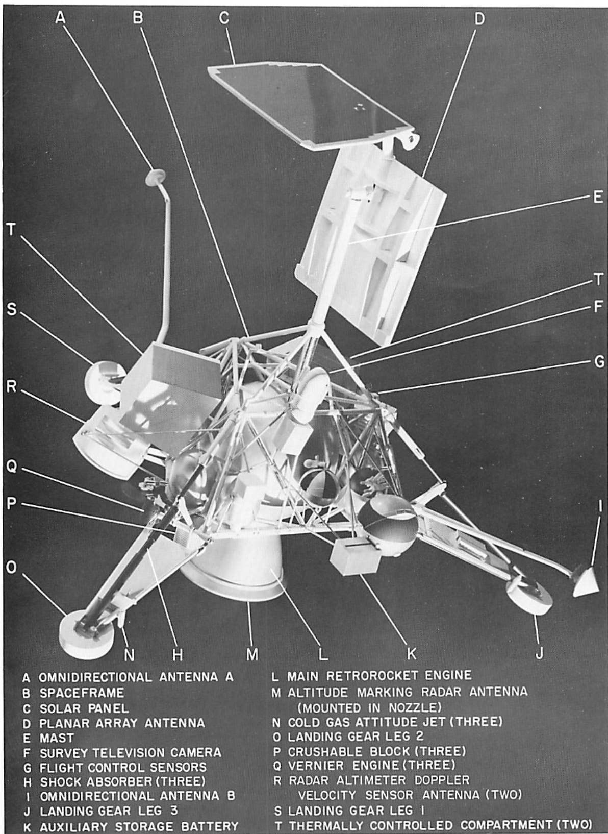
Fig. II-1. Surveyor 1 spacecraft configuration
