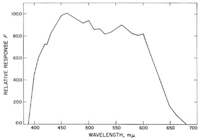
Fig. III-3. Spectral response curve of Surveyor I TV camera at clear position of filter wheel
