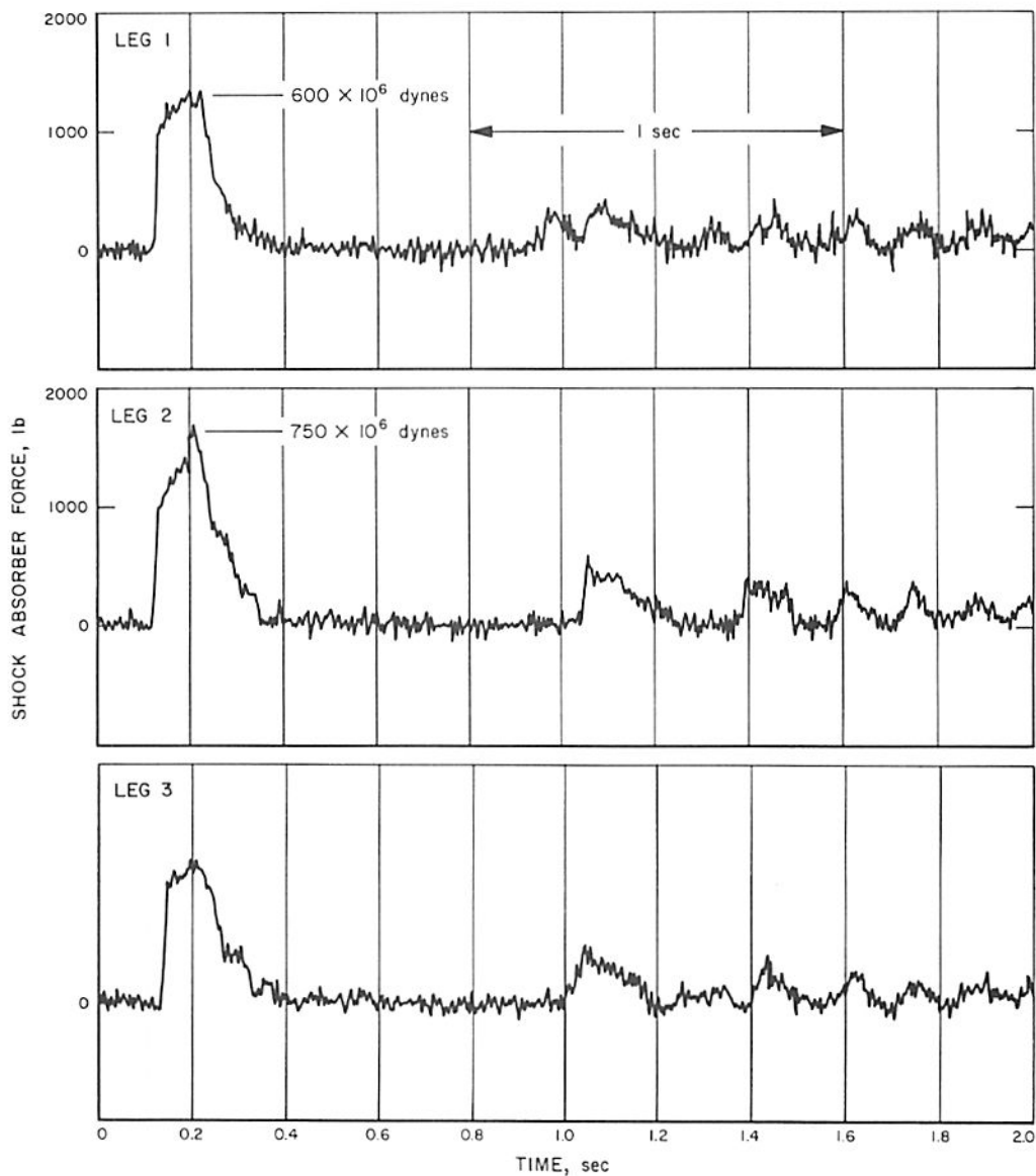
Fig. VI-4. Axial shock absorber strain gage data. (Maximum force developed by shock absorber 3 is not shown because of uncertainties in No. 3 strain gage calibration.)
