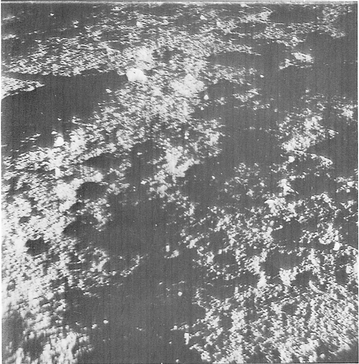
Fig. III-13. Area A: sun elevation of approximately 8^\circ
