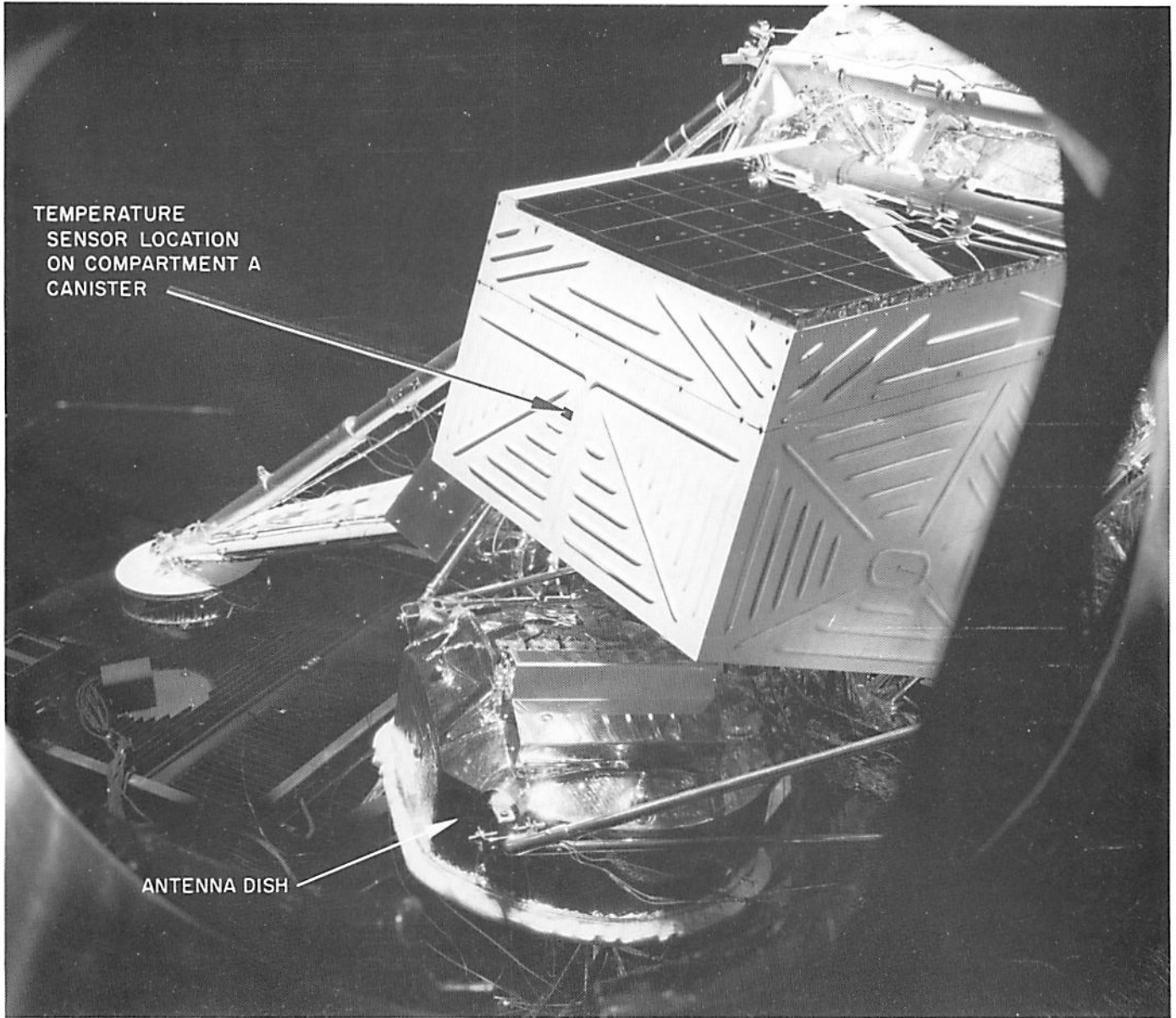
Fig. IV-4. Surveyor model showing compartment A
