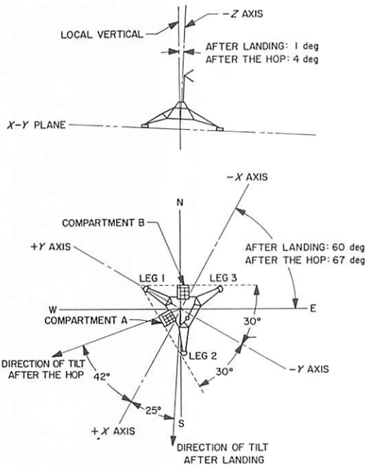
FIGURE 5-5. — Surveyor VI orientation.
