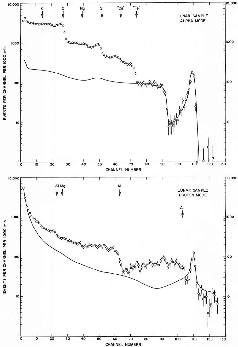
FIGURE 7-11.—Data obtained by means of Surveyor VI alpha-scattering experiment in the alpha and proton modes during 790 minutes of measurement on the lunar surface. The experimental points are indicated with (1\sigma) statistical errors. The data have been corrected to standard instrument response. The solid curve in each case is a smoothed version of the background observed in the previous stage of lunar operations.
