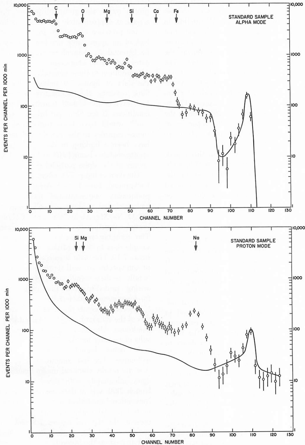
FIGURE 7-9. — Results of data taken on the Surveyor VI mission by the alpha-scattering instrument in the alpha and proton modes during 280 minutes of measurement of the standard sample after lunar landing. The experimental points are indicated with statistical ( 1\sigma ) error bars. They have been corrected approximately by using the temperature coefficient of the instrument. For comparison, the smooth curve shows the approximate magnitude of the background (fig. 7-8).
