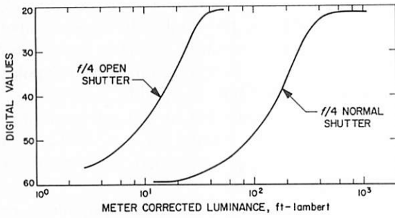
FIGURE 3-29.—Digitized plot of the light-transfer characteristic of the Surveyor television camera in the part of the picture format that contains the right side of the Sun's corona. The open-shutter data were obtained during preflight calibration at the f/8 iris position and extrapolated to f/4 .
