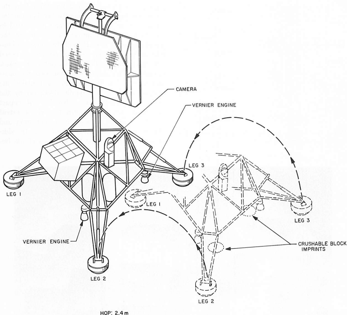
FIGURE 4-3. — Surveyor spacecraft trajectory during hop.
