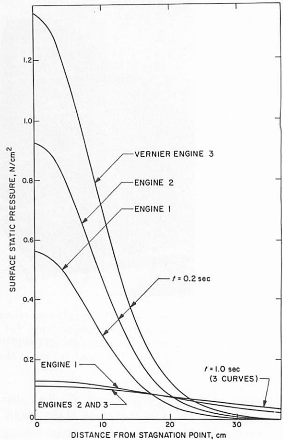
FIGURE 4-47.—Theoretical static pressure, along a surface parallel to the engine nozzle exit plane, 0.2 and 1.0 second after initiation of the hop.
