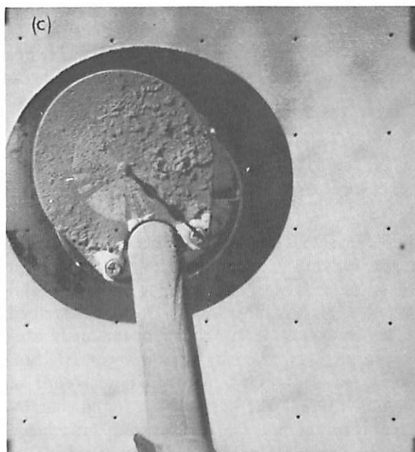
FIGURE 3-28.—Photometric target on the boom of the omnidirectional antenna, which was partially covered by lunar material blown by vernier engine 3 during the hop. (a) Target a few hours before the hop (day 321, 09:37:05 GMT). (b) Target with the Sun's rays at an angle of 17^\circ on the surface of the target (day 321, 12:29:08 GMT). (c) Target illuminated by the Sun's rays at an angle of 70^\circ to the surface of the target. More of the target can be seen under direct illumination (day 326, 06:47:06 GMT).
