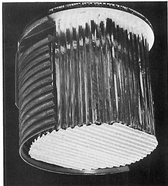
FIGURE 4-25. — A crushable block, with corrugated thermal shield.
