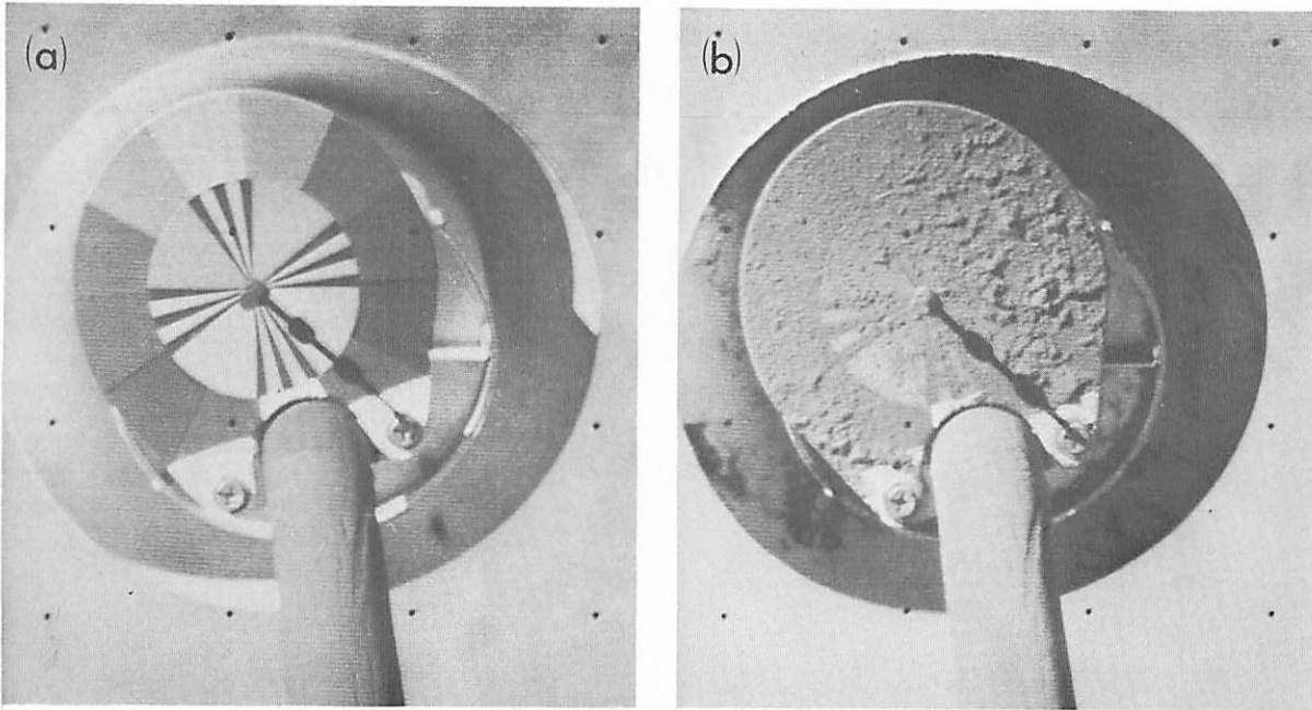
FIGURE 4-39. — Photometric target on omnidirectional antenna boom B : (a) before and (b) after the vernier engine firing. Before the firing, the target is clean; after the firing the target is coated with a layer of soil up to 0.9 mm thick. The coating probably was caused by impact of a soil clump on the target during the firing. (a) Day 321, 09:37:11 GMT; (b) day 321, 12:30:00 GMT.
