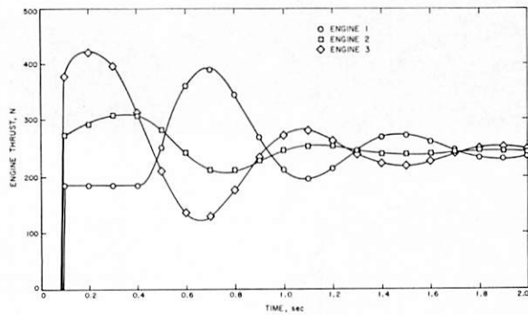
FIGURE 4-20. — Variation of vernier engine thrust with time during the hop.
