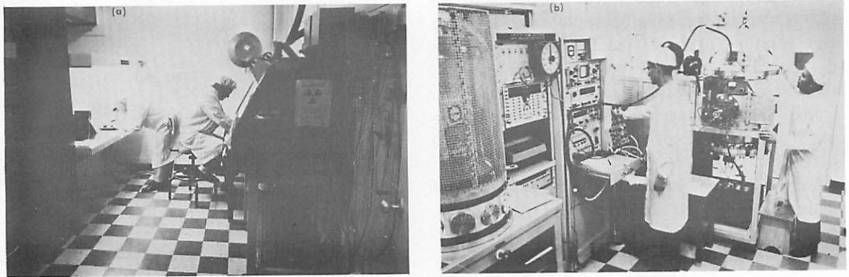
FIGURE 7-4. — Source loading and calibration facilities at Cape Kennedy, Florida. Shown are the source loading room (a) and the instrument calibration room (b) as they were during prelaunch operations of the alpha-scattering experiment for the Surveyor VI mission. On the left side of the source loading room (a) is a laminar-flow clean bench. When the sensor head was removed from the spacecraft for the final operation at Cape Kennedy, it was kept in a "handling container." The frame in which this container was maneuvered during source loading is shown on the clean bench. On the right side of this room is an enclosed hood of the type used for handling alpha radioactivity. In the instrument calibration room (b) two large vacuum chambers are visible. These were used for testing and storage of the sensor head and its spare. Also shown is the electronic equipment for instrument control and data analysis.
