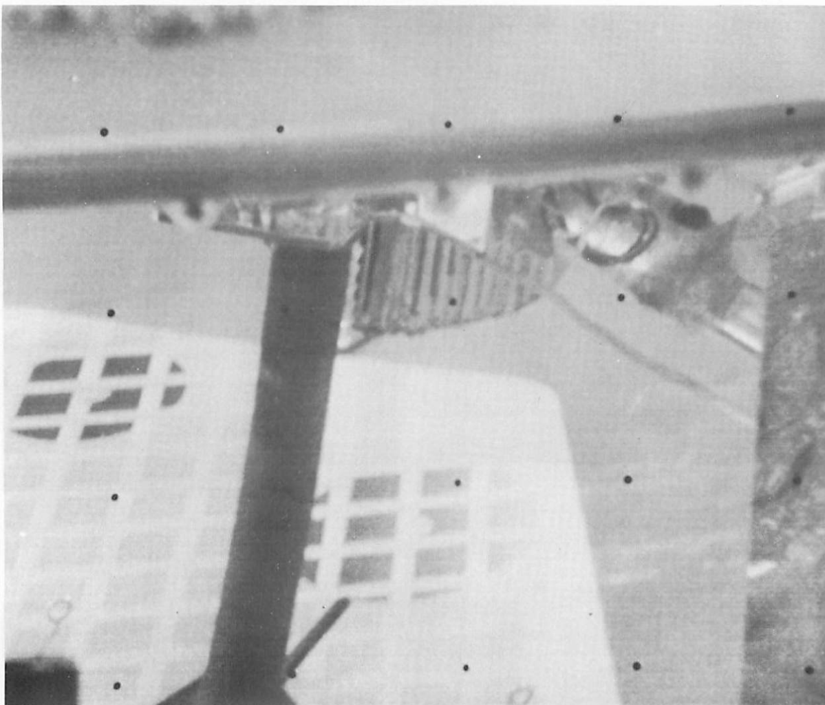
FIGURE 4-16. — Reference picture taken by the Surveyor VI television camera after final calibration and alignment before launch. Crushable block 3 can be seen near the top of the auxiliary mirror image. The large circle, indicating the area directly below the crushable block, has been positioned to simulate a 7.6-cm footpad penetration. (The black vertical post in the center of the picture is a support used during prelaunch checkout.)
