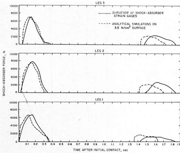
FIGURE 4-17. — Initial landing data and analytical shock-absorber force/time histories.
