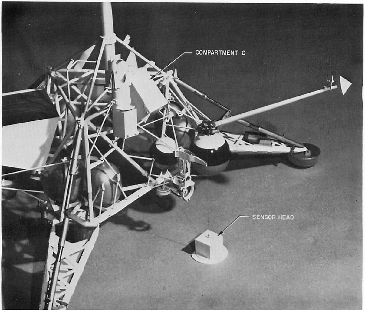
FIGURE 7-1. — Photograph of a 1/5-scale model of a Surveyor spacecraft showing the location of the alpha-scattering instrument. The sensor head is shown in its nominal lunar surface position. Electronic cables are not simulated on this model.
