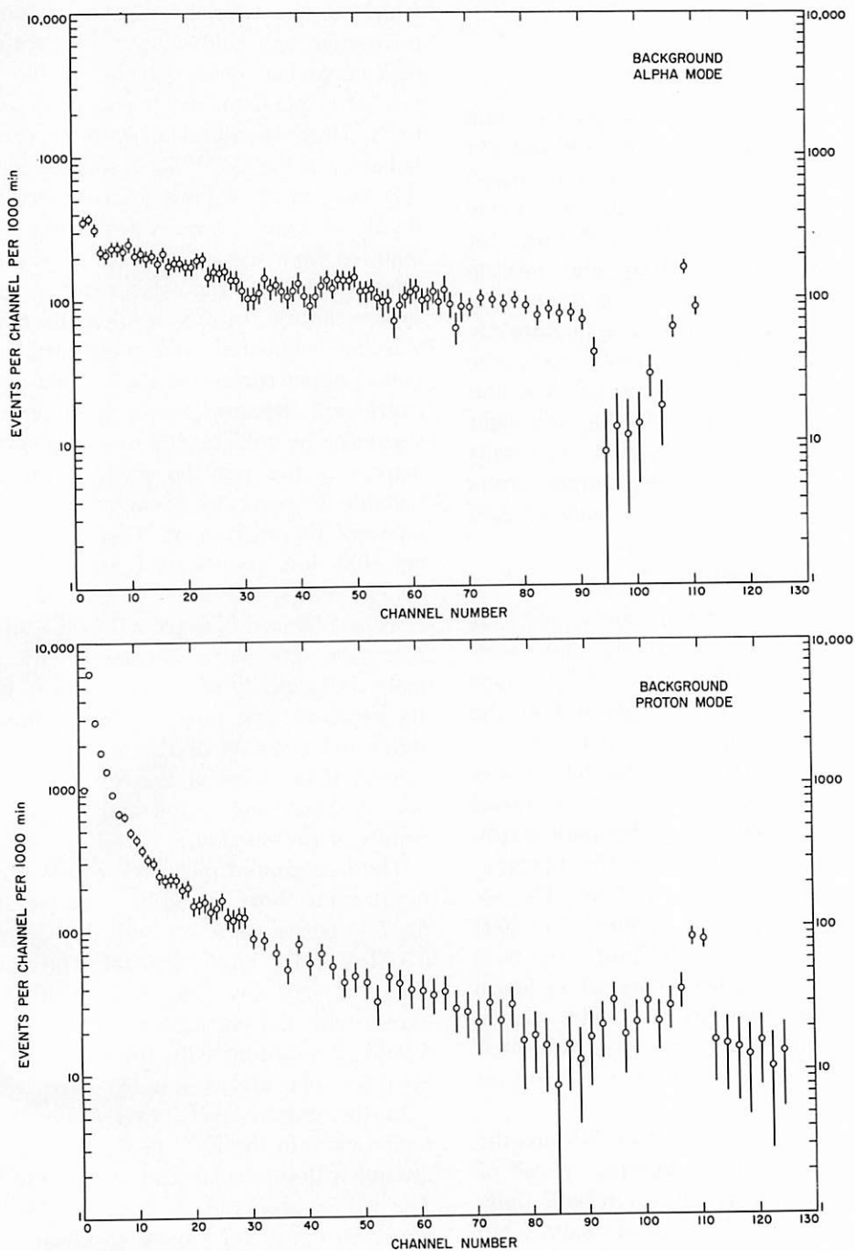
FIGURE 7-8. — Results of data taken on the Surveyor VI mission by the alpha-scattering instrument in the alpha and proton modes during 366 minutes of measurement during the background phase on the Moon. The experimental points with statistical ( 1\sigma ) errors are averages of two channels in the regions of low counting rates to improve their statistical significance. The experimental points have been corrected approximately by using the temperature coefficient of the instrument. The peaks at approximately channel 110 in both modes are due to \text{Es}^{254} placed near the detectors before launch.
