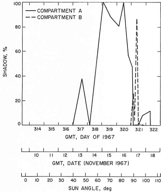
FIGURE 5-8. — Percentage of shadow on outboard faces of compartments A and B.
