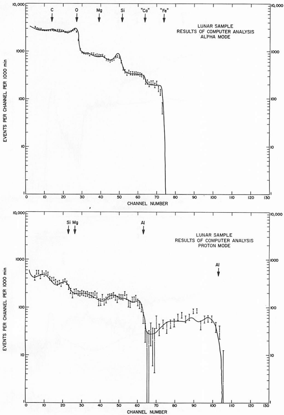
FIGURE 7-12. — The calculated spectra (smooth curves), using an eight-element library, are compared with the data (points with 1\sigma error bars) taken during 790 minutes of analysis. The background (fig. 7-8) has been subtracted before the comparison was made. The computer analysis has been made over channels 8 to 85 for the alpha mode, and over channels 8 to 110 for the proton mode.
