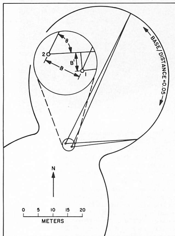
FIGURE 3-9. — Geometry of Surveyor VI photogrammetry.
