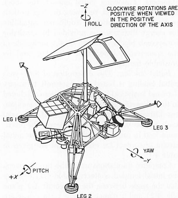
FIGURE 4-2. — Surveyor spacecraft configuration and coordinate system.
