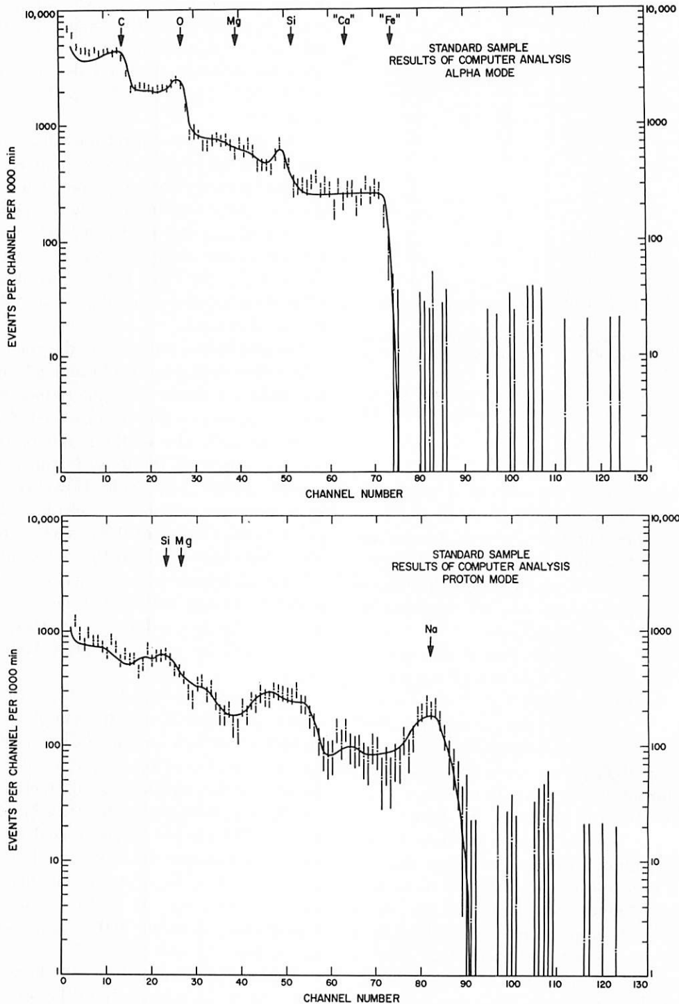
FIGURE 7-10.—The calculated spectra (smooth curves), using an eight-element library, are compared with the data (points with 1\sigma error bars) taken during 280 minutes of analysis of the standard sample on the Surveyor VI mission on the Moon. The background (fig. 7-8) has been subtracted before the comparison was made. The computer analysis has been made over channels 8 to 85 in the alpha mode and over channels 8 to 110 in the proton mode.
