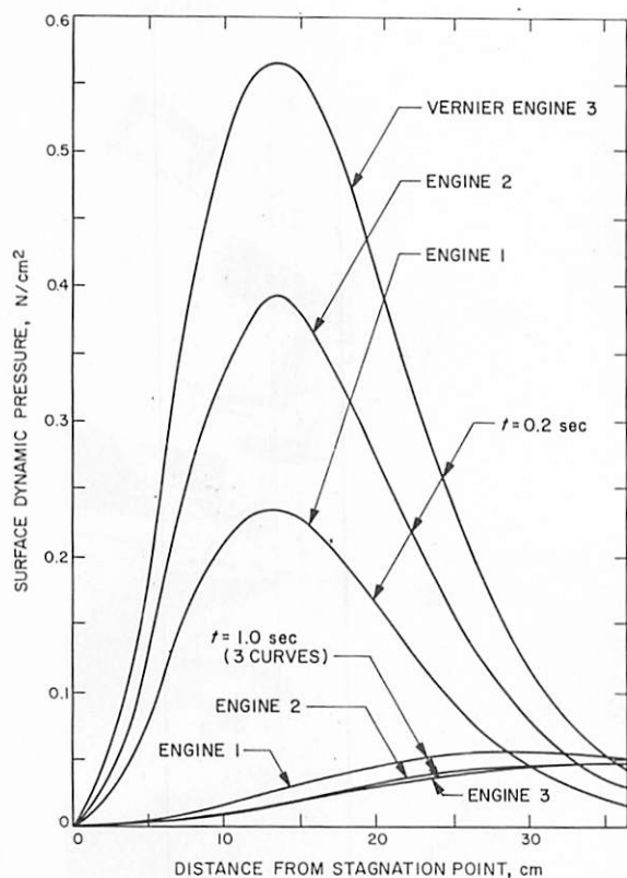
FIGURE 4-48.—Theoretical dynamic pressure developed by the three vernier engines along a planar surface parallel to the engine nozzle exit plane 0.2 and 1.0 second after initiation of the hop.
