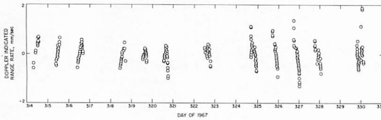
FIGURE 10-9. — Surveyor VI, DSS 42 (Canberra, Australia). First lunar day, O — C residual set (compressed five data points/min). DE 29/LE 5 was used.
