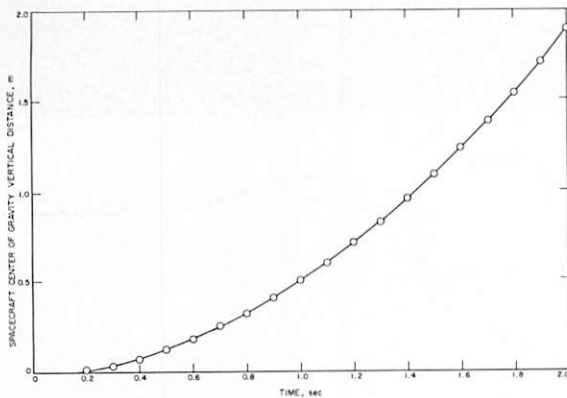
FIGURE 4-18. — Change of vertical height with time during the hop.
