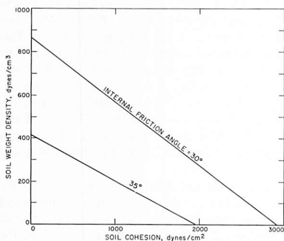
FIGURE 4-49.—Values of soil cohesion and weight density for which the maximum loading under vernier engine 3 is equal to the soil bearing capacity.
