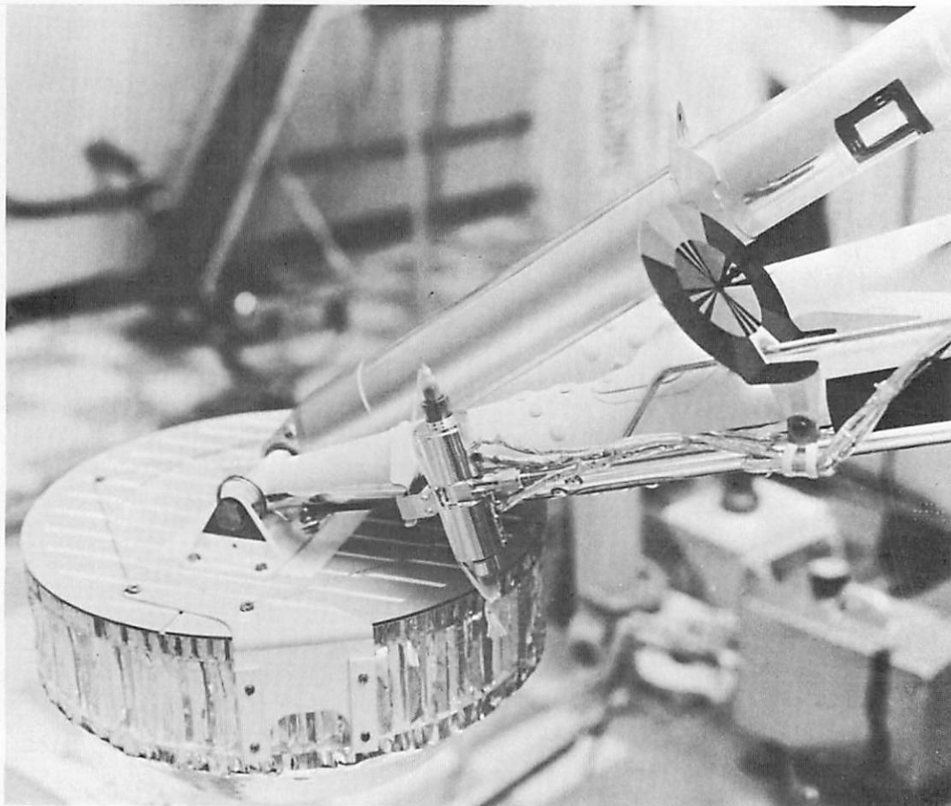
FIGURE 4-50. — A Surveyor leg 2 assembly showing the attitude control jet mounted between the footpad and the photometric target.
