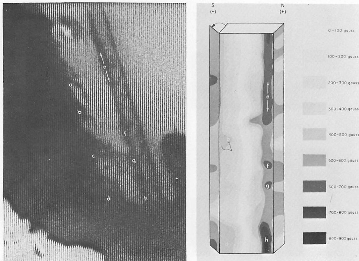
FIGURE 8-10. — Comparison of enlarged view of Surveyor VI magnet with tonal plot of gauss strength. (Compare with fig. 8-3.) Letters indicate the same relative areas on the lunar magnet and on the magnetic-strength plot.
