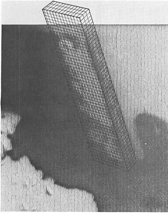
FIGURE 8-11.—Enlarged view of Surveyor VI magnet with transparent grid overlay. Grid line spaces are equivalent to 1 mm, which is approximate resolution of the Surveyor VI camera. Most particles appear to be <1 mm; some may be \approx 1 mm. All appear to occur in clumps or groups of particles.
