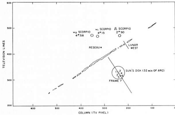
FIGURE 3-30.—Diagram showing the position of the Sun's disk in relation to the horizon and beads at 14:25:25 GMT on day 328. The position of the center of the Sun is also indicated for other frames showing the bright line on the horizon. The stars \omega_1 and \omega_2 Scorpio are those used to determine the Sun's position. The magnitudes of these stars are indicated beside the circles. The grid coordinates refer to position in the digital frame.
