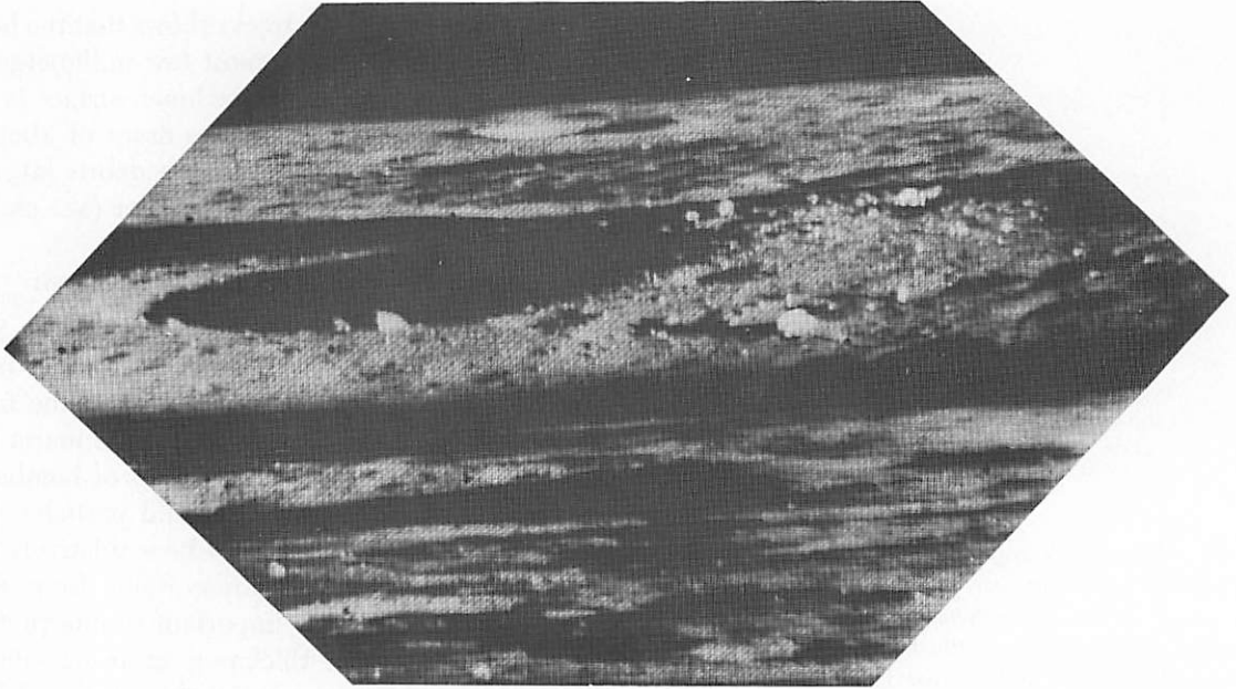
FIGURE 3-25.—Wide-angle picture looking northeast of the Surveyor VI landing site. Crater with the blocky sharp raised rim near the center horizon is about 22 meters in diameter and 700 meters from Surveyor VI. The crater with the blocky rim in the center of the picture is 30 meters in diameter and 350 meters from Surveyor VI. These craters lie on a ridge east of the spacecraft (day 328, 11:47:30 GMT).
