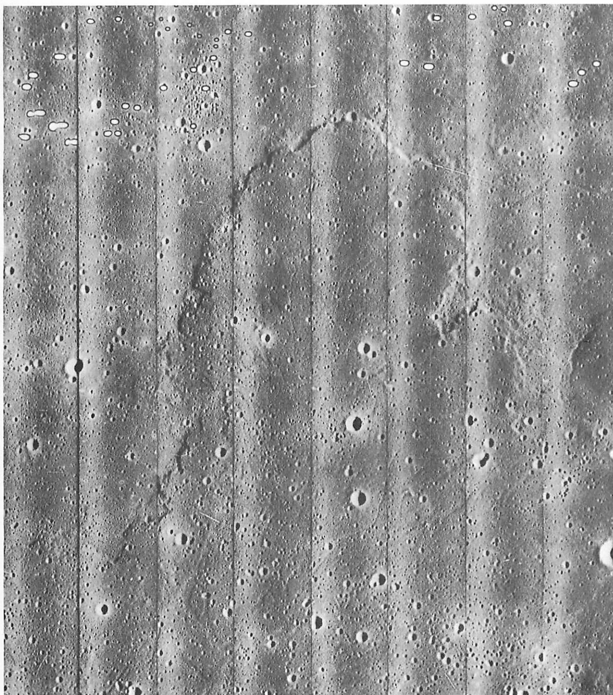
FIGURE 9-1. — Medium-resolution Lunar Orbiter photography showing flow structure in Mare Imbrium.
