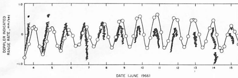
FIGURE 10-11. — Combined amplitude and period of the J_{20} defect and the faulty fit of observations to Brown's lunar theory are plotted to the same scale as the Surveyor I O — C residual set.
