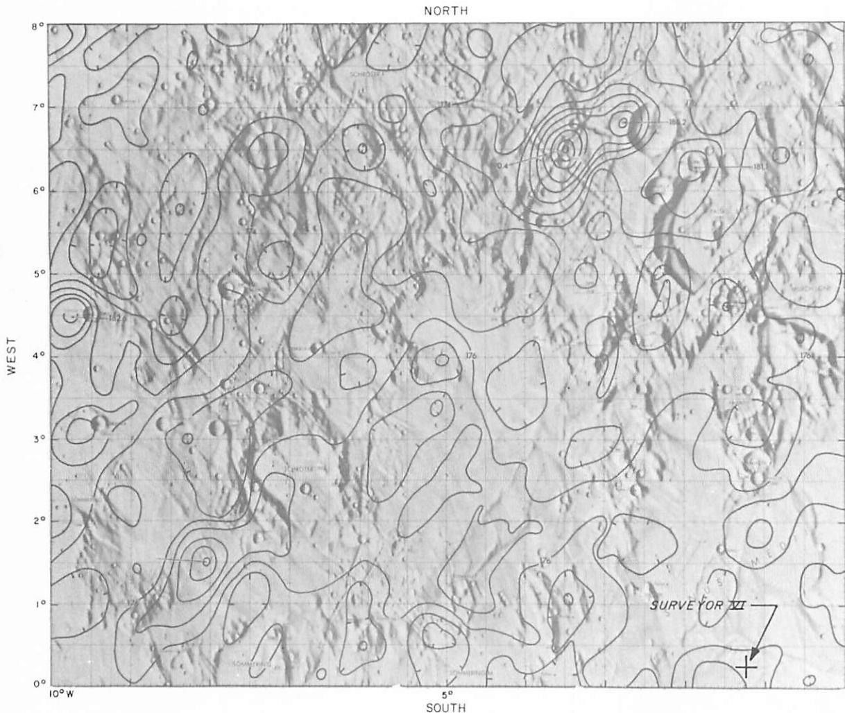
FIGURE 5-3. — Isothermal contours ( ^{\circ}\text{K} ) for landing site region obtained during totality of lunar eclipse of December 19, 1964.
