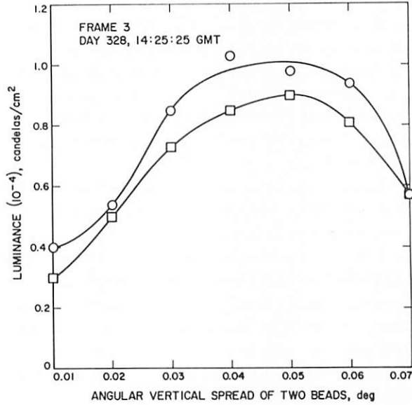
FIGURE 3-32.—Luminance versus angular spread of two beads measured in frame 3. The photometric cross section of each bead was obtained along the vector from the bead to the Sun's center as shown in fig. 3-30.
