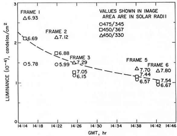
FIGURE 3-33.—Luminance of the corona measured at three constant picture frame positions as a function of time. The distance of these positions from the center of the Sun's disk is given in solar radii beside each data point. The curve is an indication of the trend of the data and does not represent absolute luminance values.
