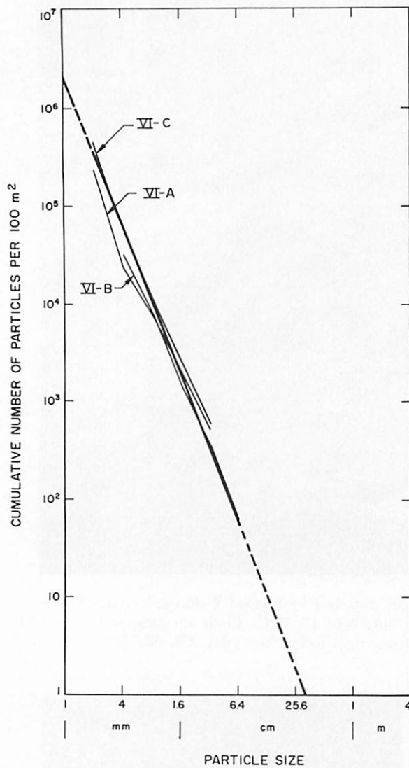
FIGURE 3-21. — Cumulative size-frequency distribution of fragments determined for three sample areas from Surveyor VI pictures.
