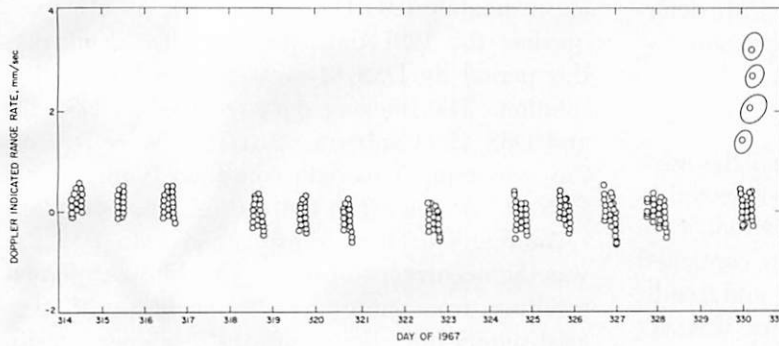
FIGURE 10-3. — Surveyor VI, DSS 42 (Canberra, Australia). First lunar day, O - C residual set (one data point/min). DE 29/LE 5 was used.
