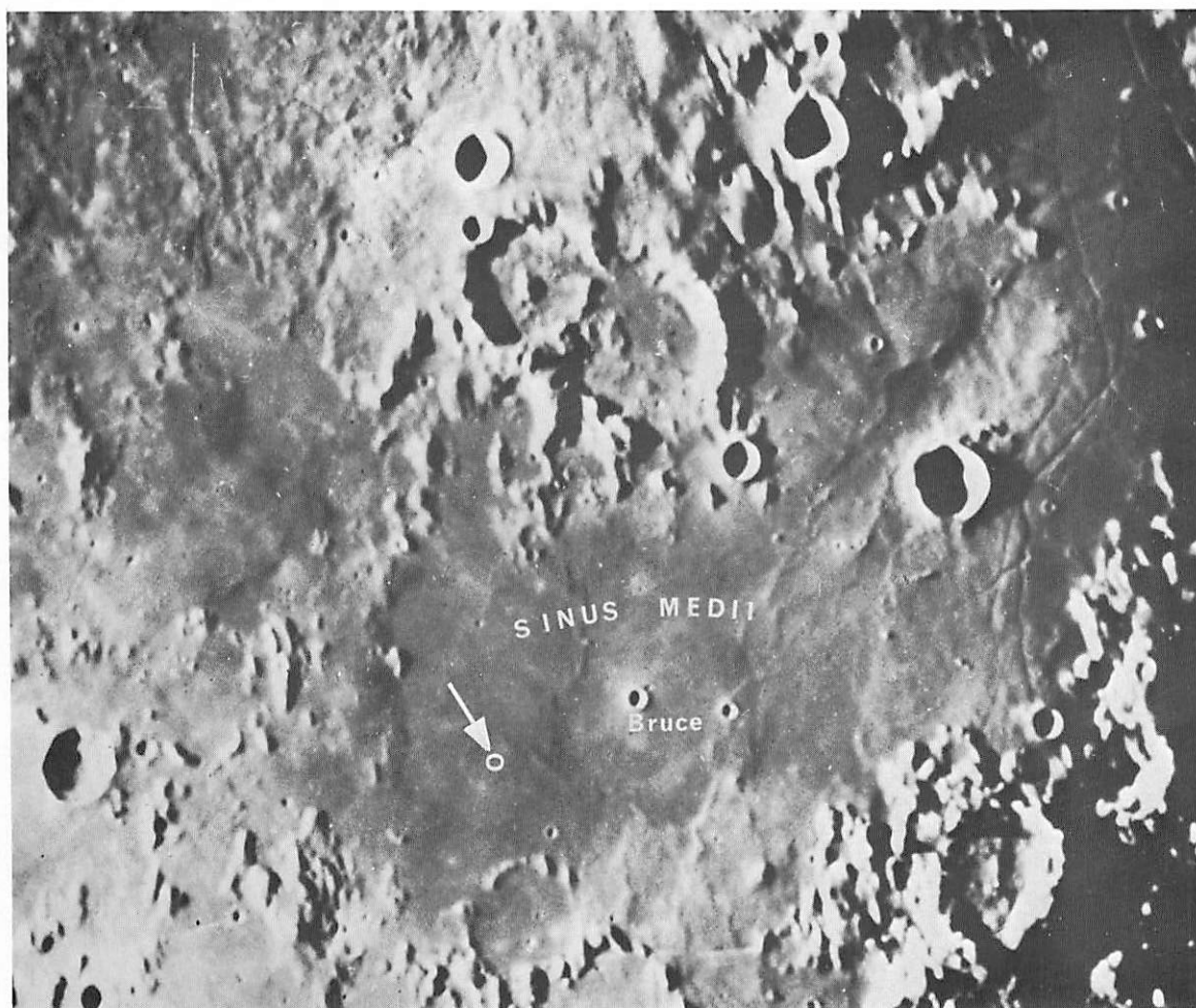
FIGURE 3-3. — Photograph of the central region of the Moon taken through the 100-inch telescope at Mt. Wilson Observatory, Calif. The white circle indicates the location of Surveyor VI, which landed in Sinus Medii at 0.49^{\circ} N latitude, 1.40^{\circ} W longitude.
