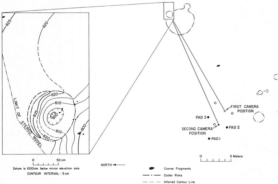
FIGURE 3-11. — Maps prepared from stereoscopic Surveyor television pictures. The sketch on the right shows the position of the camera and spacecraft footpads before the hop (open circles) and after the hop (solid circles). A few craters and a prominent block (east of the spacecraft) were plotted graphically by triangulation. The contour map on the left was drawn from stereoscopic pictures with the Surveyor anaglyphic stereoplotter shown in fig. 3-8.
