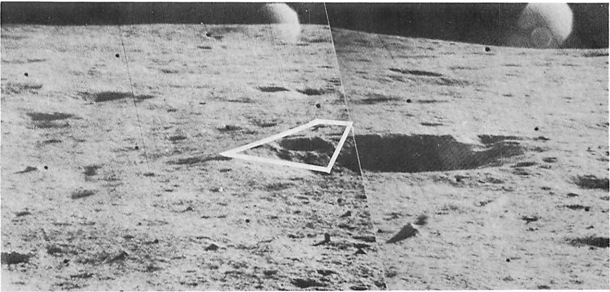
FIGURE 3-10. — Crater, 1 meter in diameter, which lies 20 meters northeast of the Surveyor VI spacecraft. A detailed contour map of the area outlined was made with the stereoplotter (day 315, 04:21:17 and 04:20:24 GMT).
