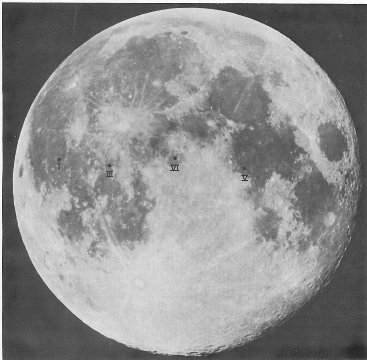
FIGURE 8-1.— Photograph of the Moon showing the location of landed Surveyor spacecraft. Note Surveyor V in Mare Tranquillitatis and Surveyor VI in Sinus Medii; Surveyors V and VI have had the magnet assembly attached to footpad 2 (Table Mountain Observatory photograph taken on Feb. 28, 1964, at 07:55:23 UT).
