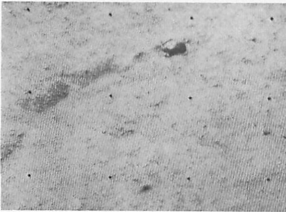
FIGURE 3-26.—Track made by a fragment 2 cm in diameter rolling across the lunar surface near Surveyor VI. The rolling fragment has disturbed a light fragile layer of surface material and exposed darker material 1 or 2 mm beneath (day 321, 07:13:54 GMT).
