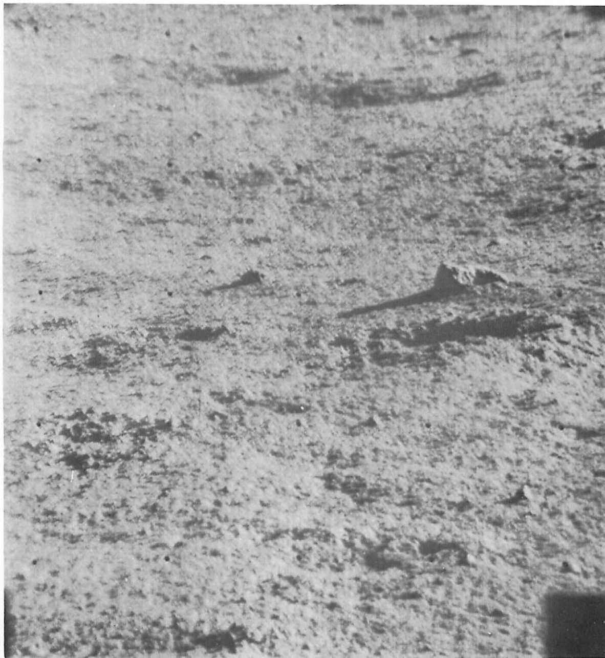
FIGURE 3-13.—Narrow-angle picture showing several small, irregular, secondary impact craters about 15 to 30 cm in diameter with rubbly material in the bottom and around the rims. Note the asymmetric shape of a 30-cm secondary impact crater in the upper right of the picture (day 315, 02:02:18 GMT).
