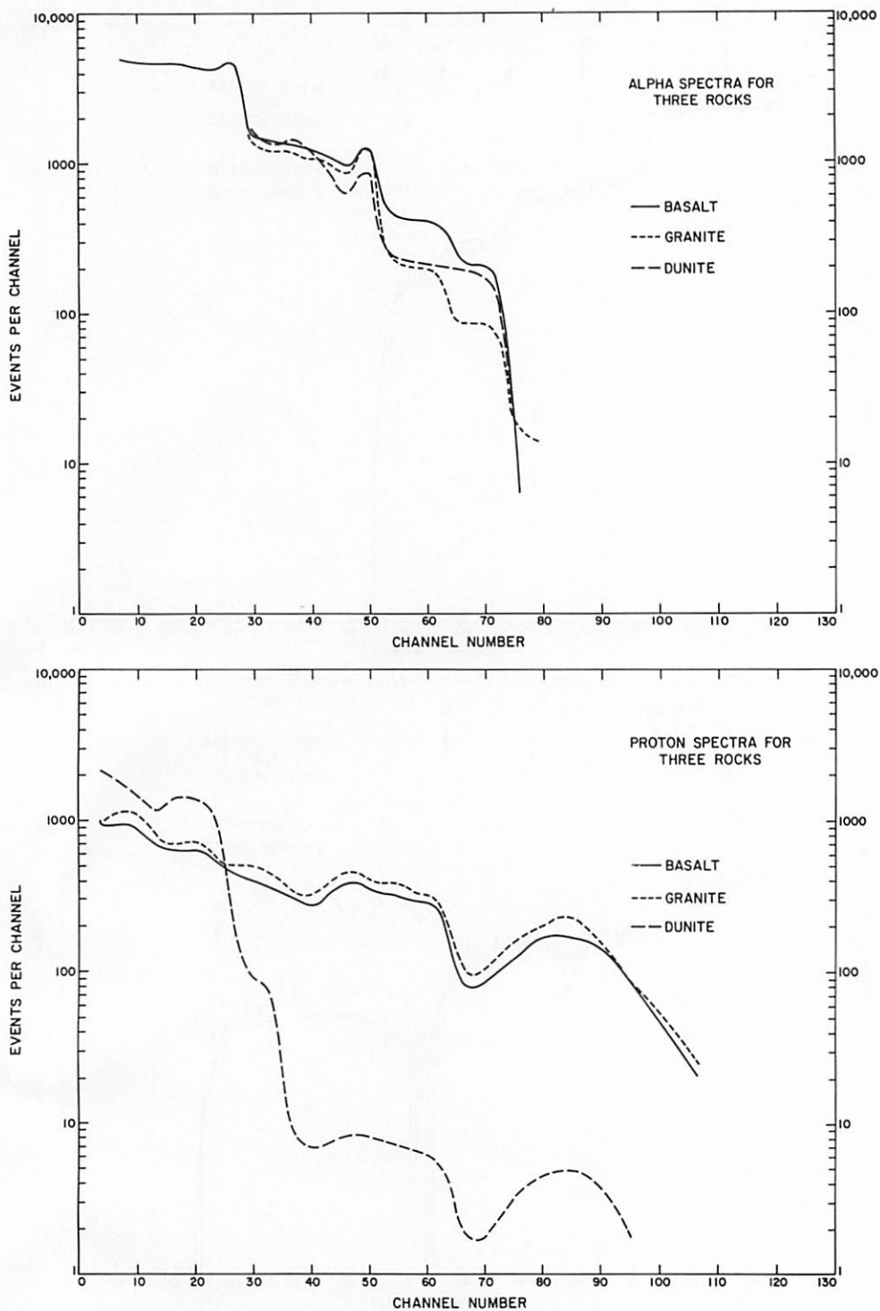
FIGURE 7-14. — Alpha-scattering instrument response from three rocks. Data taken with a Surveyor prototype instrument (P-2) on samples of basalt (USGS-W-1), granite (USGS-G-2), and dunite (USGS-DTS-1). All data from each rock have been multiplied by a factor to make the responses equal in the oxygen region of the alpha mode.
