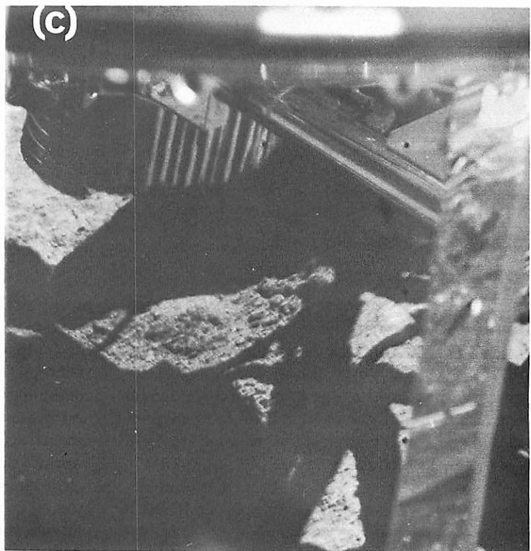
FIGURE 4-15.—Narrow-angle pictures of crushable block 3 and its impression on the lunar surface. Pictures were taken through the auxiliary mirrors of different Sun elevation angles. (a) Sun elevation of 15^\circ (day 315, 01:28:20 GMT); (b) Sun elevation angle of 30^\circ (day 316, 07:08:08 GMT); and (c) Sun elevation angle of 65^\circ (day 319, 03:57:13 GMT).
