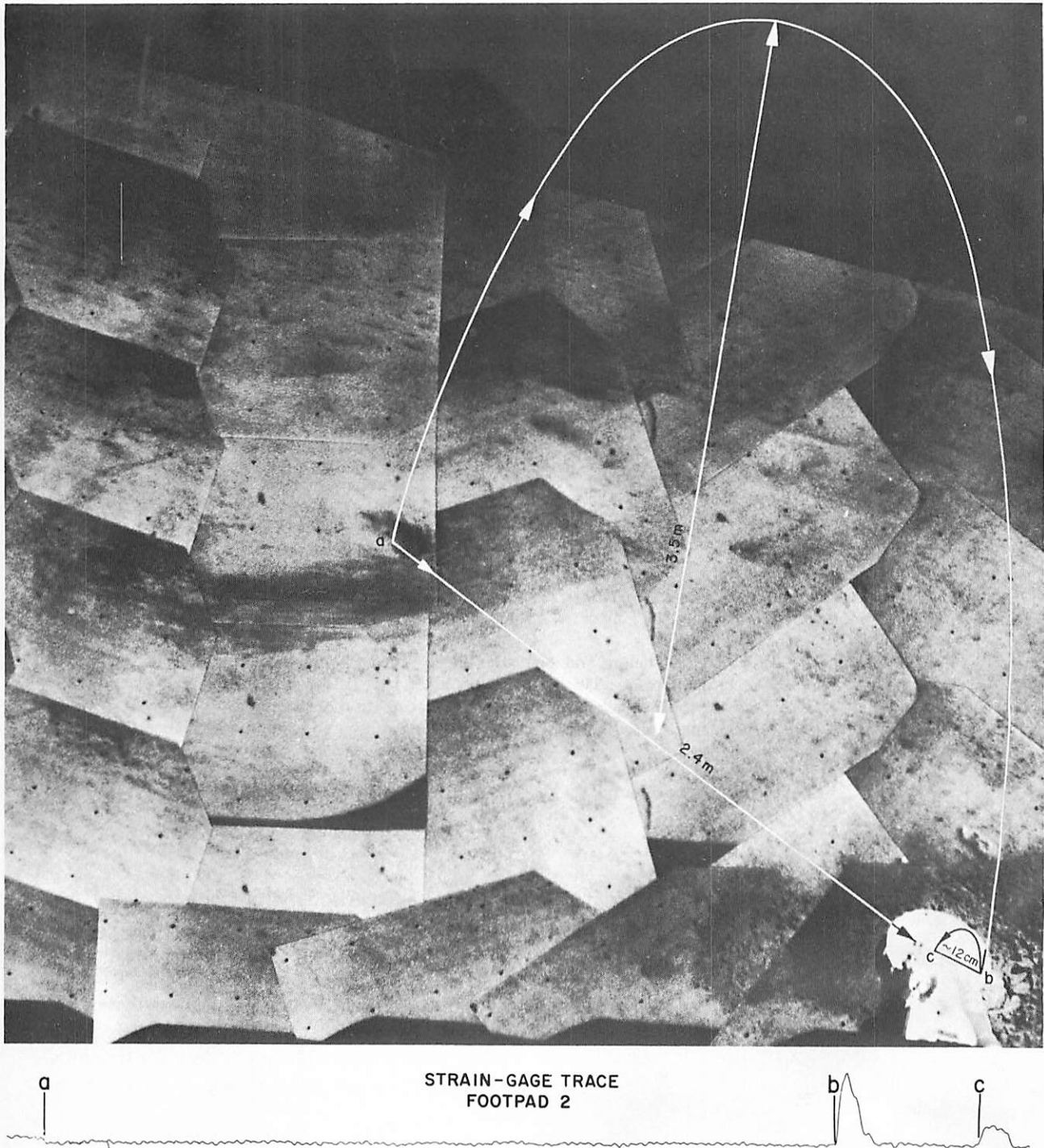
FIGURE 8-6.—Hopping movement followed by footpad 2. The original landing point of footpad 2 is seen at position (a). The spacecraft rose about 3.5 meters and landed (b) at a position about 2.4 meters to the southwest. In landing, a small bounce occurred at footpad 2, to the left (c). Penetration appears to have been up to 10 cm, causing the lower seven-eighths of the magnet to contact lunar surface material. The strain-gage data for footpad 2 seen at the bottom indicates that the movement from (b) to (c) was a bounce rather than a slide.
