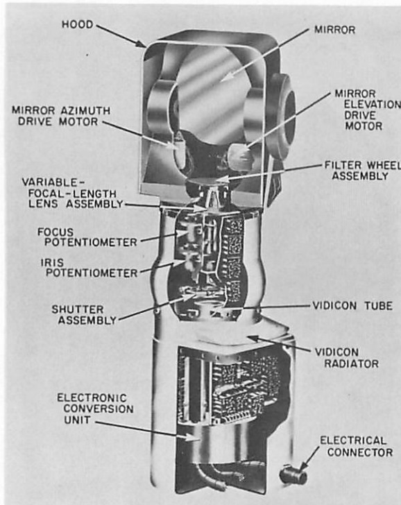
FIGURE 2-2. — Cutaway view of survey television camera.
