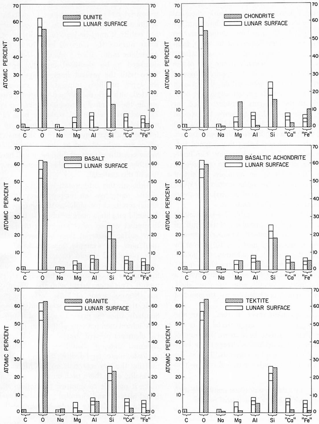
FIGURE 7-15. — Comparison of the observed chemical composition of the Surveyor VI lunar sample (open bars) with the average composition of selected materials (cross-hatched bars). The dunite and basaltic achondrite values are from ref. 7-6; the basalt values are for Continental basalts from ref. 7-7; the granite values are for the North American crust from ref. 7-8; the chondrite values are the averages of the low-iron group from ref. 7-9; the tektite values are those for the Indo Malayan body quoted in ref. 7-6.
