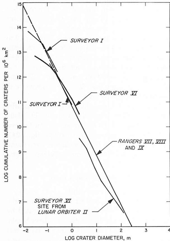
FIGURE 3-15. — Cumulative size-frequency distribution of small craters determined from Surveyor VI pictures and Lunar Orbiter II photographs compared with the cumulative size-frequency distribution of small craters determined from Surveyor I pictures and on the mare planes determined from Rangers VII, VIII, and IX pictures.
