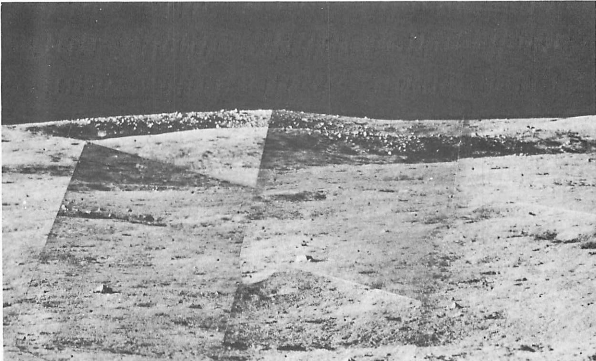
FIGURE 3-24. — Mosaic of narrow-angle pictures taken by Surveyor VI of a ridge southeast of the landing site. A field of large blocks is strewn across part of the rim of a crater 180 meters in diameter on the crest of the ridge. The largest blocks are 2 to 3 meters across. The crest of the ridge at this point is approximately 650 meters from the spacecraft.
