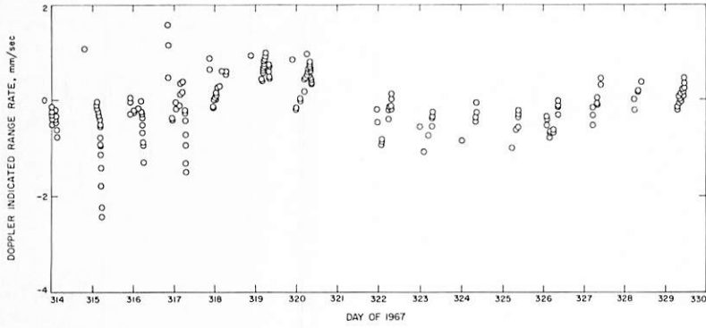
FIGURE 10-5. — Surveyor VI, DSS 11 (Goldstone, Calif.). First lunar day, O - C residual set (compressed five data points/min). DE 19/LE 4 was used.
