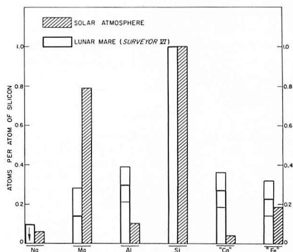
FIGURE 7-16.— Comparison of the observed chemical composition of the Surveyor VI lunar sample with that of the nonvolatile elements in the solar atmosphere. The two compositions have been normalized to unity of silicon. The solar values are from ref. 7-10.
