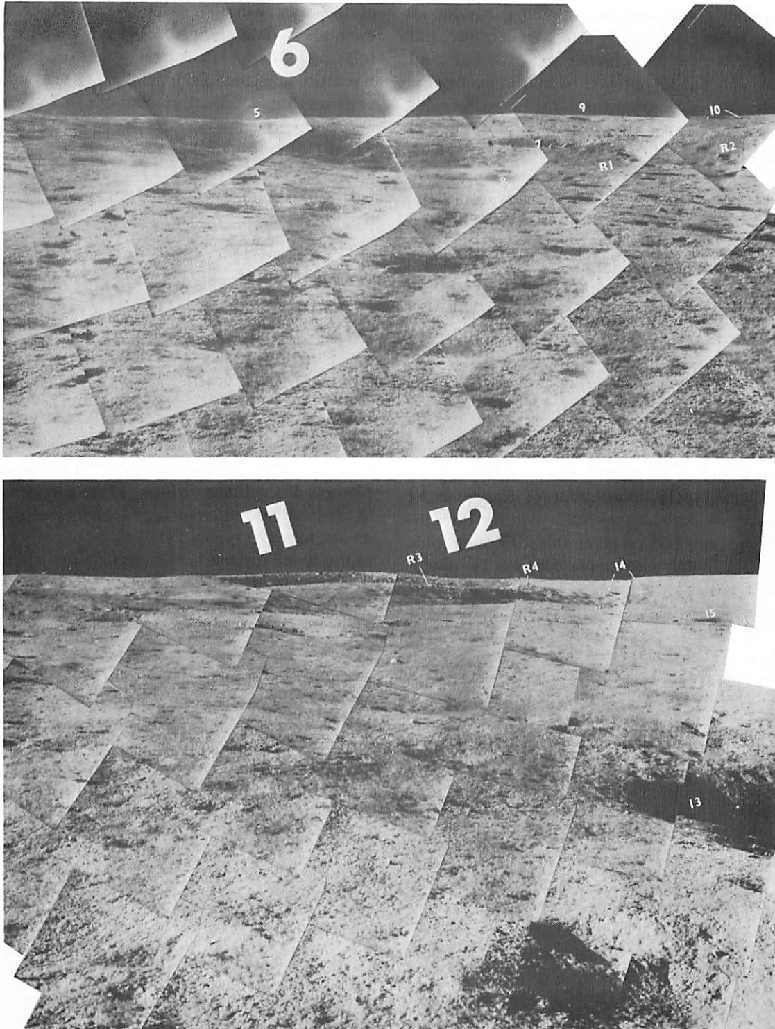
FIGURE 3-5.—Mosaic of Surveyor VI pictures of a mare ridge southeast of the spacecraft. The numbered features were correlated with features on Lunar Orbiter photographs to accurately locate the Surveyor VI spacecraft in the Lunar Orbiter photographs (day 315, 01:32:20 to 01:49:32 GMT).
