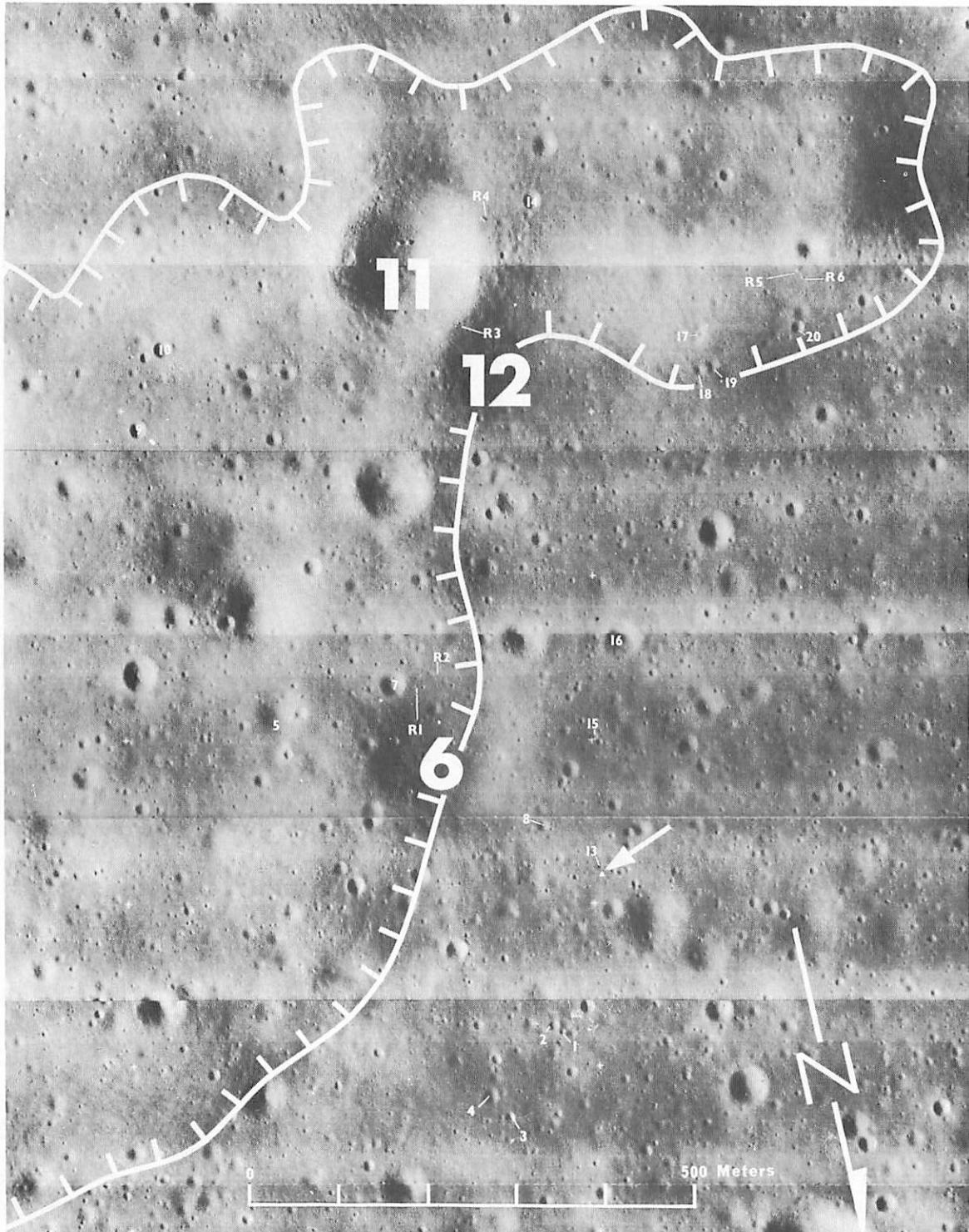
FIGURE 3-6. — Lunar Orbiter II photograph H121 of the Surveyor VI landing site. The numbered features correspond to the numbered features on the mosaic of Surveyor VI pictures (fig. 3-5). These features were used to locate Surveyor VI on the Lunar Orbiter photographs.
