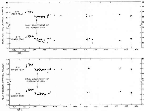
FIGURE 7-2. — Calibration-pulsar peak positions versus time, showing the long-term stability of the Surveyor VI instrument. The data are shown for one alpha and one proton detector; the remaining detector systems behaved similarly.
