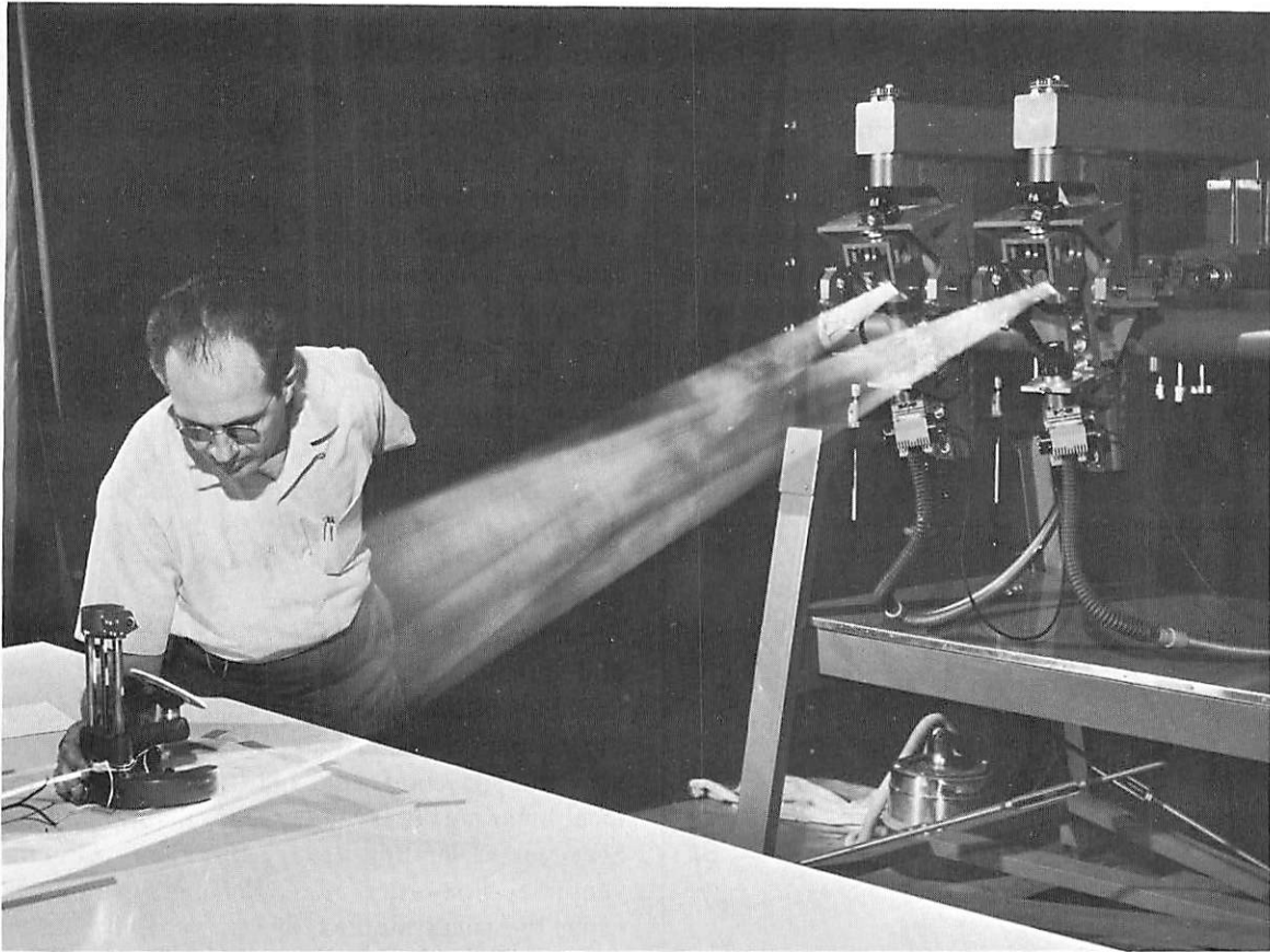
FIGURE 3-8. — The Surveyor anaglyphic stereoplotter. This instrument was originally designed to rectify monoscopic Surveyor pictures, but has been modified for use as a stereoplotter. Each projector is a geometric analog of the television camera. Glass transparencies, or "diapositives," made from stereoscopic pairs of pictures are used at each camera position. The projectors and projector mirrors are set in the same relative orientations as the camera at the time each picture is taken. One picture is projected with red light; the other is projected with blue light. The overlapping images are viewed on a small movable screen, or platen, in the center of which is a pinpoint of light. The operator wears spectacles with one red lens and one blue lens, enabling him to see the overlapping images as a single three-dimensional picture or model. As the platen is moved vertically or horizontally, the point of light at its center appears to float in the stereoscopic model. The horizontal position of the point of light is plotted on the map manuscript over which the platen carriage, or tracing table, moves. The vertical position of the point of light can be read from a counter on the tracing table.
