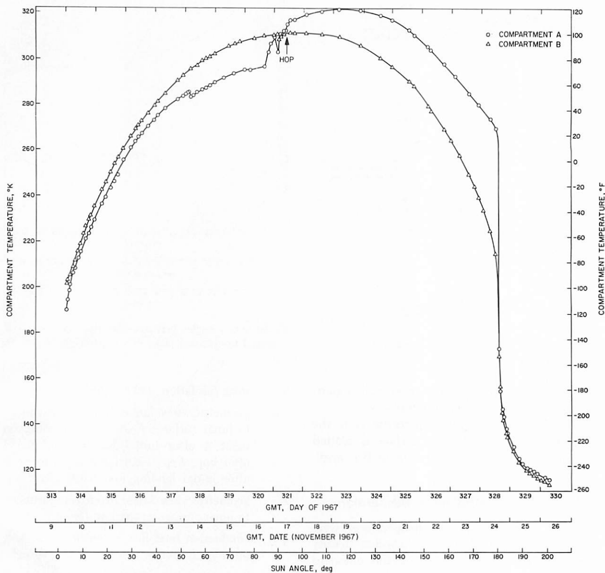
FIGURE 5-7. — Temperatures of outboard face of compartments A and B.
