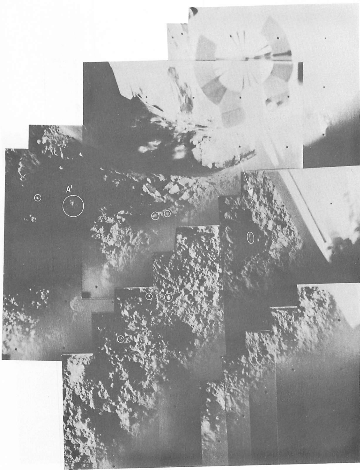
FIGURE 4-53. — Mosaic of pictures taken just after the 4-second firing of the attitude control jets. Representative fragments that arrived at their present sites because of the firing are circled (day 315, Catalog 6-MP-2).
