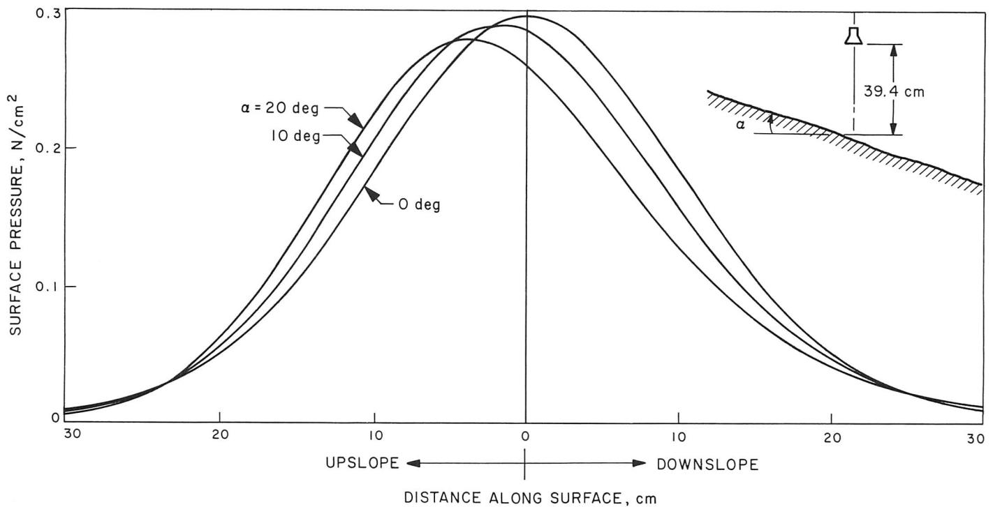
Fig. IV-47. Theoretical static pressure at the surface of planes tilted 0, 10, and 20 deg to the engine nozzle exit plane; engine thrust = 120 N; nozzle height = 39.4 cm.
