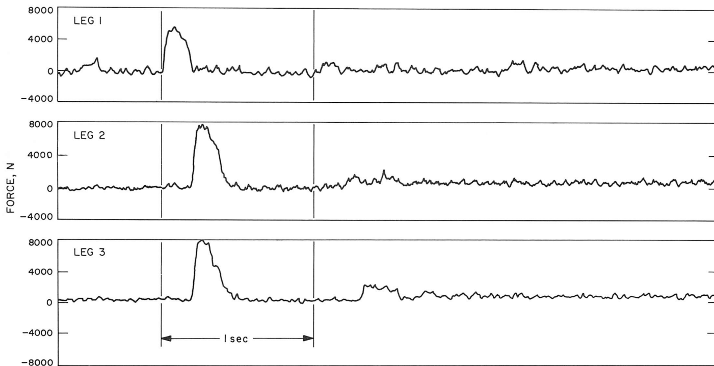
Fig. IV-2. Strain-gage telemetry data showing shock-absorber axial load histories during landing of Surveyor V.
