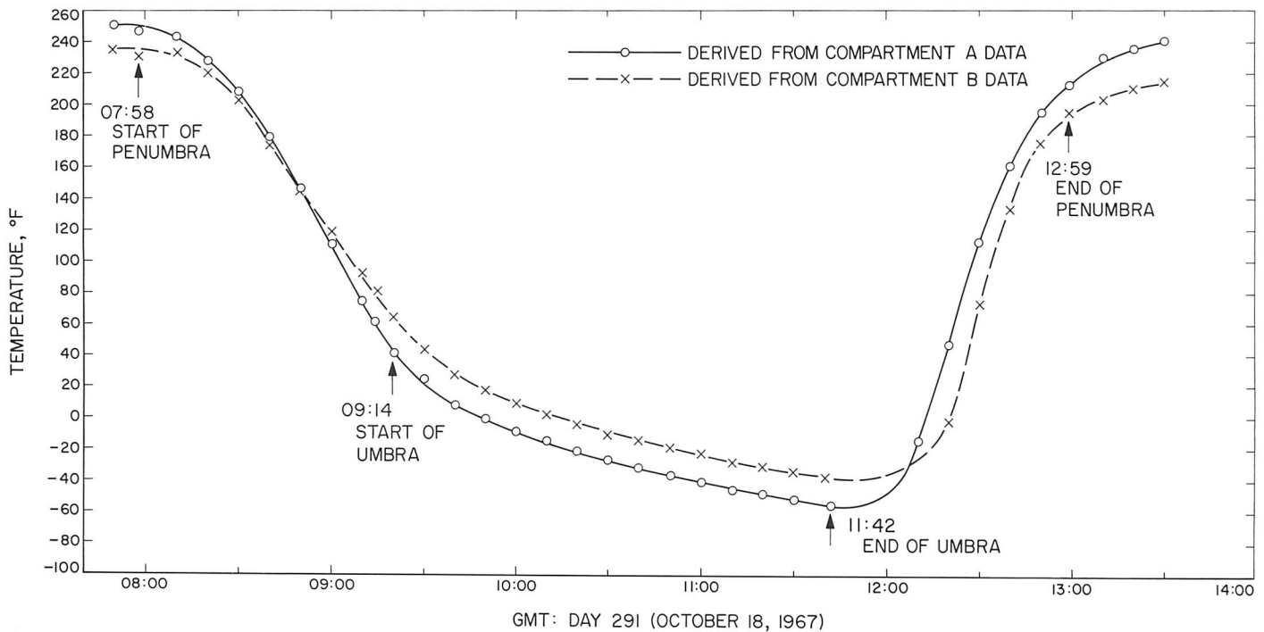
Fig. V-24. Lunar surface brightness temperatures during eclipse.
