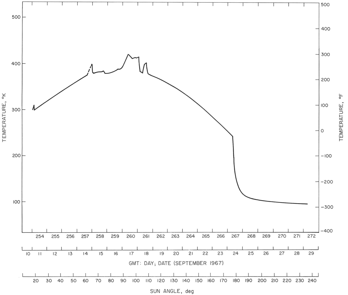
Fig. V-15. Temperature of planar array antenna during first lunar day.
