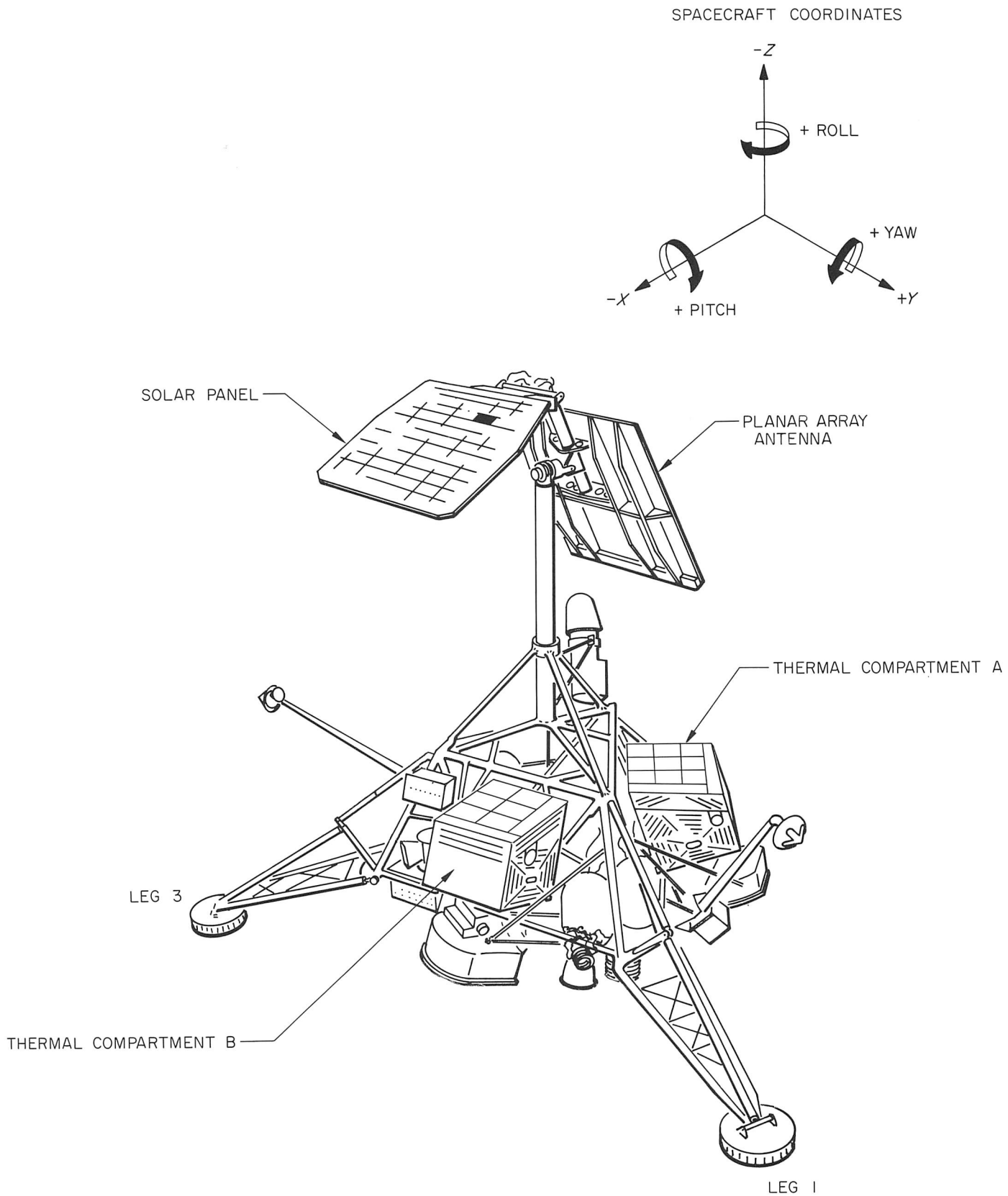
Fig. V-7. Surveyor spacecraft configuration.
