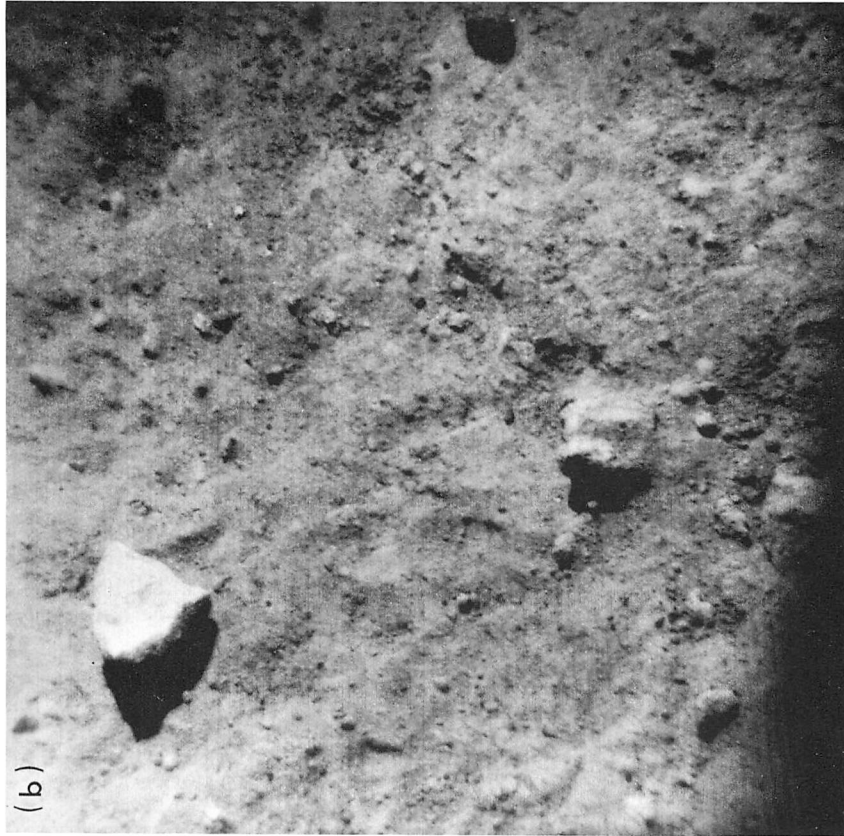
Fig. III-17. A small area on the lunar surface about 2 m from the spacecraft, in which loose fragments moved during the firing of the vernier engines. (a) Picture taken approximately 24 hr before firing of the vernier engines. A fragment approximately 3 cm wide was disturbed by Surveyor V during landing and rolled and bounced across the lunar surface, leaving a track which can be seen near the center of the picture (Day 255, 06:07:26 GMT). (b) Picture of the same area approximately 24 hr after firing of the vernier engines. A comparison with (a) shows that, while some of the larger fragments and lumps have not moved, most of the finer fragments have shifted positions (Day 257, 08:21:19 GMT).
