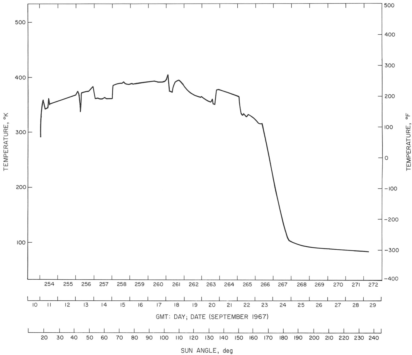
Fig. V-14. Temperature of solar panel during first lunar day.
