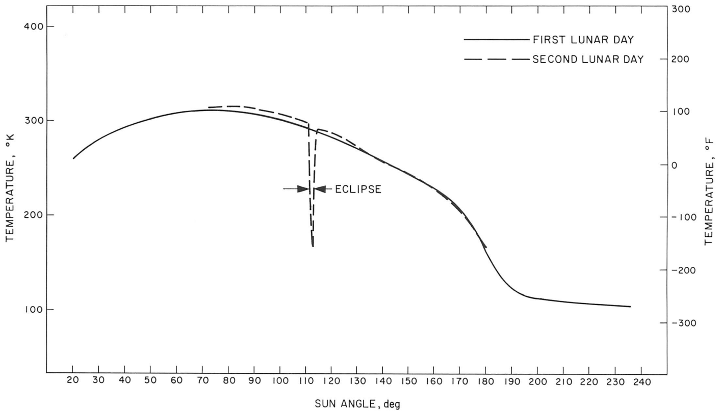
Fig. V-10. Temperatures of outboard face of compartment A during first and second lunar days.
