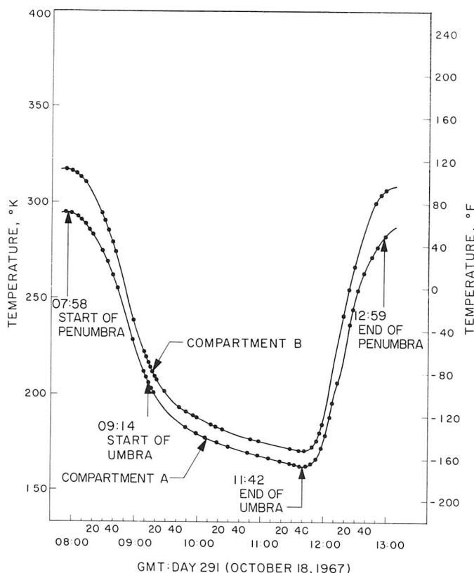
Fig. V-12. Temperatures of outboard faces of compartments A and B during eclipse.
