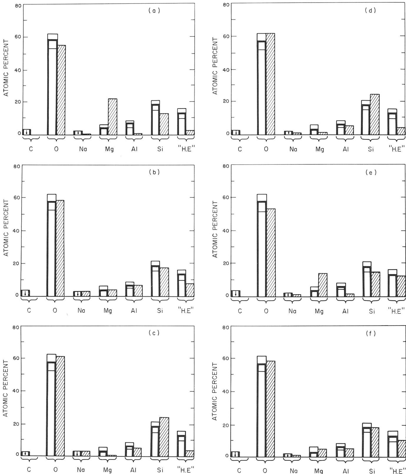
Fig. VII-16. Comparison of the observed chemical composition of the lunar sample (open bars) with the average composition (Ref. VII-6) of selected materials (cross-hatched bars). A, dunite; B, basalts; C, granites; D, tektite (Indo-Malayan body); E, low iron chondritic meteorite; F, basaltic achondrite meteorites. The "H. E." means elements heavier than silicon.
