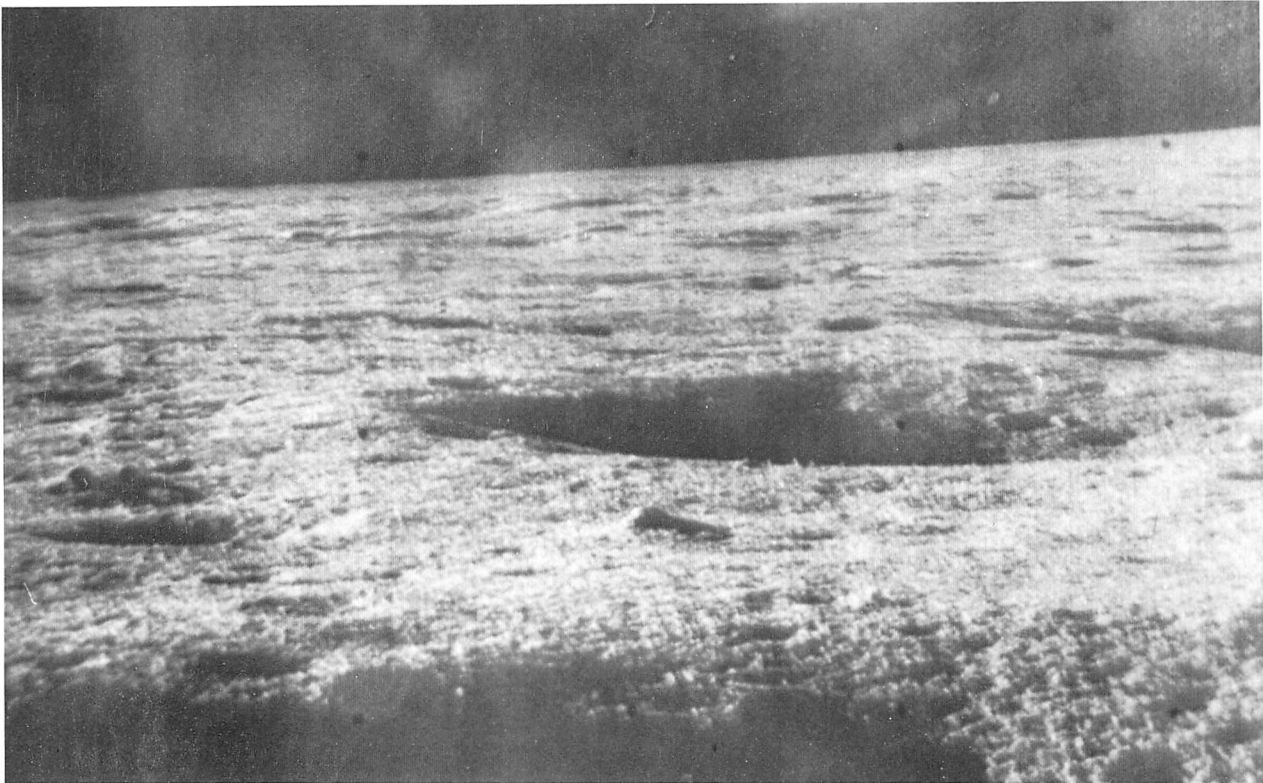
Fig. III-9. Wide-angle picture of the far field and horizon northwest of Surveyor V. The dark area along the bottom of the picture is part of the wall of the Surveyor V crater in shadow. A crater 4 m in diameter lies between the rim of the Surveyor V crater and the horizon. This crater, which is devoid of a raised rim, probably is part of a system of craters aligned in a northwest direction and parallel with one of the major lineation directions in Mare Tranquillitatis (Day 266, 11:27:18 GMT).
