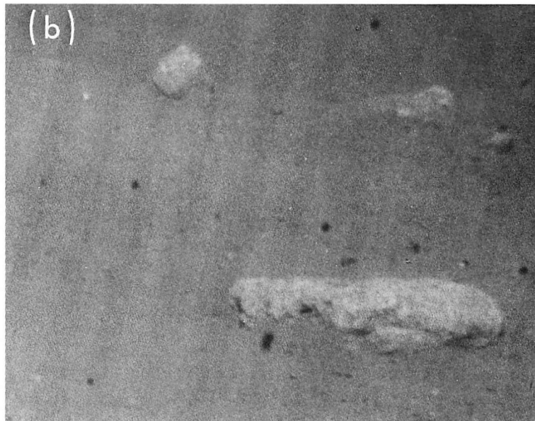
Fig. III-24. Fragments in a strewn field of blocks south of the spacecraft. (a) Subrounded fragments lying 18 to 30 m from Surveyor V television camera. Largest fragment, which casts a small shadow, is 30 to 40 cm across. These are some of the largest fragments in the field of view around Surveyor V (Day 263, 07:38:46 GMT). (b) Mottled, subrounded fragments, largest of which is about 20 cm across, lying 5 to 6 m from Surveyor V television camera. These fragments exhibit bright spots 1 to 2 cm across, similar to those on one of the large rocks observed at the Surveyor I landing site (Day 264, 11:37:01 GMT).
