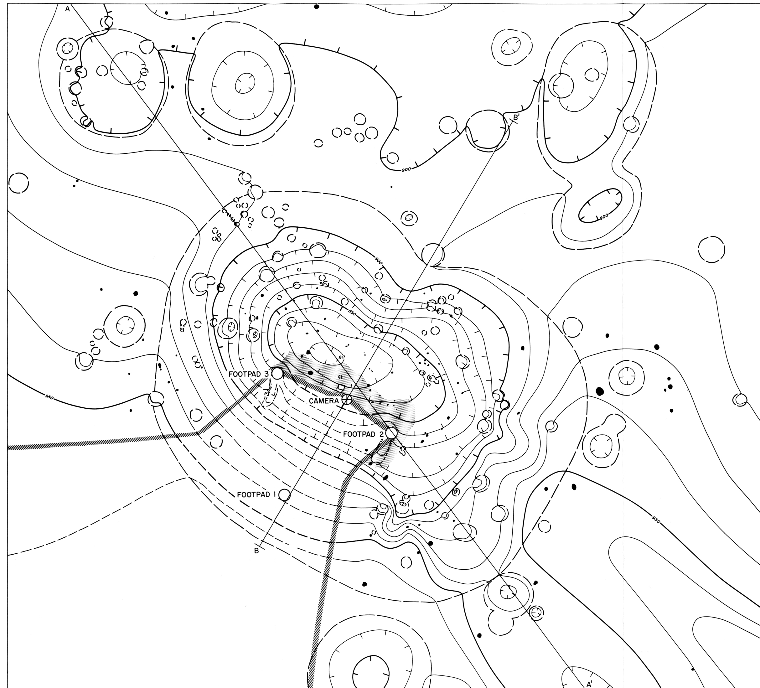
Fig. III-3. Large-scale topographic map of Surveyor V landing site (topography by R. M. Batson, R. Jordan, and K. B. Larson).
