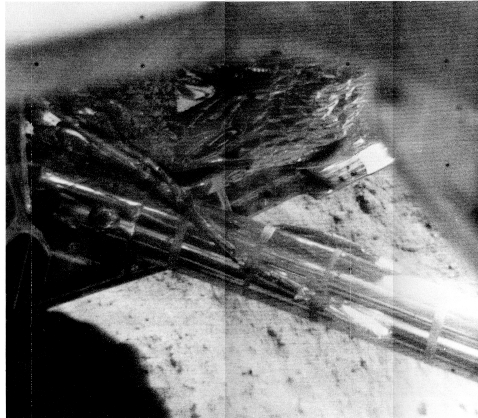
Fig. IV-24. A post-firing view of the only part of the vernier engine 1 impact area that can be seen by the television camera. The rough-textured lunar surface within the small triangular area is probably part of an erosion crater. This area was in shadow before the firing (Day 263, 11:47:05 GMT).
