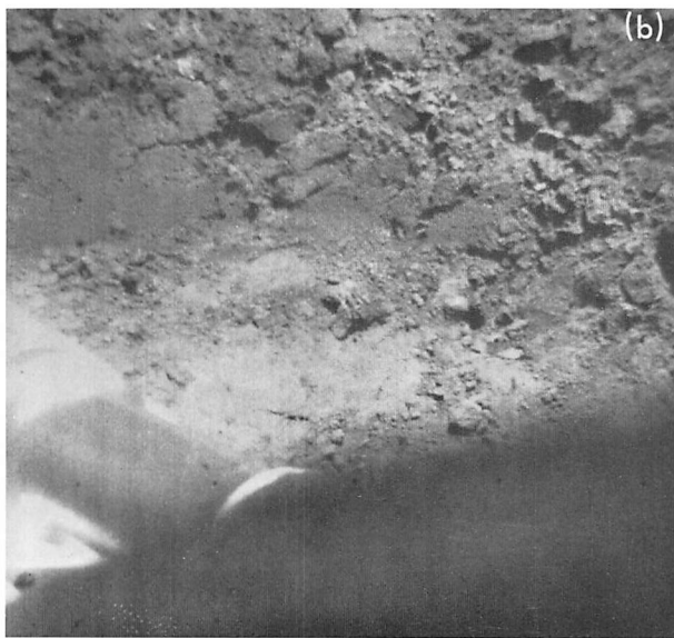
Fig. VIII-19. (a) Laboratory simulation of footpad 2 landing mode in 37–50 \mu Little Lake basalt. Velocity, depth of penetration, and distance were simulated. (b) Picture taken by Surveyor V of the side of trench dug by footpad 2. Note similarity to Fig. VIII-18a and VIII-18c (Day 258, 04:02:17). (c) Closeup of footpad and magnet assembly used in laboratory simulation studies of landing (Fig. VIII-18a). Six such landings were performed; all results were similar. Note material on control bar on the right, material in the honeycomb and clumped on the magnet, covering the attachment screws. The increased humidity in the laboratory may have caused results similar to the apparent vacuum cohesion on the moon.
