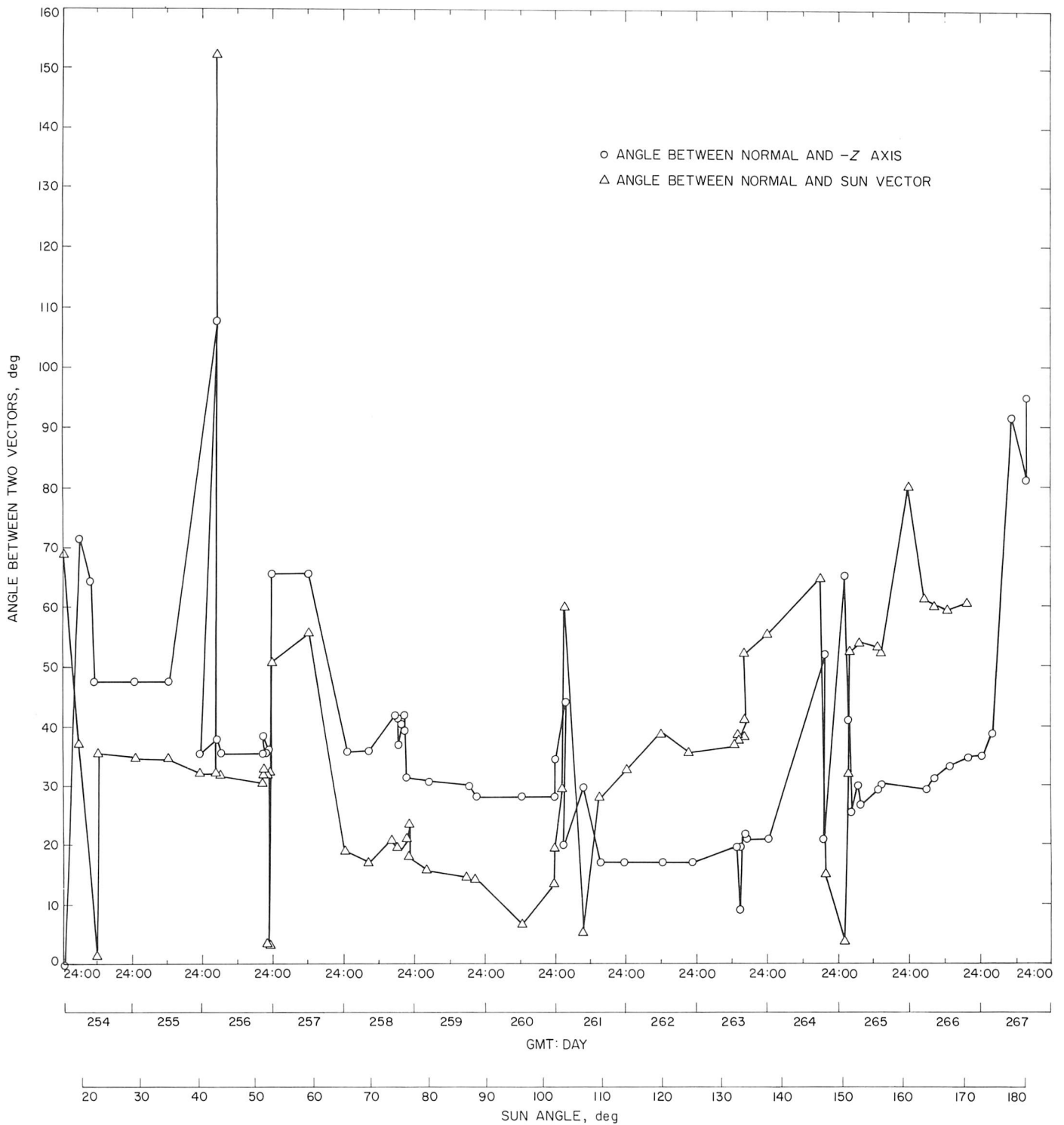
Fig. V-17. Angle that normal to solar panel makes with sun vector and -Z axis during first lunar day.
