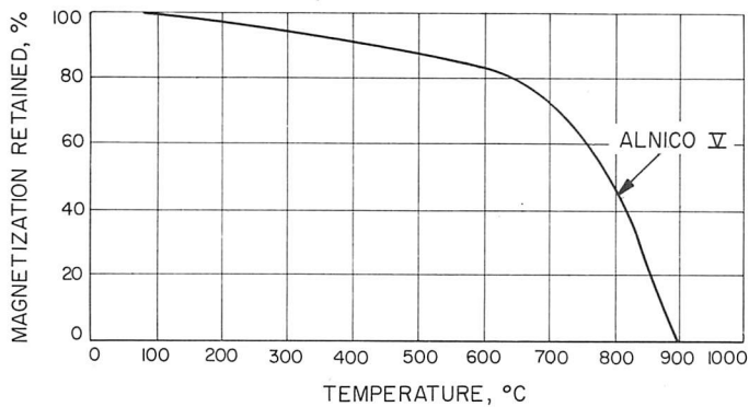
Fig. VIII-6. Magnetic remanence vs temperature for Alnico V. Internal structure and the metallurgical properties of the alloy used control the effect of high temperatures on magnetic materials. Alnico V has retraceable temperature characteristics over a wide range ( -200 to 300^{\circ}\text{C} ). This is one of the properties that dictated its choice for the Surveyor V magnet.
