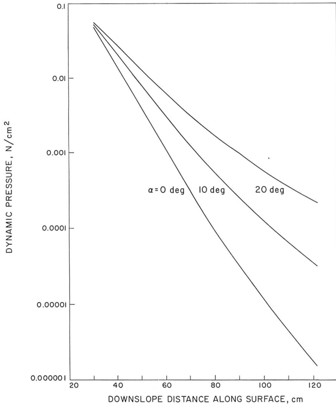
Fig. IV-44. Theoretical dynamic pressure at the surface of planes tilted 0, 10, and 20 deg to the engine nozzle exit plane; engine thrust = 120 N; nozzle height = 39.4 cm. Dynamic pressure over a 30- to 120-cm range from a point directly below the engine.
