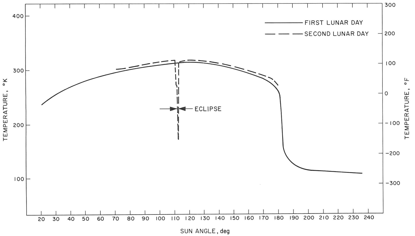
Fig. V-11. Temperatures of outboard face of compartment B during first and second lunar days.
