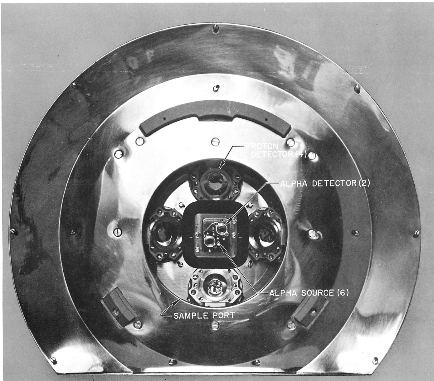
Fig. VII-2. Bottom view of the alpha-scattering sensor head.
