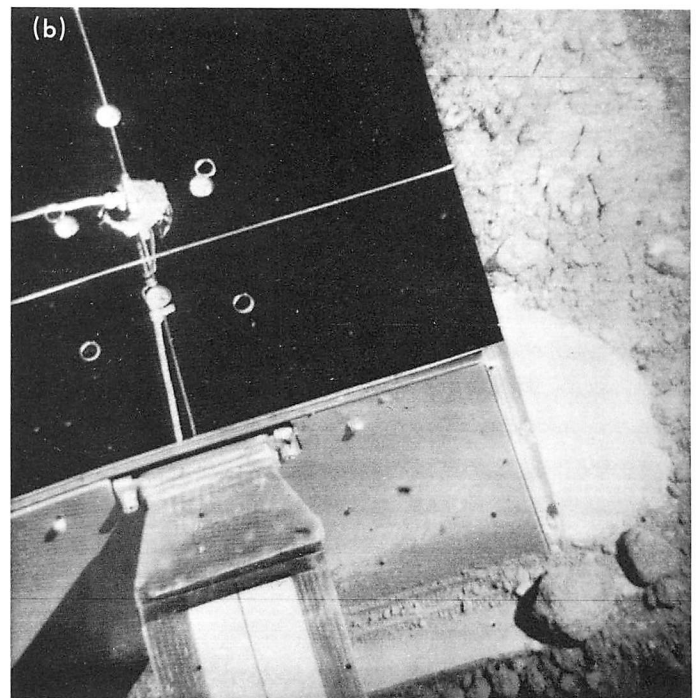
Fig. IV-31. Gold-plated face D (see Figs. IV-27 and IV-28) of the sensor head. (a) Pre-firing picture; face D is highly reflective (Day 255, 05:06:27 GMT). (b) Post-firing picture; face D is nonreflective (Day 257, 07:15:09 GMT).
