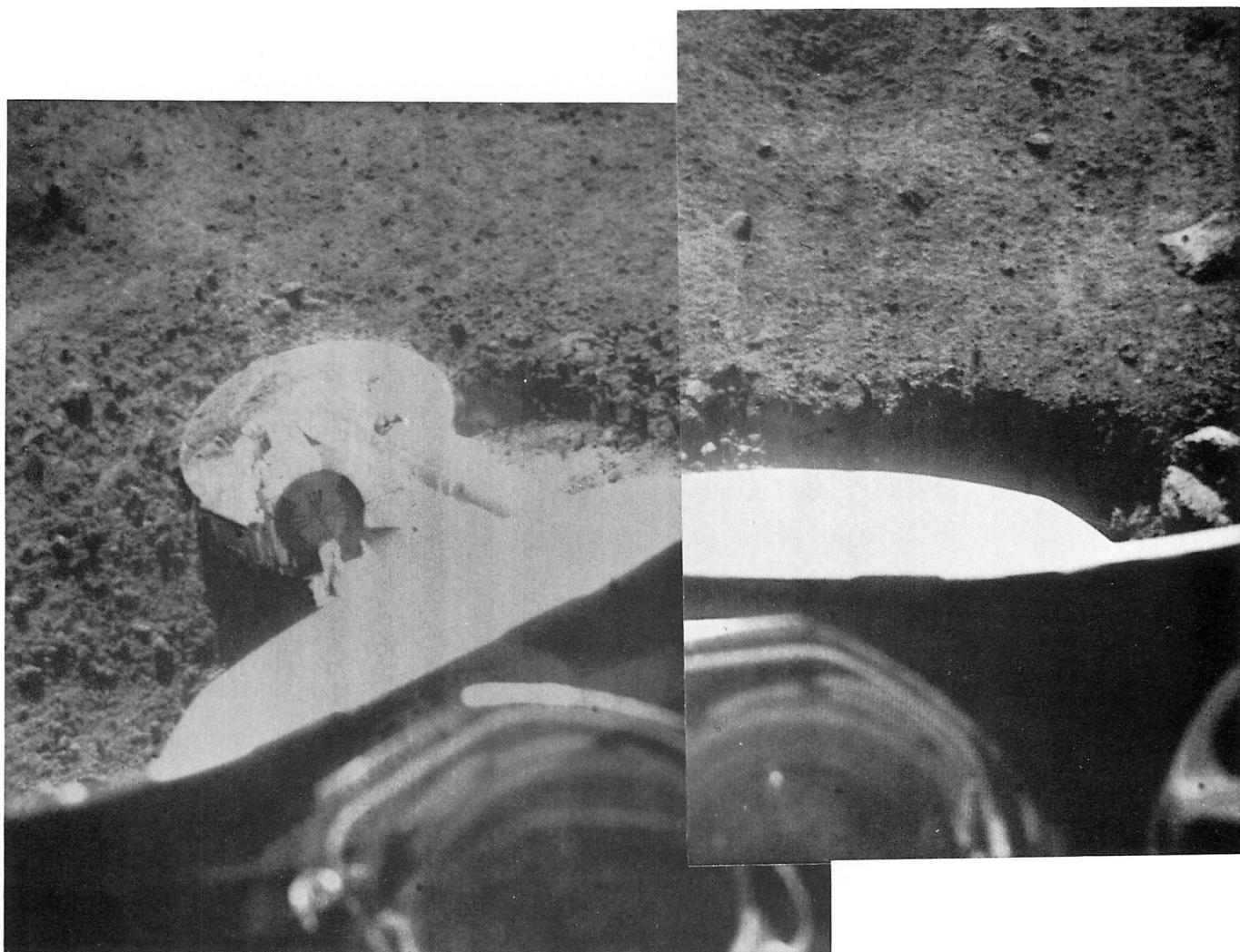
Fig. VIII-7. Landing mode of footpad 2. The spacecraft landed on a 19.5\text{-deg} , inner slope of a 9\text{-} \times 12\text{-m} crater, causing footpad 2 to slide downhill a distance of about 1\text{ m} at a depth of 3 to 10\text{ cm} through the lunar surface material. Note material on top of the footpad; also note well-defined footpad imprint at the end of the slide and the scalloped effect in part of the trench. This is indicative of the slight bouncing of the footpad in sliding. Velocity during downhill trenching is estimated at 1\text{ m sec}^{-1} (Day 255, 00:18:35 and Day 254, 23:29:23).
