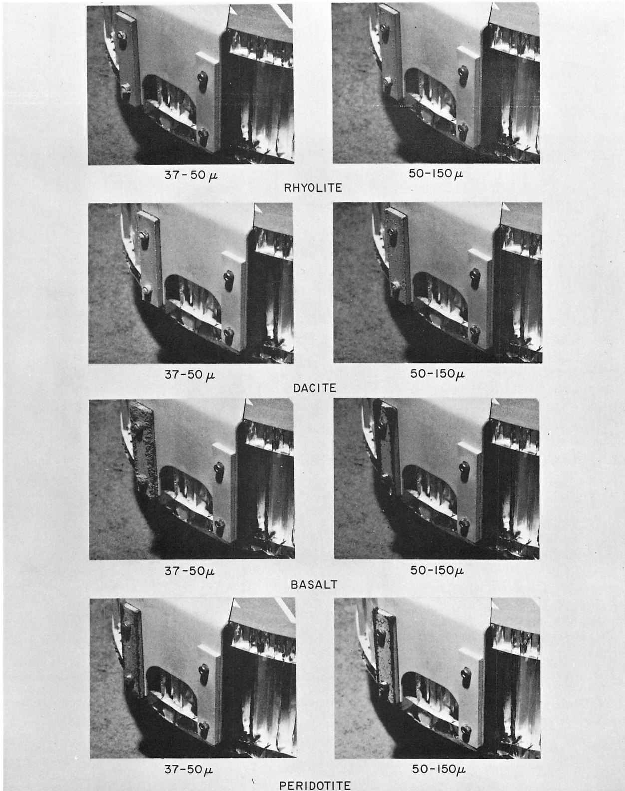
Fig. VIII-13. Results of impact in atmosphere in rock types ranging from acidic (high silica content) rhyolite to basic (low silica content) peridotite. Two powder sizes were used: 37-50 \mu and 50-150 \mu . Note appearance of basalt powders.
