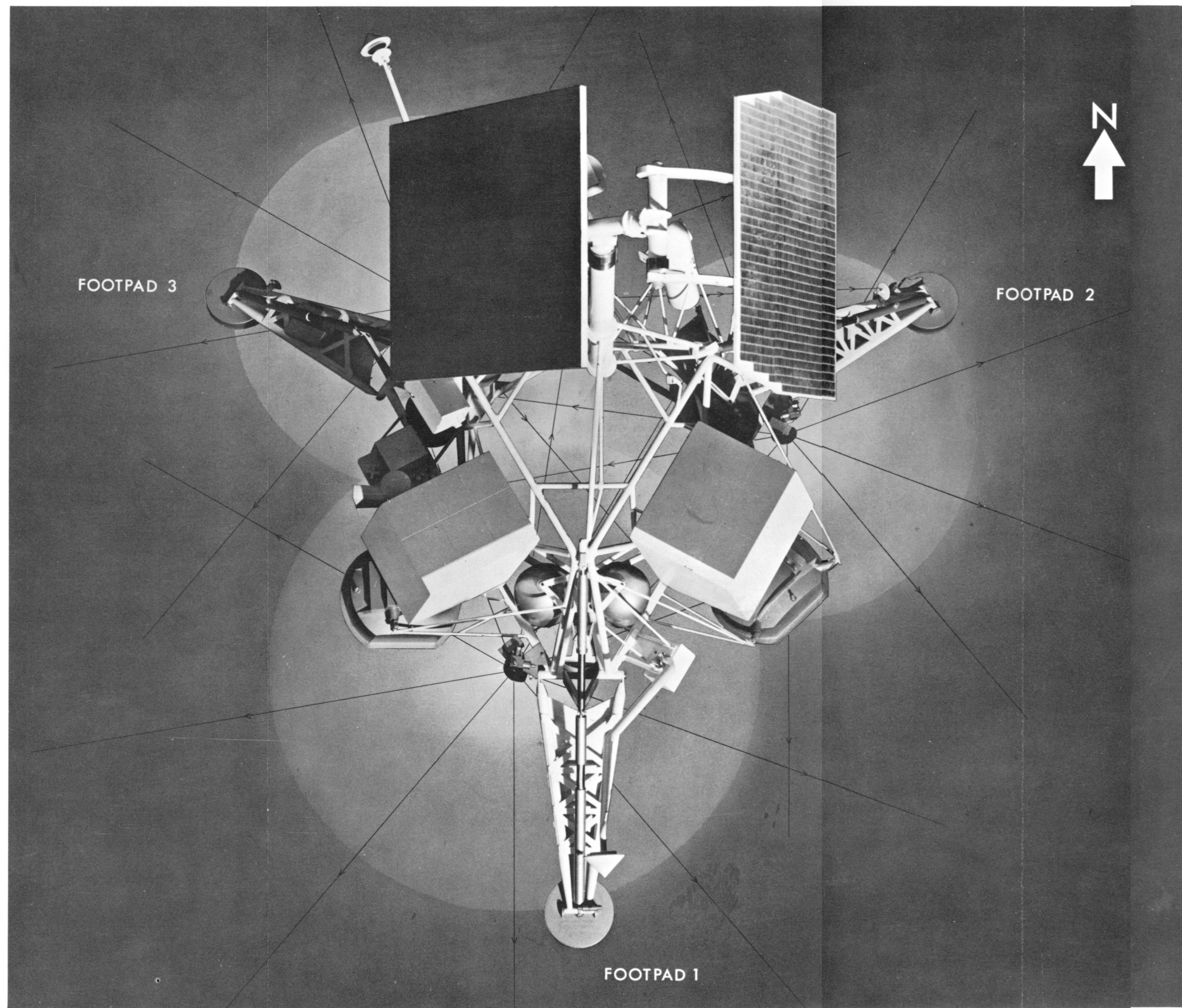
Fig. VIII-10. Vernier exhaust vectors relative to the magnet assembly. The light circles represent 1.1 m from verniers at which distance the dynamic pressure was approximately 1 \text{ dyne cm}^{-2} . The gas dispersion curve becomes asymptotic at about 2.44 m from the vernier engines. Left: view is looking down on the spacecraft, located on a 19.5-deg slope. North is to the top, footpad 2 is top right. Right: view looking east, showing the vernier exhaust vector relationships. The main vectors are lateral, the top of the footpads probably near the height limit for the main vectors.
