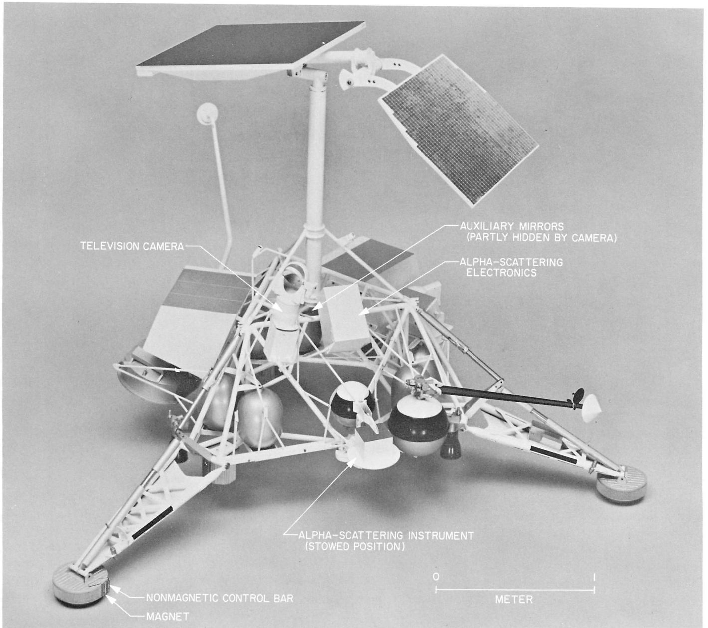
Fig. I-1. Model of Surveyor V spacecraft in landed configuration.
