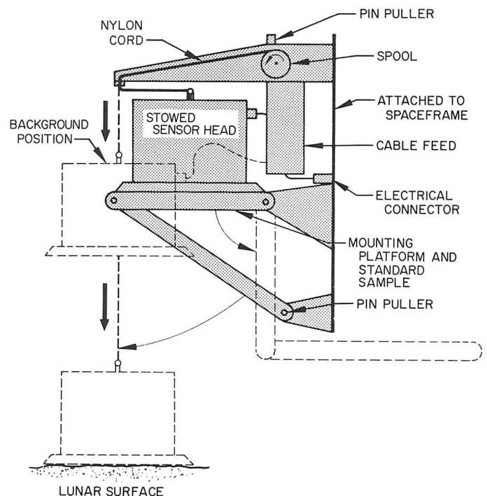
Fig. VII-4. Operation of the alpha-scattering deployment mechanism.
