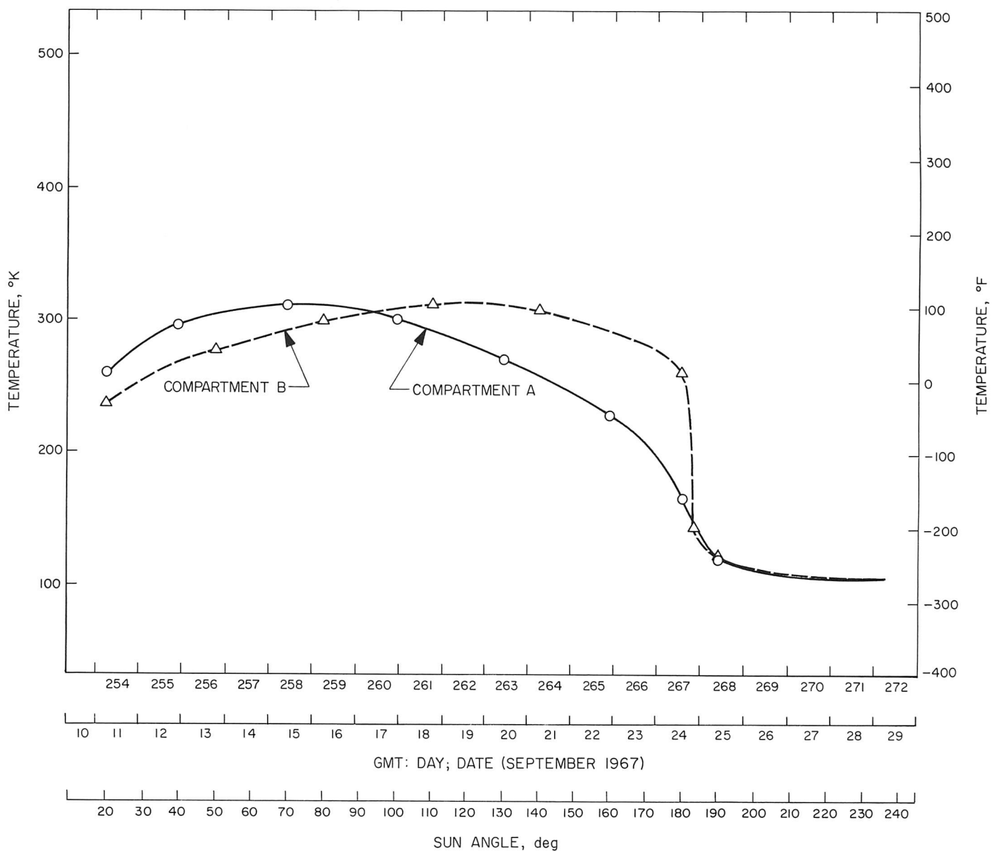
Fig. V-8. Temperatures of outboard faces of compartments A and B during first lunar day.
