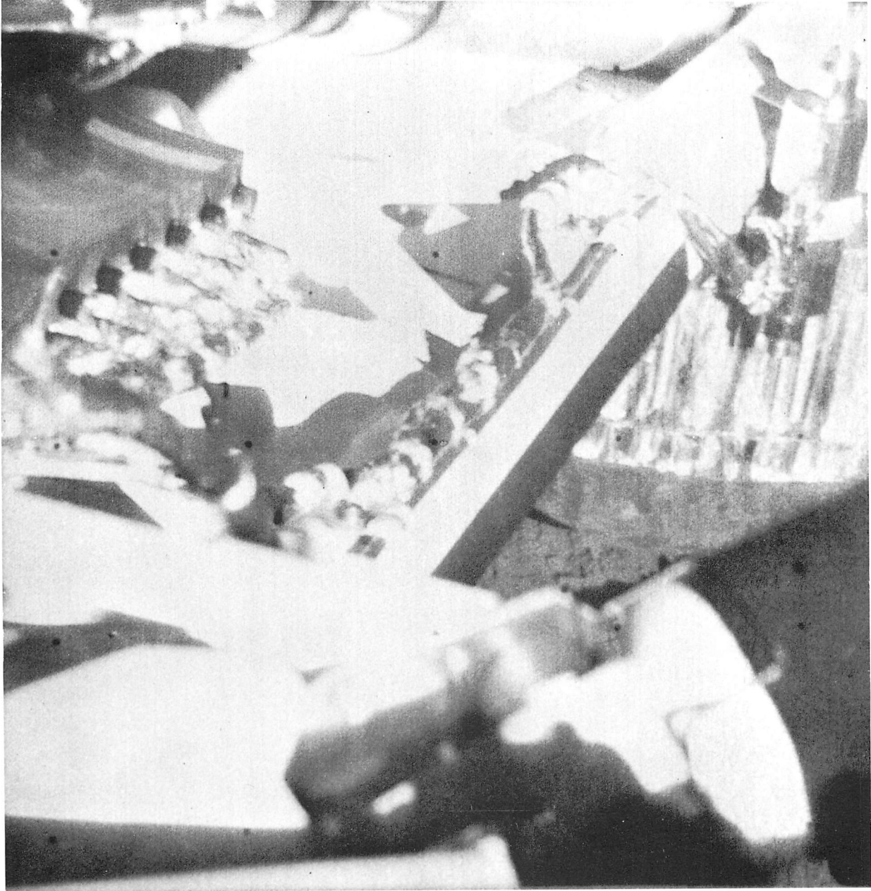
Fig. IV-13. Narrow-angle picture of the inboard section of footpad 3. The tilted footpad and the footpad imprint can be seen (Day 255, 02:09:40 GMT).
