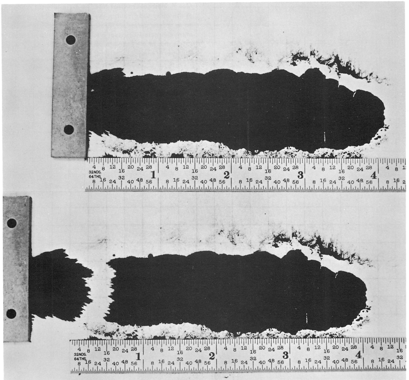
Fig. VIII-5. Distance from which magnet on Surveyor V will attract powdered iron on earth is shown by placing the magnet adjacent to powdered iron (above) and displacing the bar to the left (below). The magnet collected iron from a distance of 1.93 cm.
