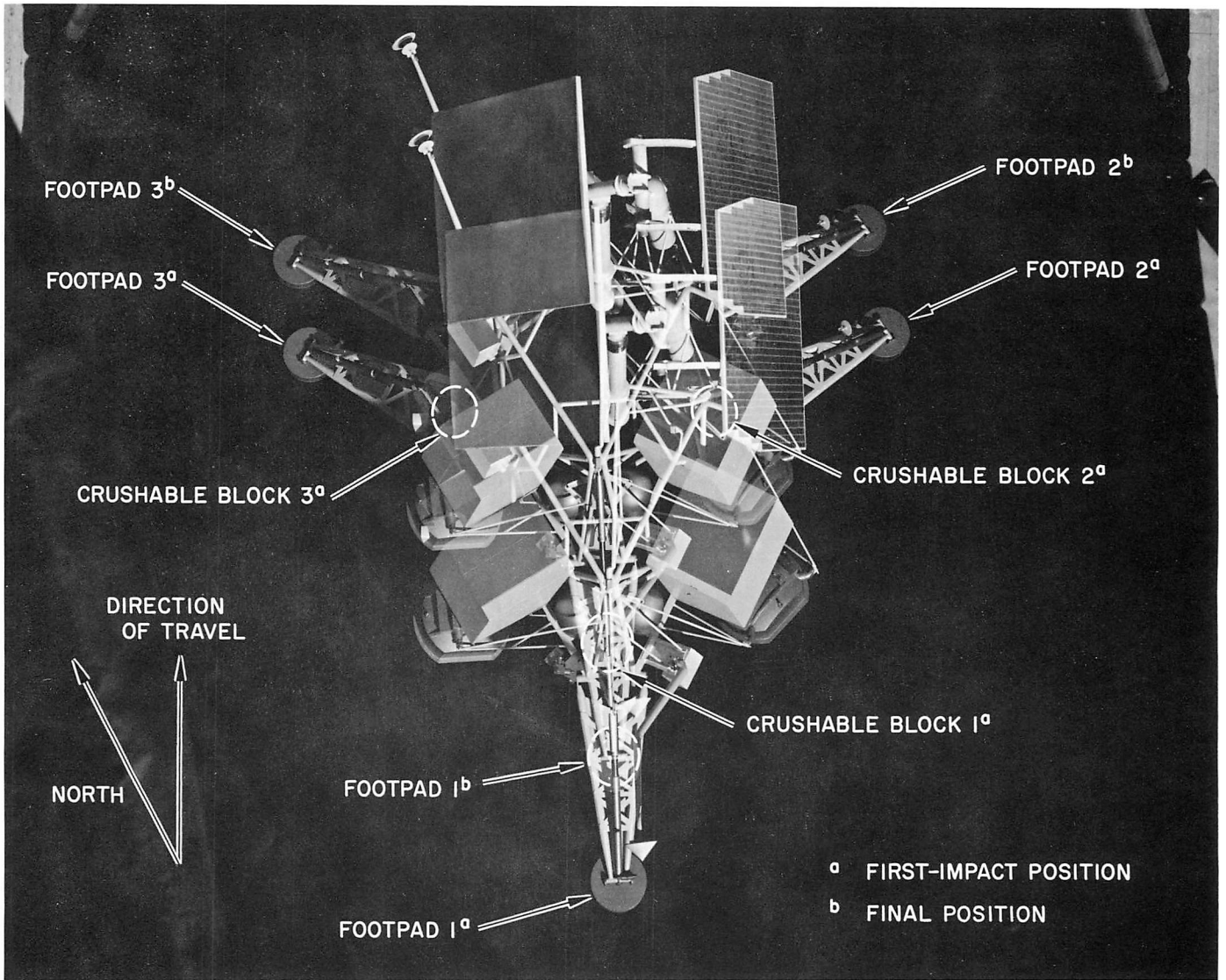
Fig. IV-4. Spacecraft motion during landing. (a) Probable spacecraft position at time of first landing impact. (b) Final position after the spacecraft had come to rest.
