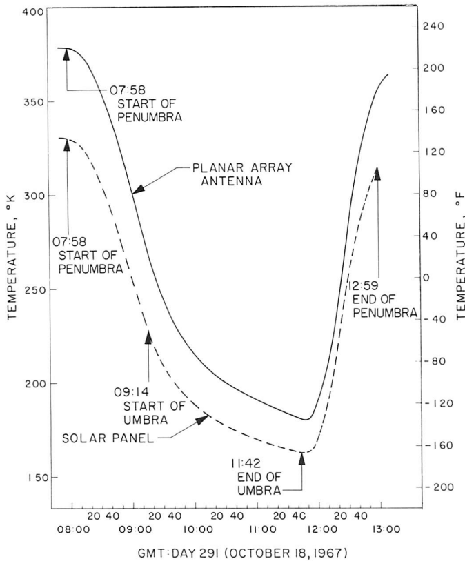
Fig. V-16. Temperatures of solar panel and planar array antenna during eclipse.
