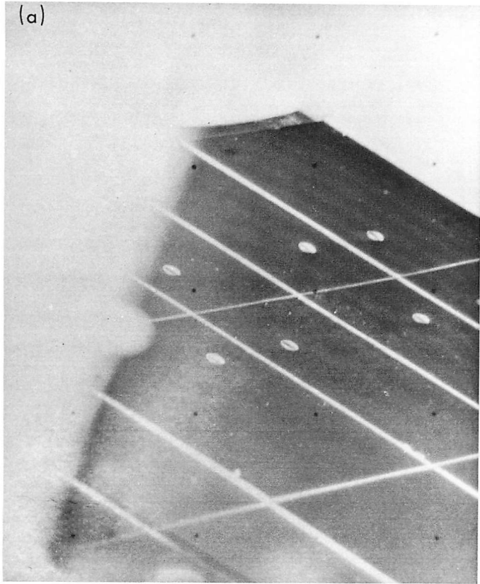
Fig. IV-39. Top of compartment B taken before and after the firing. A lump of material was transported to the compartment top and splattered in a direction away from vernier engine 1. (a) Day 255, 02:29:29 GMT. (b) Day 265, 05:48:58 GMT.
