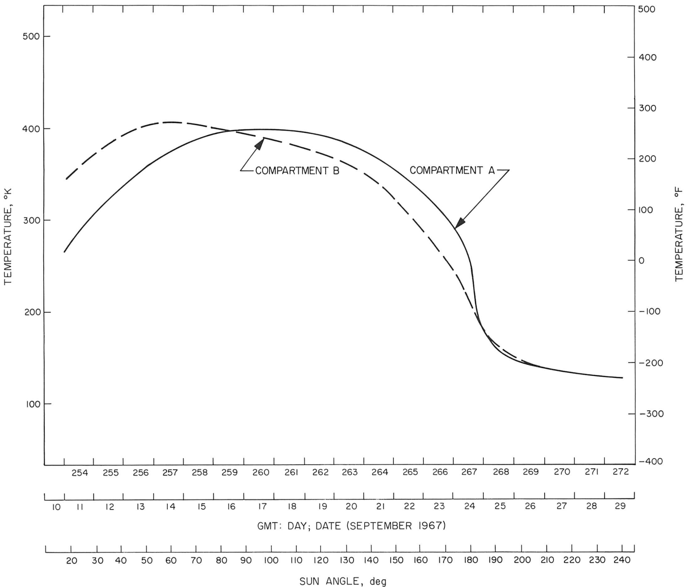
Fig. V-19. Lunar surface temperatures during first lunar day, as calculated from telemetry data for compartments A and B.
