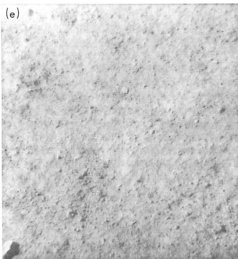
Fig. III-28. Areas on the lunar surface near Surveyor V in which size-frequency distribution of fragments was measured. The location of these areas is shown in Fig. III-10. (a) Area V-B: on the floor of the Surveyor V crater. Smallest fragments resolved are about 1 mm across, and the largest fragments are about 4 to 5 cm across (Day 265, 12:15:52 GMT). (b) Area V-D: on the wall of the Surveyor V crater approximately 2.5 m from the spacecraft. Smallest fragments resolved are about 2 mm; the largest fragment is about 3 cm across (Day 257, 07:08:23 GMT). (c) Area V-E: on the wall of the Surveyor V crater about 2.4 m from the spacecraft. Smallest fragments resolved are about 1 mm, and the largest fragments are about 6 to 8 mm (Day 257, 07:08:44 GMT). (d) Area V-F: on the wall of the Surveyor V crater about 3 m from the spacecraft. Smallest fragments resolved are about 1 mm, and the largest fragments are about 1 cm (Day 257, 07:10:20 GMT). (e) Area V-G: on the wall of the Surveyor V crater about 3 m from the spacecraft. Smallest fragments resolved are about 2 mm, and the largest fragments are about 1 cm across (Day 264, 12:14:09 GMT). (f) Mosaic of narrow-angle pictures showing area V-H on the wall of the Surveyor V crater approximately 2 to 4 m from the spacecraft. Smallest fragments resolved are about 4 mm across, and the largest fragment is about 10 cm across (Day 257, 07:18:30 to 07:21:58 GMT).
