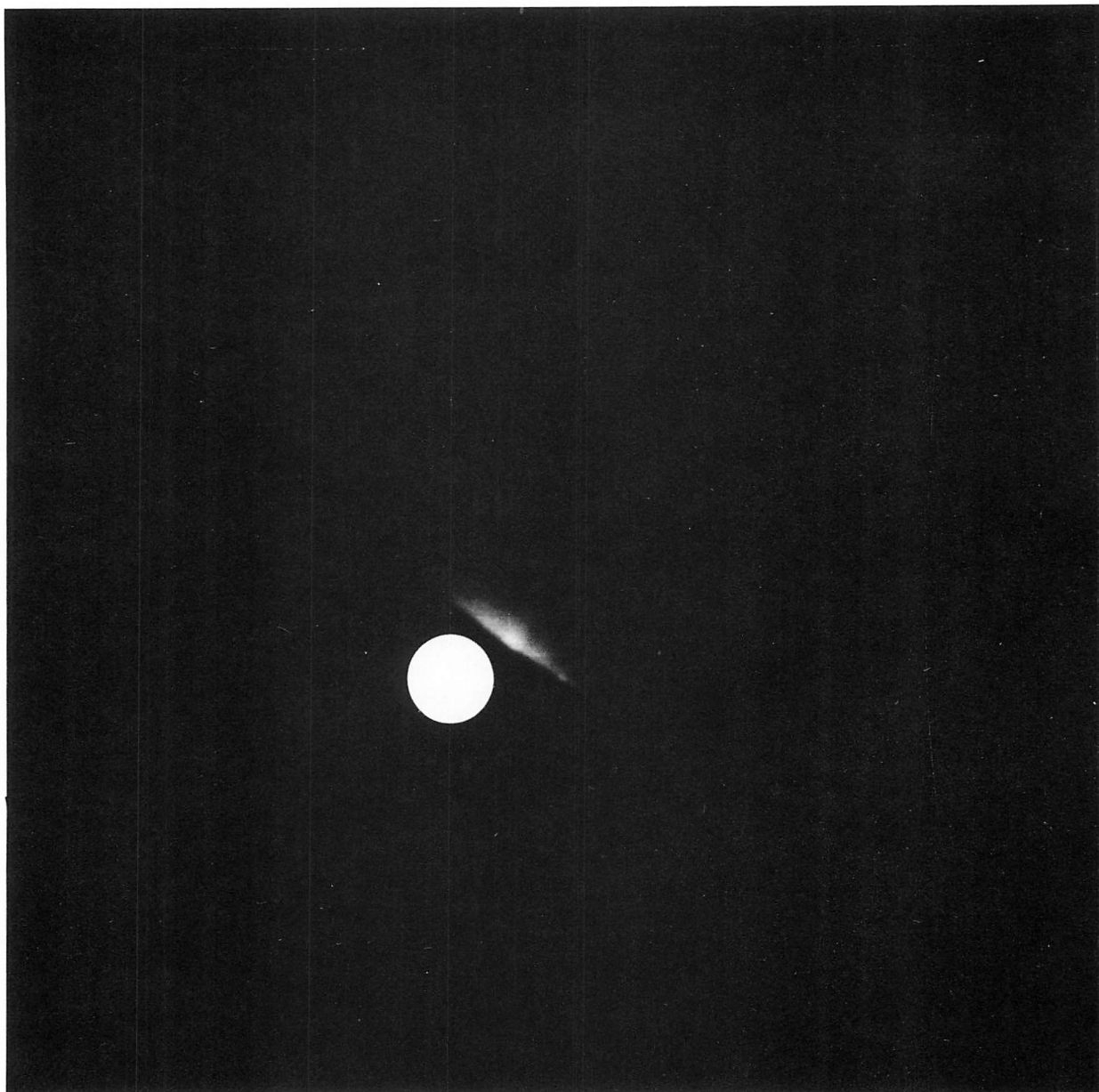
Fig. VI-1. Picture of the K-corona; a 30-sec exposure at f/22 . The upper solar limb is approximately 0.5 solar radius below the horizon. Several coronal streamers are visible. The K-corona in this picture is produced by scattering from electrons near the sun. The white circle denotes the relative size and location of the sun (Day 267, 11:08:32 GMT).
