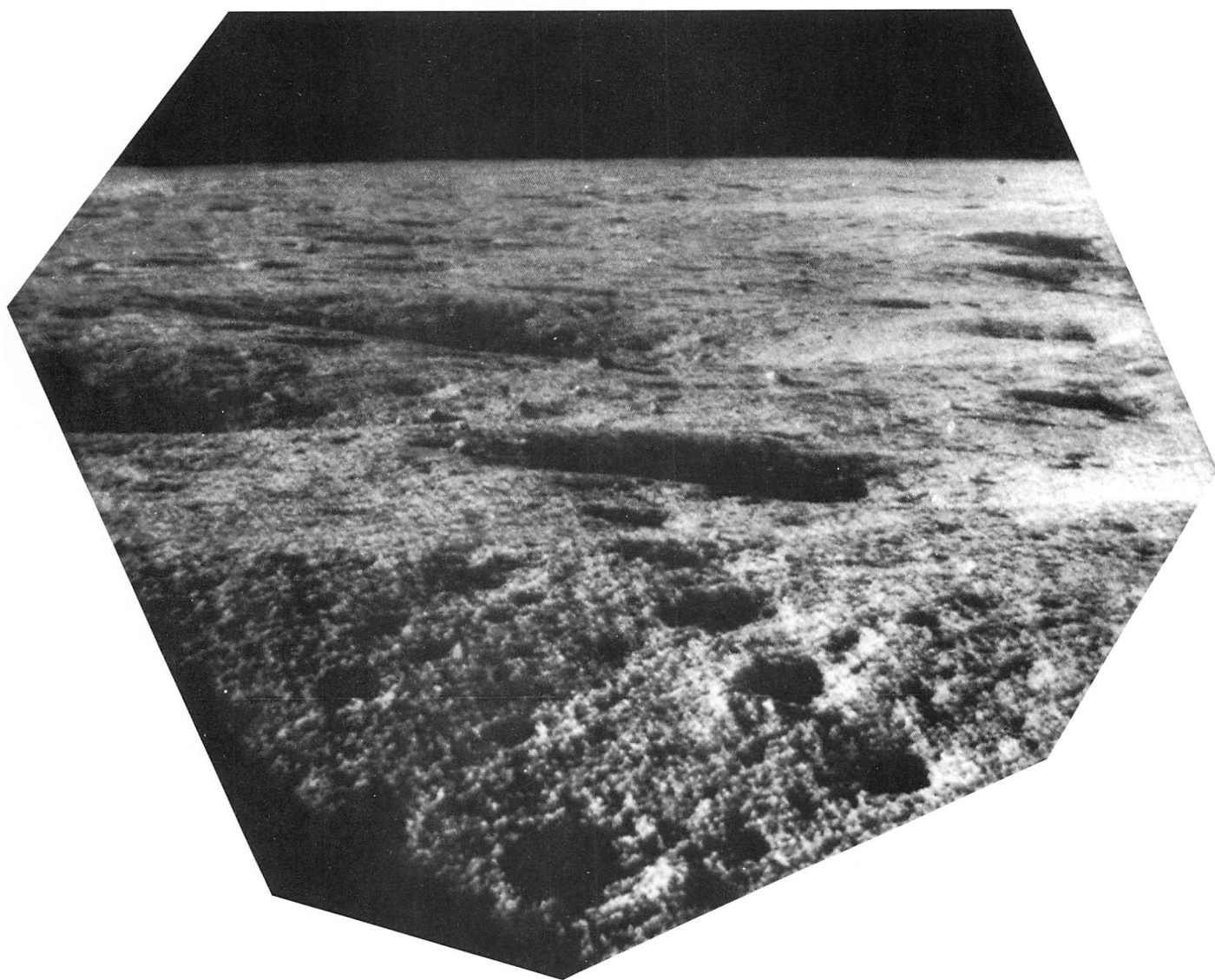
Fig. III-8. Wide-angle picture of the northwest wall of the Surveyor V crater. Chain of small craters 20 to 40 cm in diameter extends from the center to the bottom of the picture (Day 266, 11:26:28 GMT).
