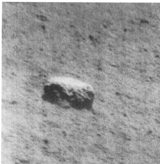
Fig. III-22. Angular block 11 cm in diameter on the east rim of the Surveyor V crater. The nearly level, upper surface of this block is much brighter at large phase angles than the surrounding fine-grained debris (Day 258, 08:44:16 GMT).
