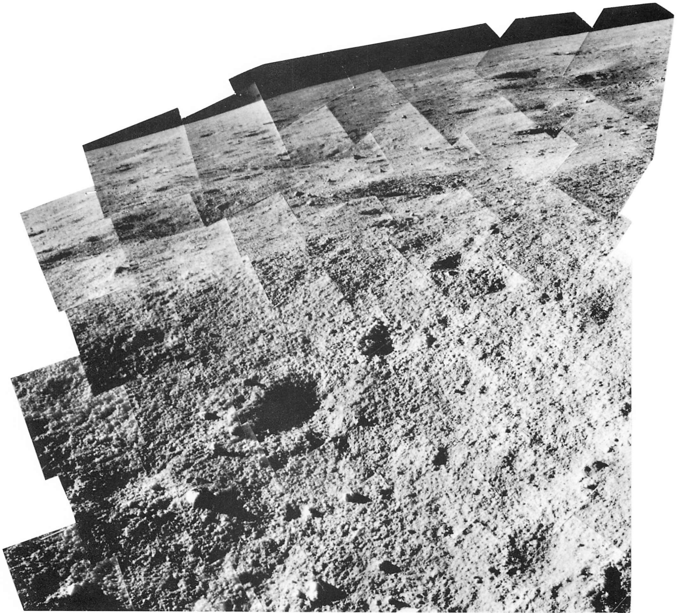
Fig. III-6. Mosaic of narrow-angle pictures from Surveyor V showing the northwest wall of the Surveyor V crater, and the far field beyond the rim of the crater extending to the horizon. Differences in texture of the crater wall and the far field are due to differences in the distance from the camera and inclination of the surfaces (Day 275, 15:12:50 to 16:11:20 GMT).
