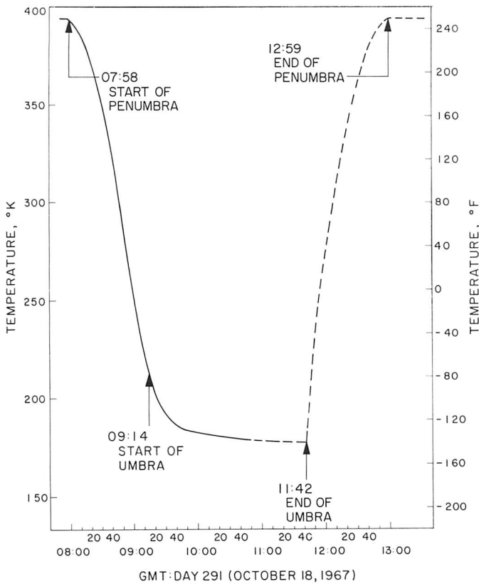
Fig. V-4. Predicted lunar surface temperatures during eclipse (data from December 19, 1964, eclipse adjusted in time for October 18, 1967, eclipse).
