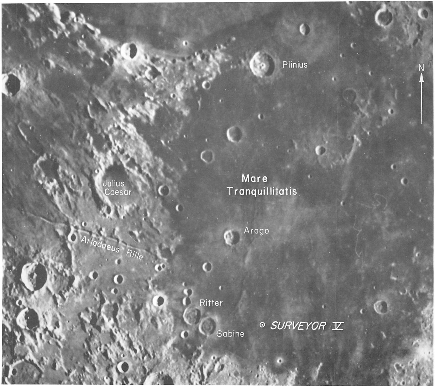
Fig. III-2. Earth-based telescopic photograph of Mare Tranquillitatis and the highlands to the west. Prominent northwest-trending ridges and valleys in the highlands are part of Imbrian sculpture.
