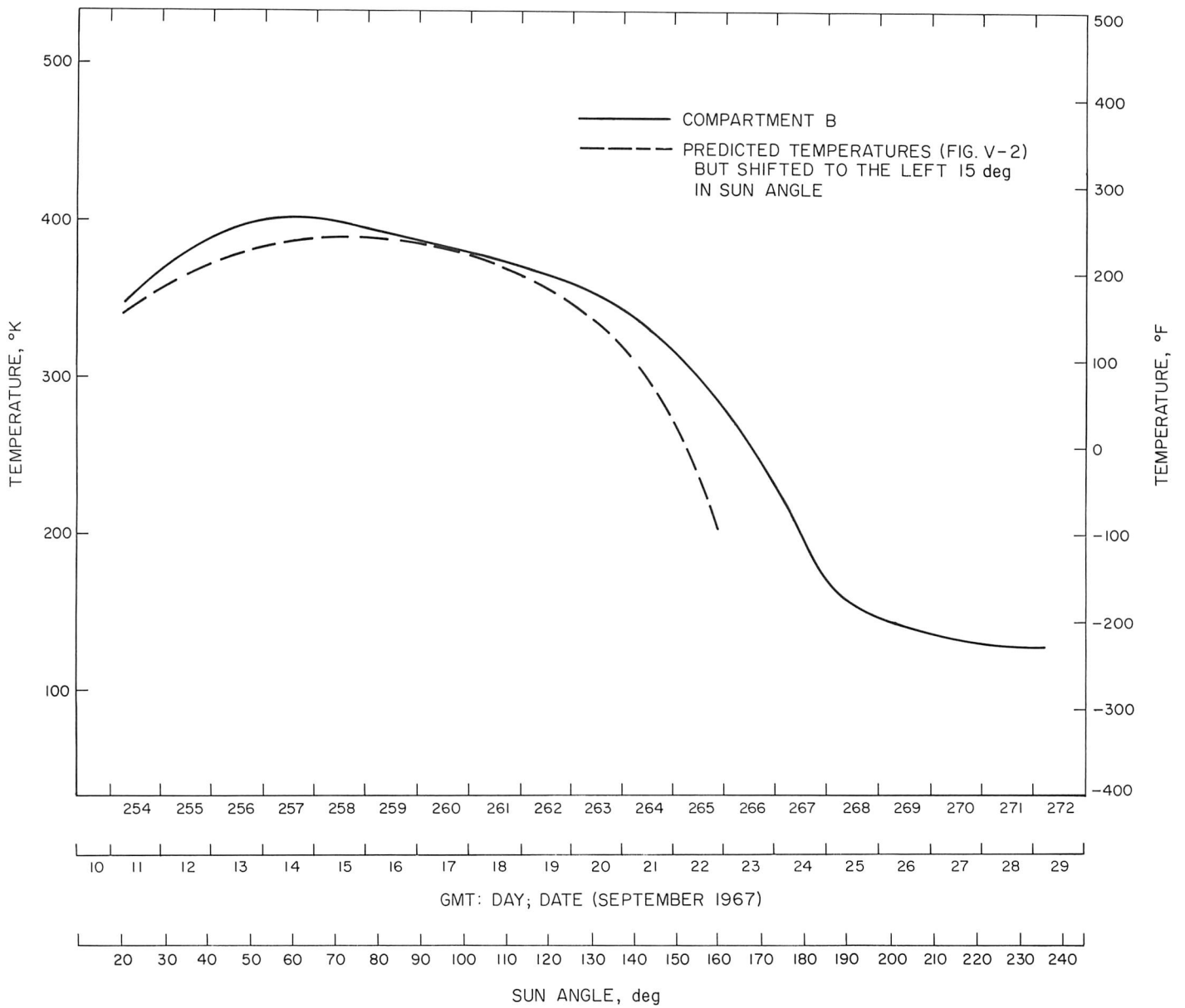
Fig. V-21. First-day brightness temperatures on lunar surface: compartment B data compared with predicted temperatures.
