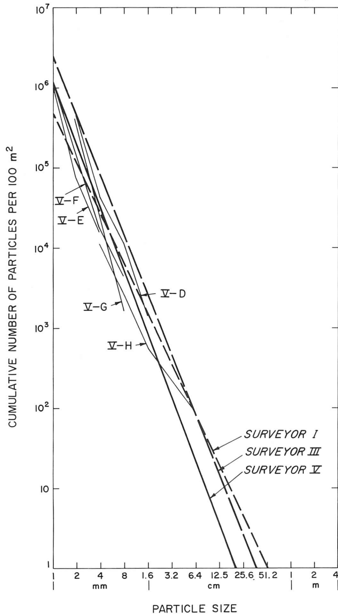
Fig. III-29. Size-frequency distribution of fragments on the undisturbed surface around Surveyor V (solid line) compared with the average size-frequency distribution of fragments at the Surveyor I and III landing sites (dashed lines).
