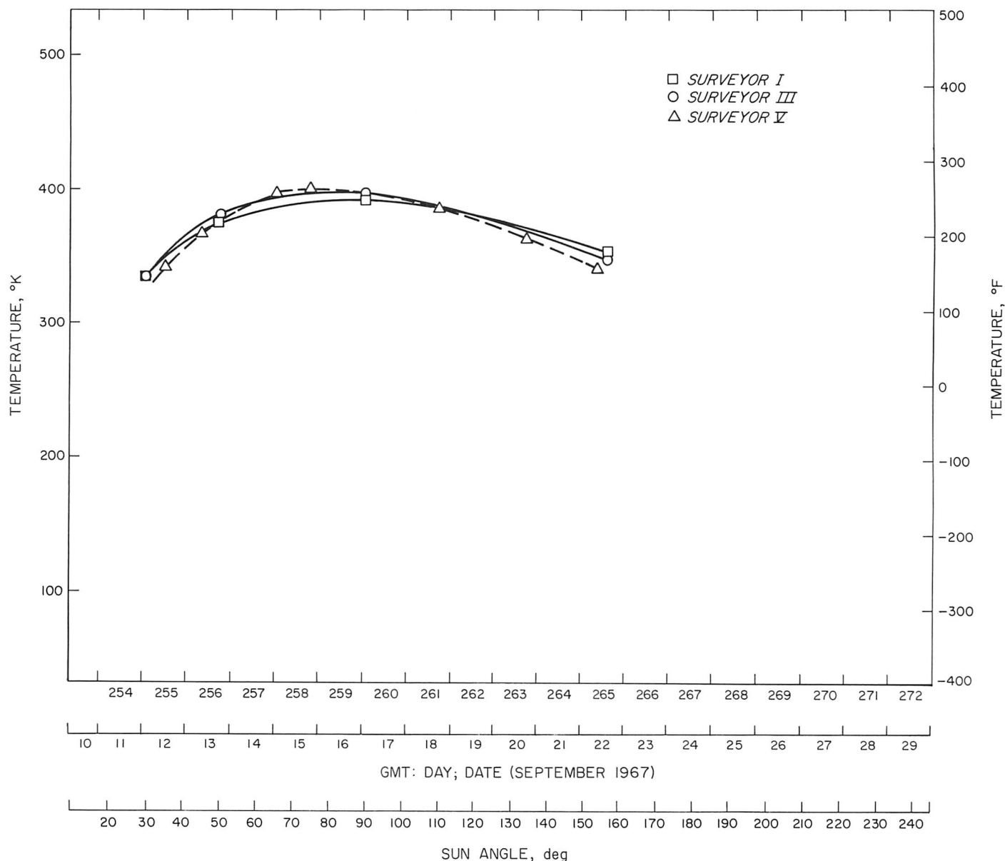
Fig. V-22. Lunar surface brightness temperatures from compartment B data on Surveyors I, III, and V (adjusted in time for Surveyor V ).
