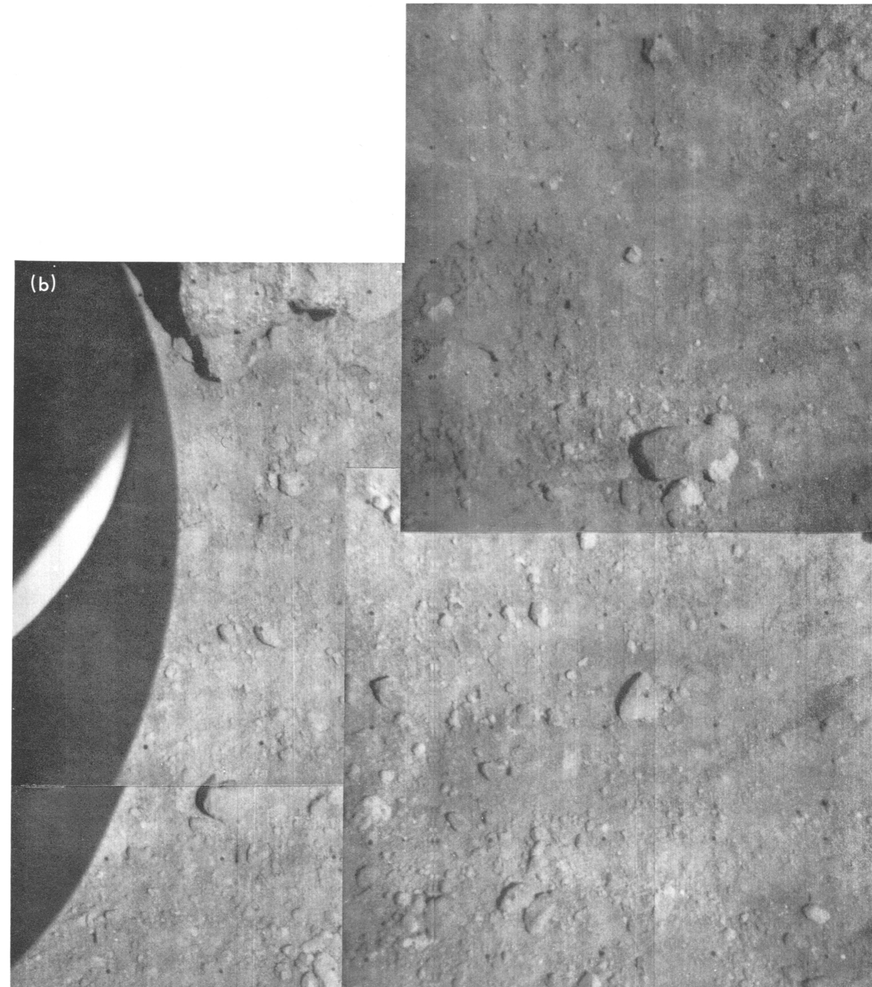
Fig. IV-29. Lunar surface beside the helium tank (see Figs. IV-27 and IV-28). Soil erosion from around rock "a" and the trail left by impact of fragment 26 were caused by the firing. (a) Pre-firing picture; Catalog 5-MP-43. (b) Post-firing picture; Catalog 5-MP-44.
