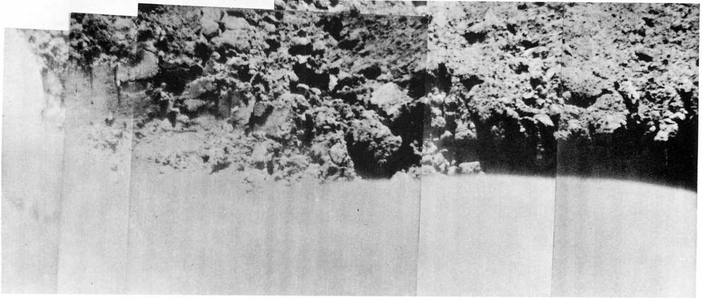
Fig. IV-37. Pre-firing mosaic of part of the trench dug by footpad 2 during landing (Day 256; Catalog 5-MP-36).
