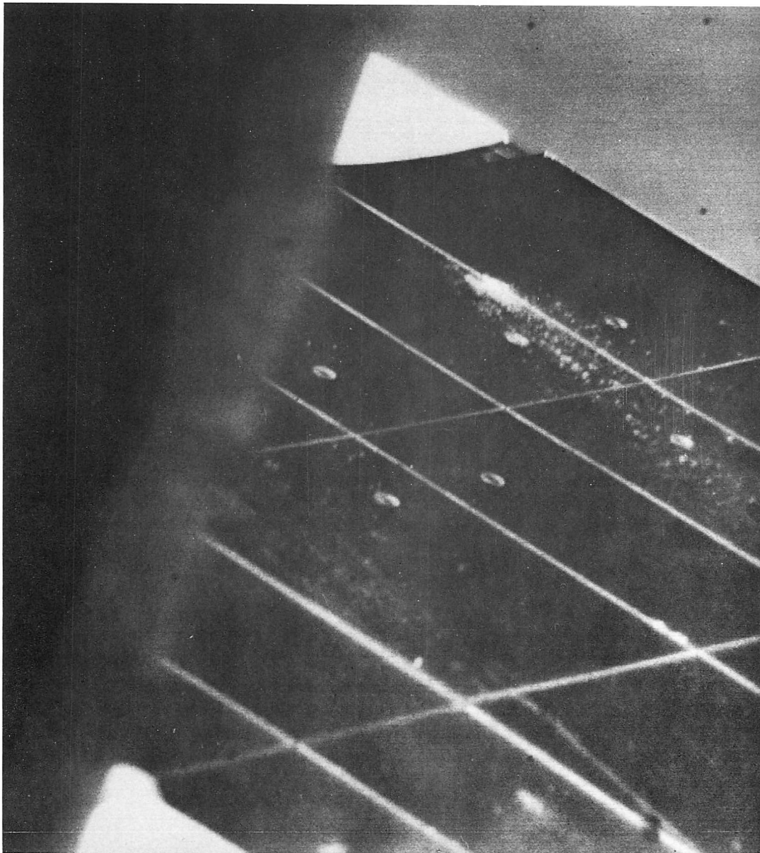
Fig. III-35. Narrow-angle picture of part of the top of compartment B of the Surveyor V spacecraft showing small clod of lunar surface material, dislodged by the exhaust from the vernier engines during an erosion experiment 53 hr after landing. This material has impacted the top of the compartment and broken into very fine grains (Day 258, 04:31:24 GMT).
