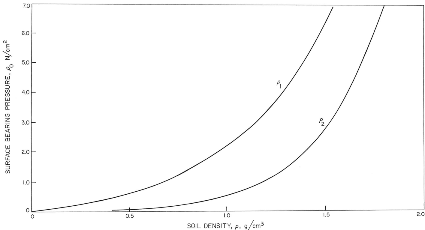
Fig. IV-18. Assumed relationship between surface bearing pressure and the soil density at the surface.
