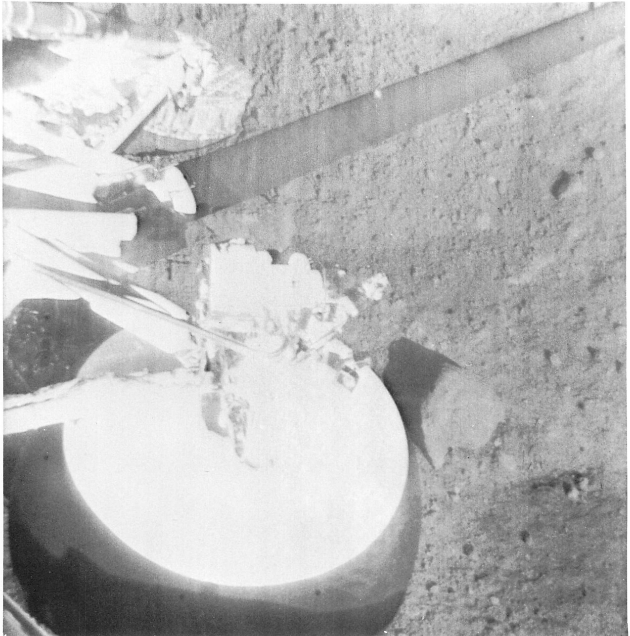
Fig. IV-12. Wide-angle picture of footpad 3. The footpad imprint in the lunar material can be seen above the antenna boom. The footpad remained tilted after the landing phase. Ghost image of the helium tanks was caused by incomplete erasure of previous image on vidicon (Day 254, 23:50:28 GMT).
