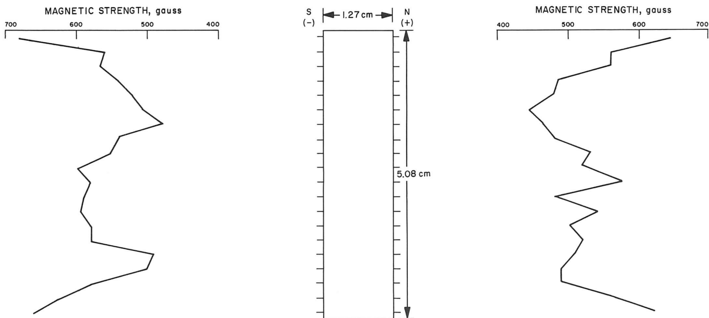
Fig. VIII-3. Plot of pole-strength dropoff along the pole faces of the magnet on Surveyor V.
