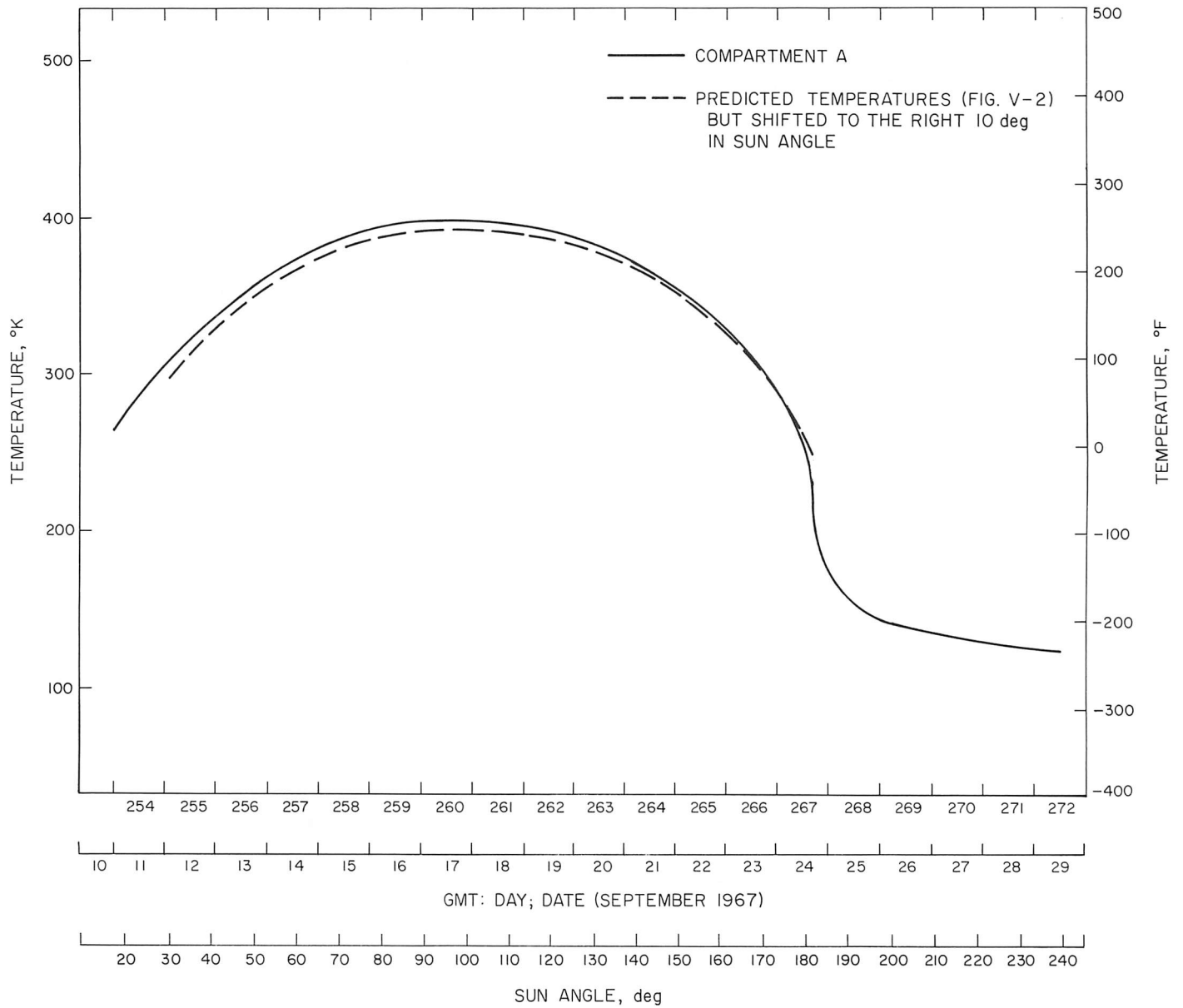
Fig. V-20. Lunar surface brightness temperatures during first lunar day: compartment A data compared with predicted temperatures.
