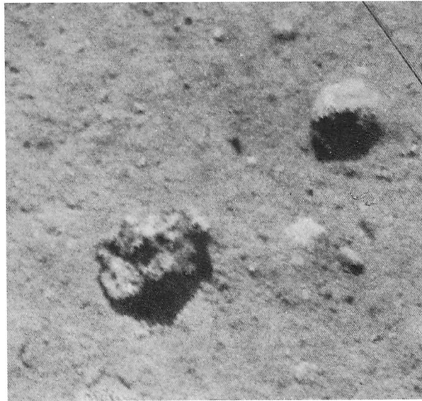
Fig. III-25. Small, irregular fragment, about 3 cm across, close to spacecraft. Various parts of fragment are either much brighter or much darker than surrounding fine-grained debris, which suggests that this fragment is partly glassy. It resembles impactites from Meteor Crater, Arizona, and shock-melted ejecta from nuclear craters (see Fig. III-27; Day 258, 08:30:15 GMT).
