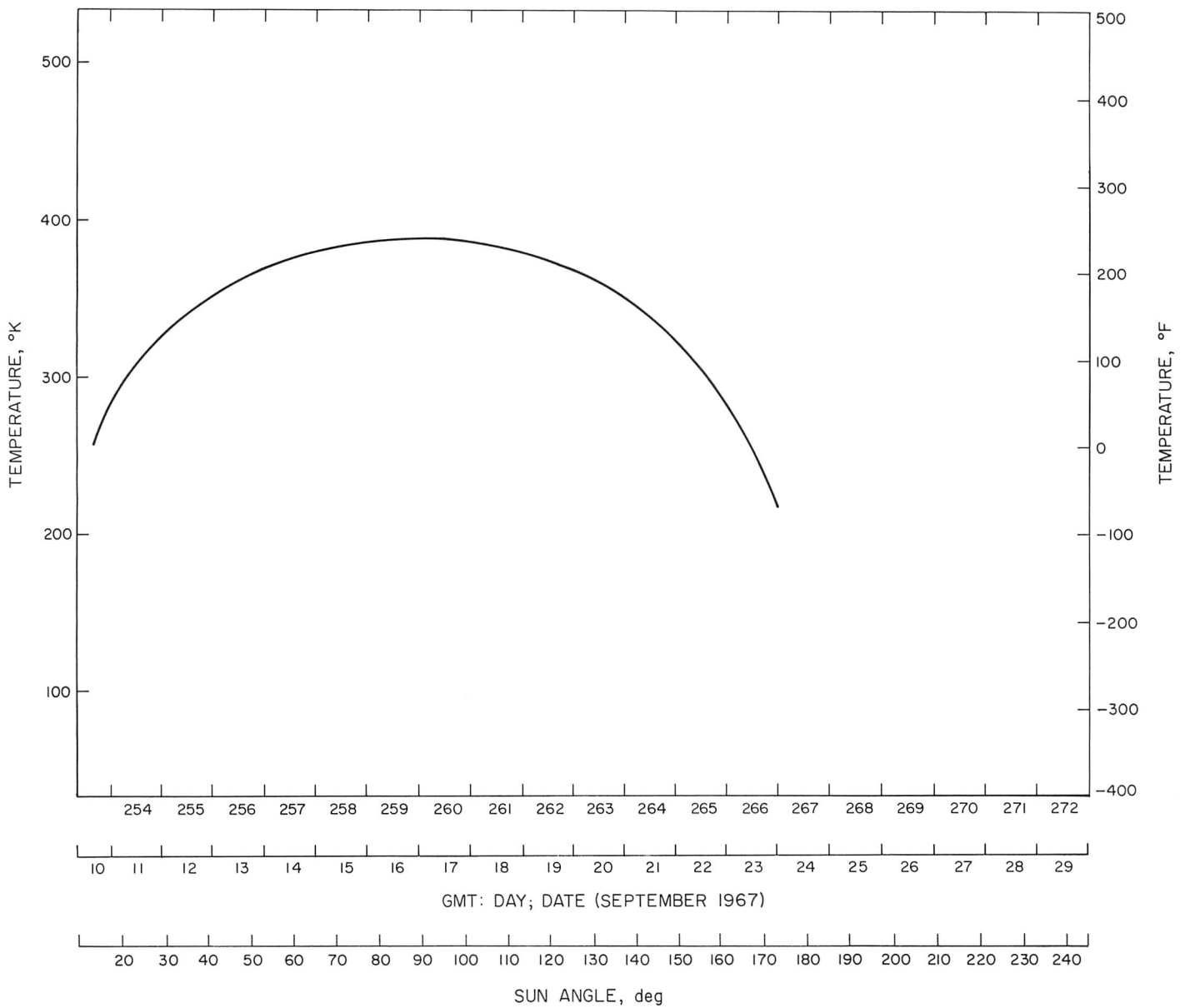
Fig. V-2. Earth-based lambertian temperatures for Surveyor V landing site, assuming level lunar surface.
