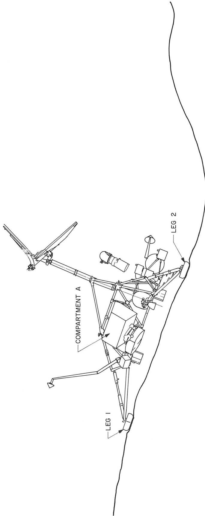
Fig. V-6. Profile of crater in which Surveyor V landed.
