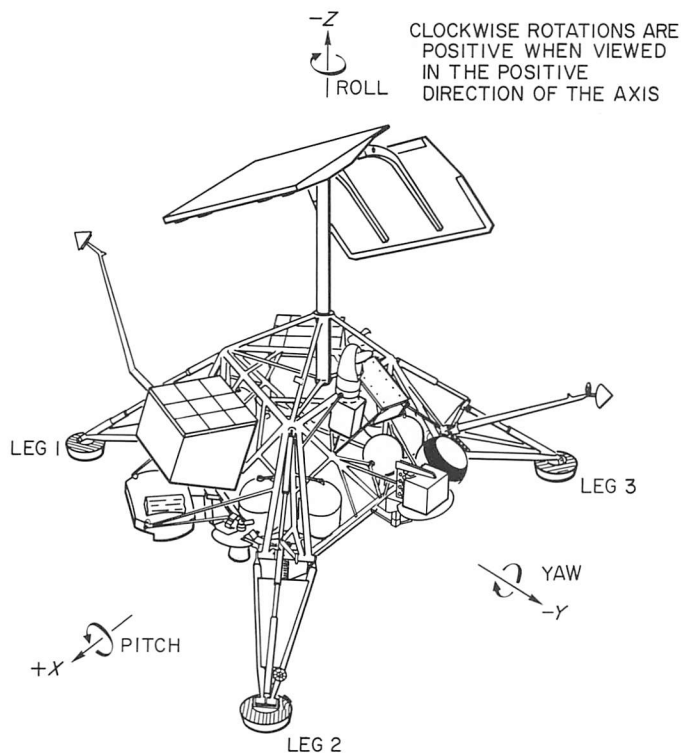
Fig. IV-1. Surveyor spacecraft configuration and coordinate system.
