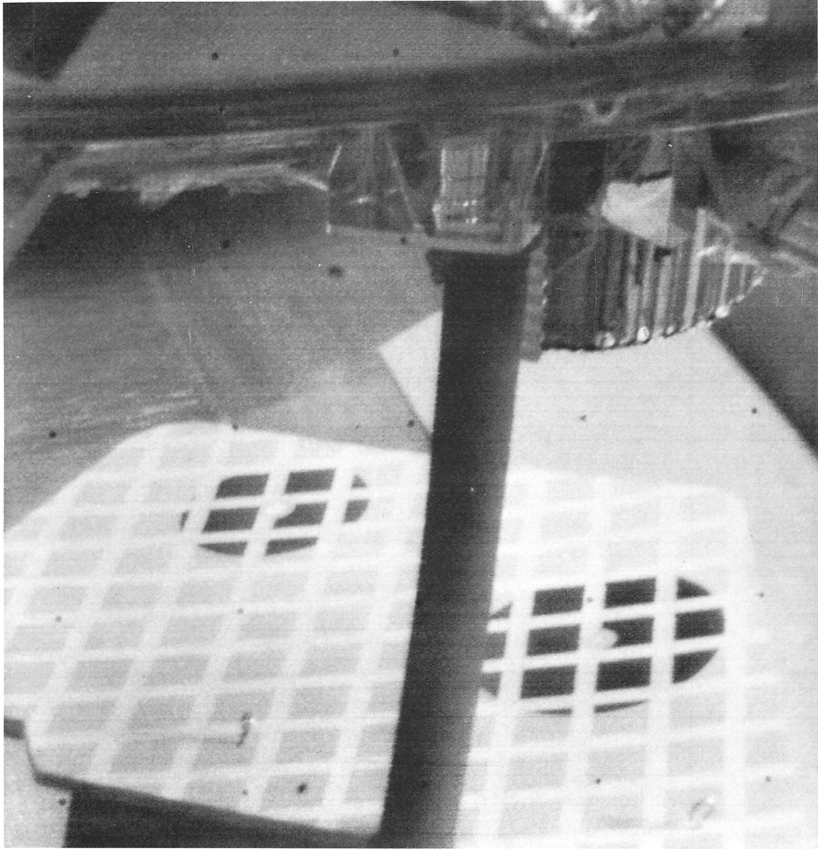
Fig. IV-40. Narrow-angle picture taken by the Surveyor V television camera system prior to launch.
