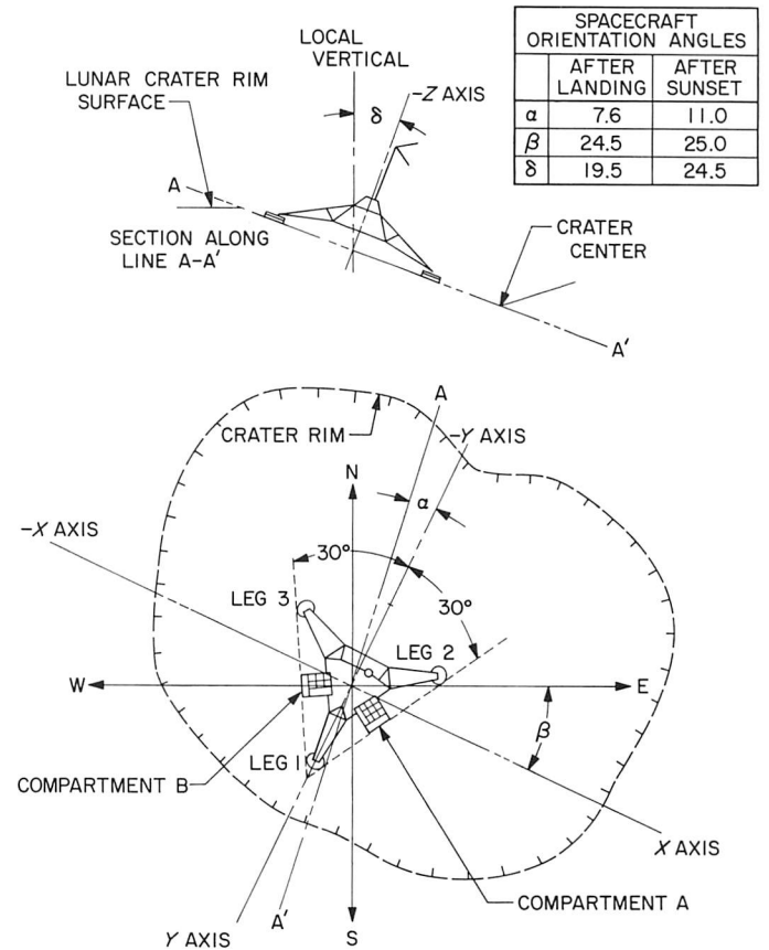
Fig. V-5. Surveyor V landed orientation.
