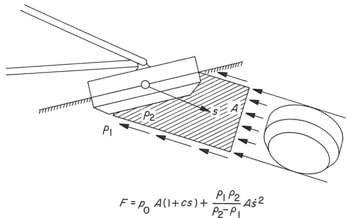
Fig. IV-17. Soft surface model for the landing dynamics analysis.
