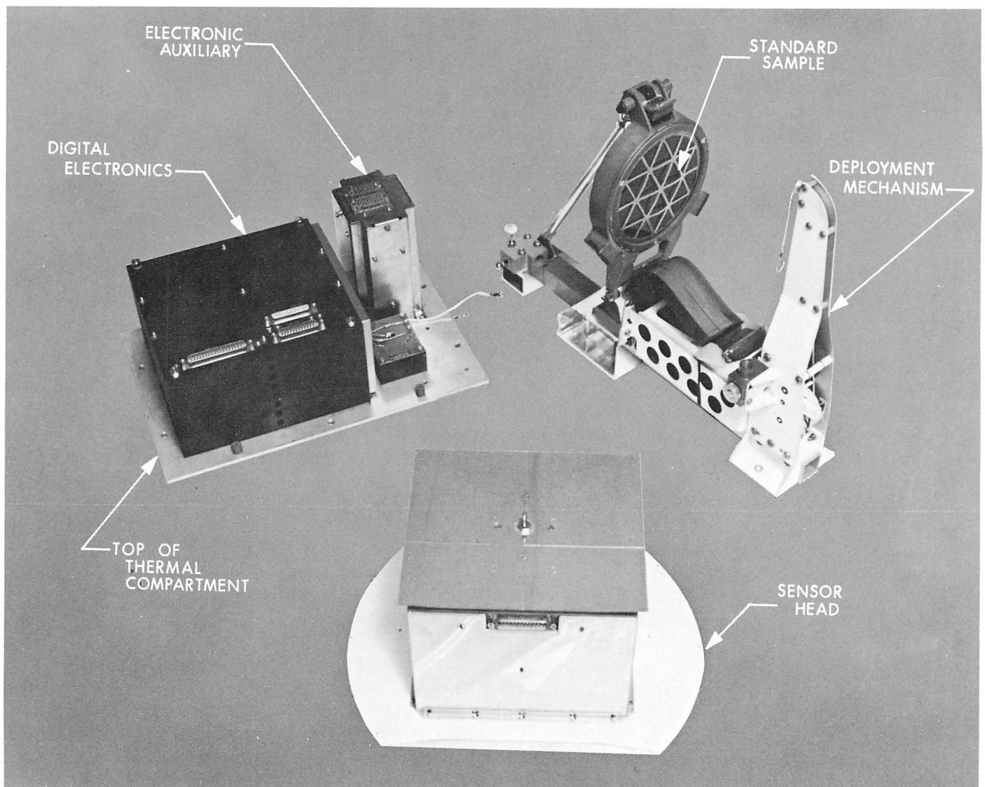
Fig. VII-1. Alpha-scattering instrument and auxiliary hardware.
