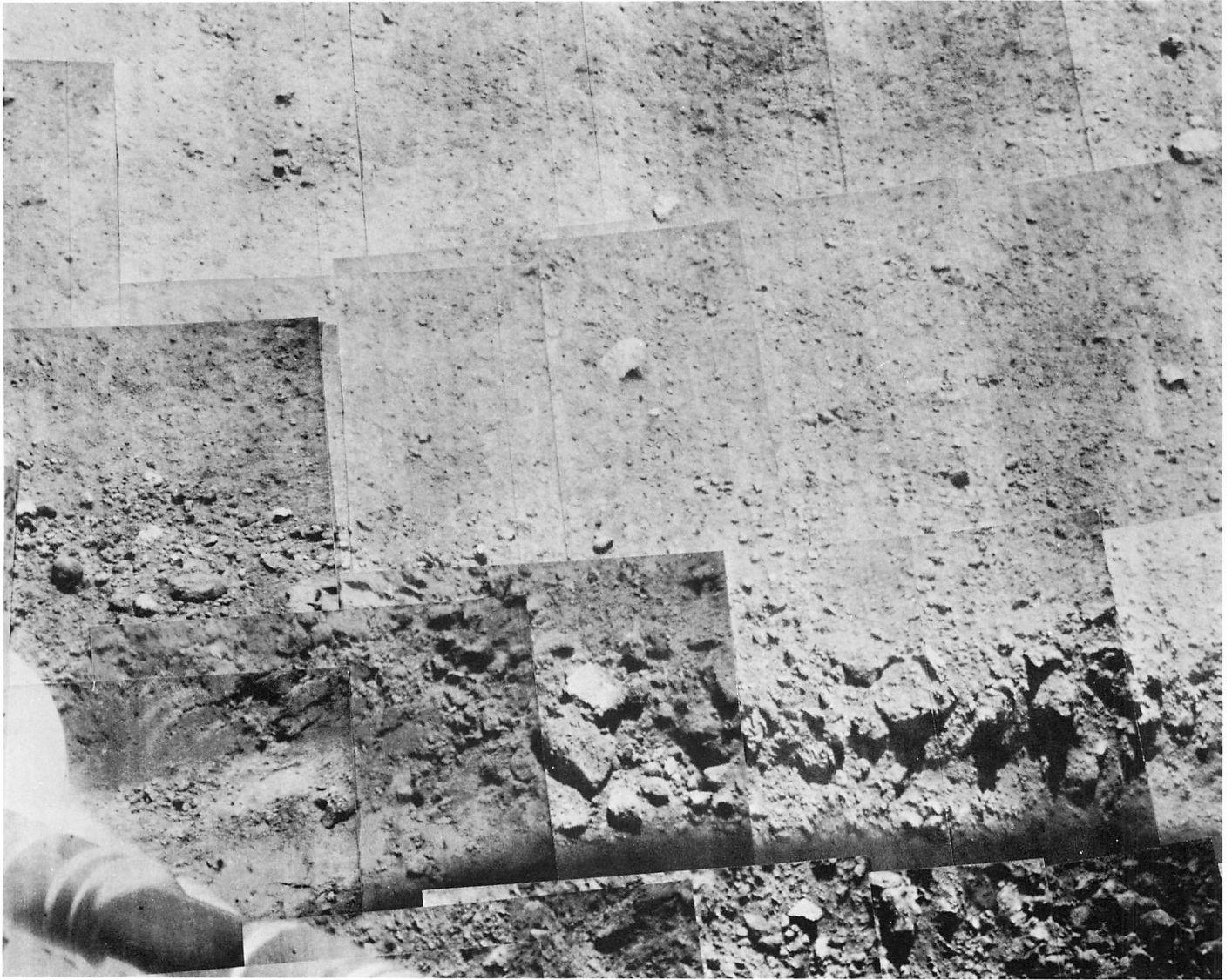
Fig. IV-38. Post-firing mosaic of the same portion of footpad 2 trench seen in the pre-firing mosaic (Fig. IV-37). No disturbance was caused by the firing of vernier engine 2, which was approximately 1 m away (Day 258).
