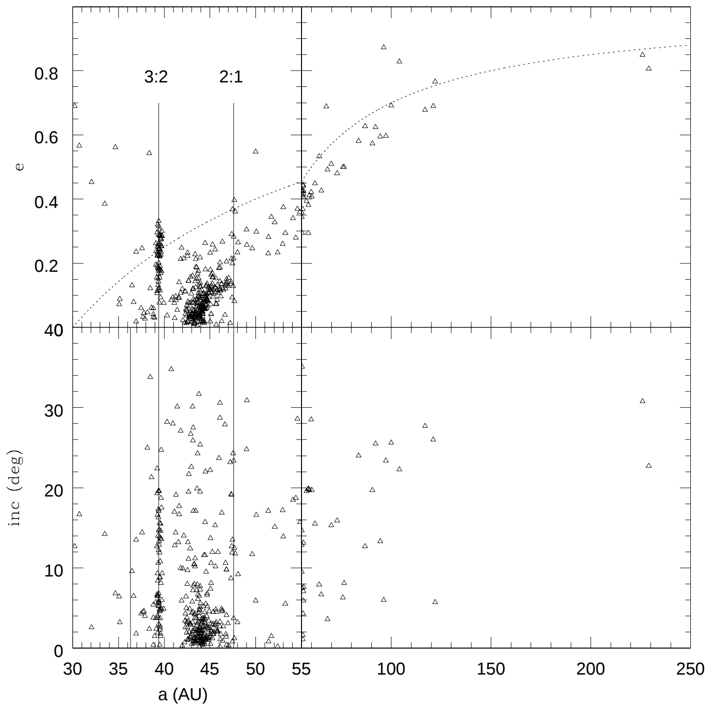
Kuiper Belt Objects: orbital distribution
