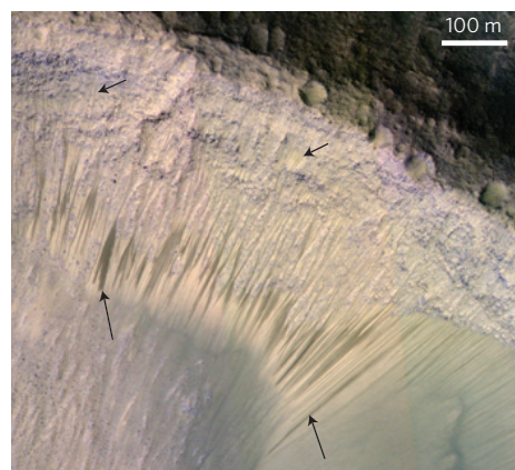
Figure 3 | RSL on the south-facing slope of a crater on the floor of Melas Chasma. IRB colour with minimum–maximum stretch as in Fig. 2, but north is up. Black arrows point to some of the many individual lineae. The RSL begin in narrow channels on the steep, rocky crater slope and spread out on the smooth fans. They were active on this portion of crater wall in early southern spring and summer (Table 1 and Supplementary Table 1). See http://www.uahirise.org/sim/ for a set of animated GIF files illustrating the activity. Portion of image ESP_031059_1685.
