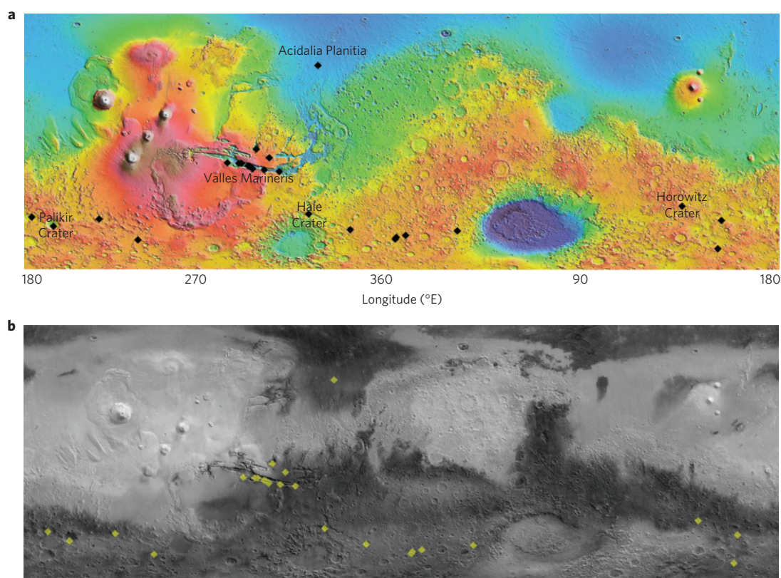
Figure 1 | Locations of confirmed recurring slope lineae (RSL). a , Confirmed RSL sites (black diamonds) on MOLA (ref. 9) colour-coded altimetry (latitude 60° S–60° N). MOLA elevation colours range from blue (low elevations) to red and white (high elevations). b , The same set of RSL (yellow diamonds) on a global bolometric albedo map from the Thermal Emission Spectrometer 40 . Both maps show MOLA shaded relief and are in simple cylindrical projection. All RSL sites plotted here are in areas with Thermal Emission Spectrometer albedo < 0.2.
